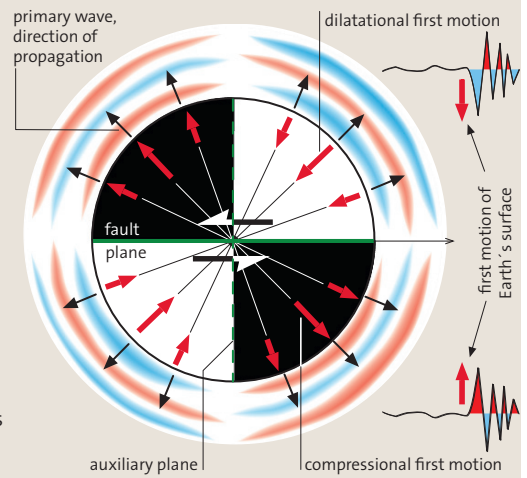
► Fig. 2.14 Principle of fault-plane-solutions of an earthquake hypocenter. The fault plane of the earthquake (orthogonal to the paper plane) and an orthogonal virtual aiding plane define four quadrants. First motions of the primary waves oscillating in the propagation direction and expressed by vertical motions in the soil indicate the sense of movement of the blocks displaced during the earthquake. Seismograms subdivide two quadrants with compressive and two quadrants with dilatative first motion.
