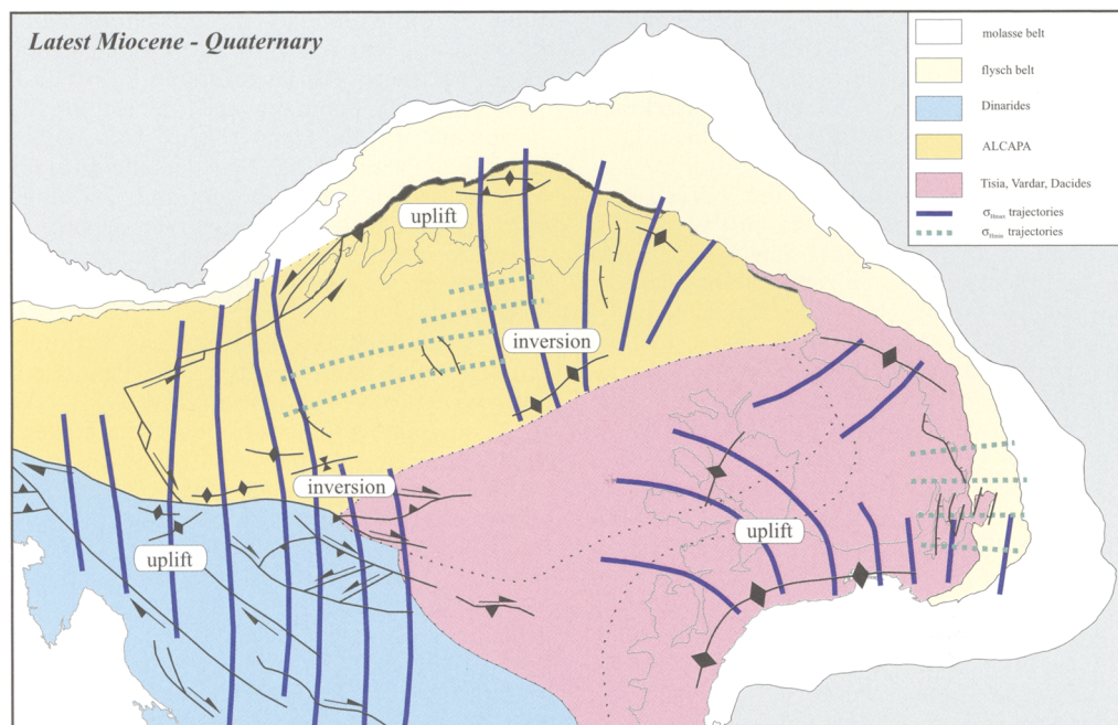
Fig. 6. Evolution of major blocks of the Pannonian area: tentative model for the connection of stress field and deformation. Compare with Figs 4 and 5. Kinematic reconstruction of major blocks is partly after Balla (1984); Csontos (1995); Kováč et al. (1994), Ratschbacher et al. (1991a). Numbers along the thrust front indicate the age of the last thrust in Ma, after Jiříček (1979).
