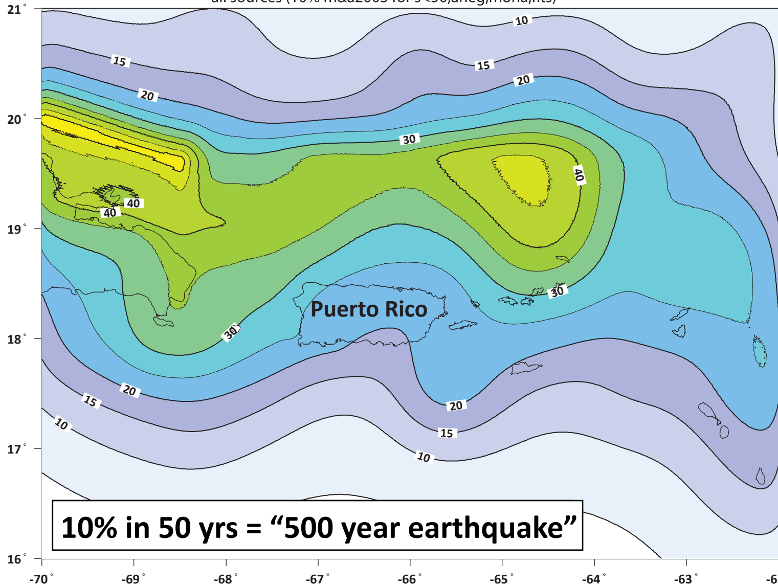
PGA with 10% Probability of Exceedance in 50 Years (%g) all sources (10% m&a2003 for s<50,aneg,mona,flts)
