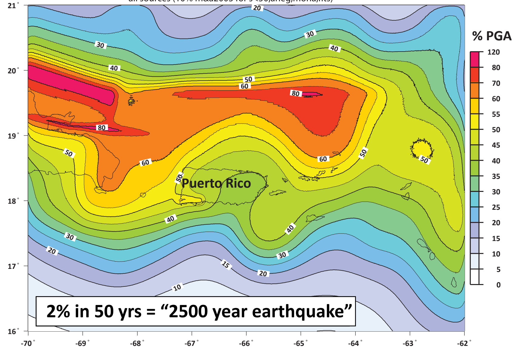
PGA with 2% Probability of Exceedance in 50 Years (%g) all sources (10% m&a2003 for s<50,aneg,mona,flts)
