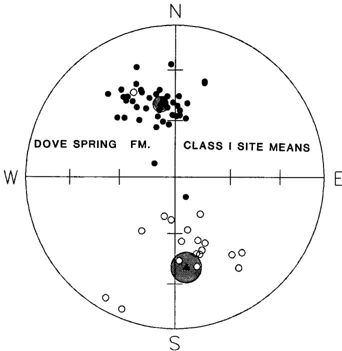
Figure 6. Stereonet plot of demagnetized class I normal and reversed sites. The data are nearly antipodal and indicate that a mean of 15^\circ of counterclockwise rotation has occurred. The stippled areas indicate the \alpha_{95} -error envelope on the mean directions.
