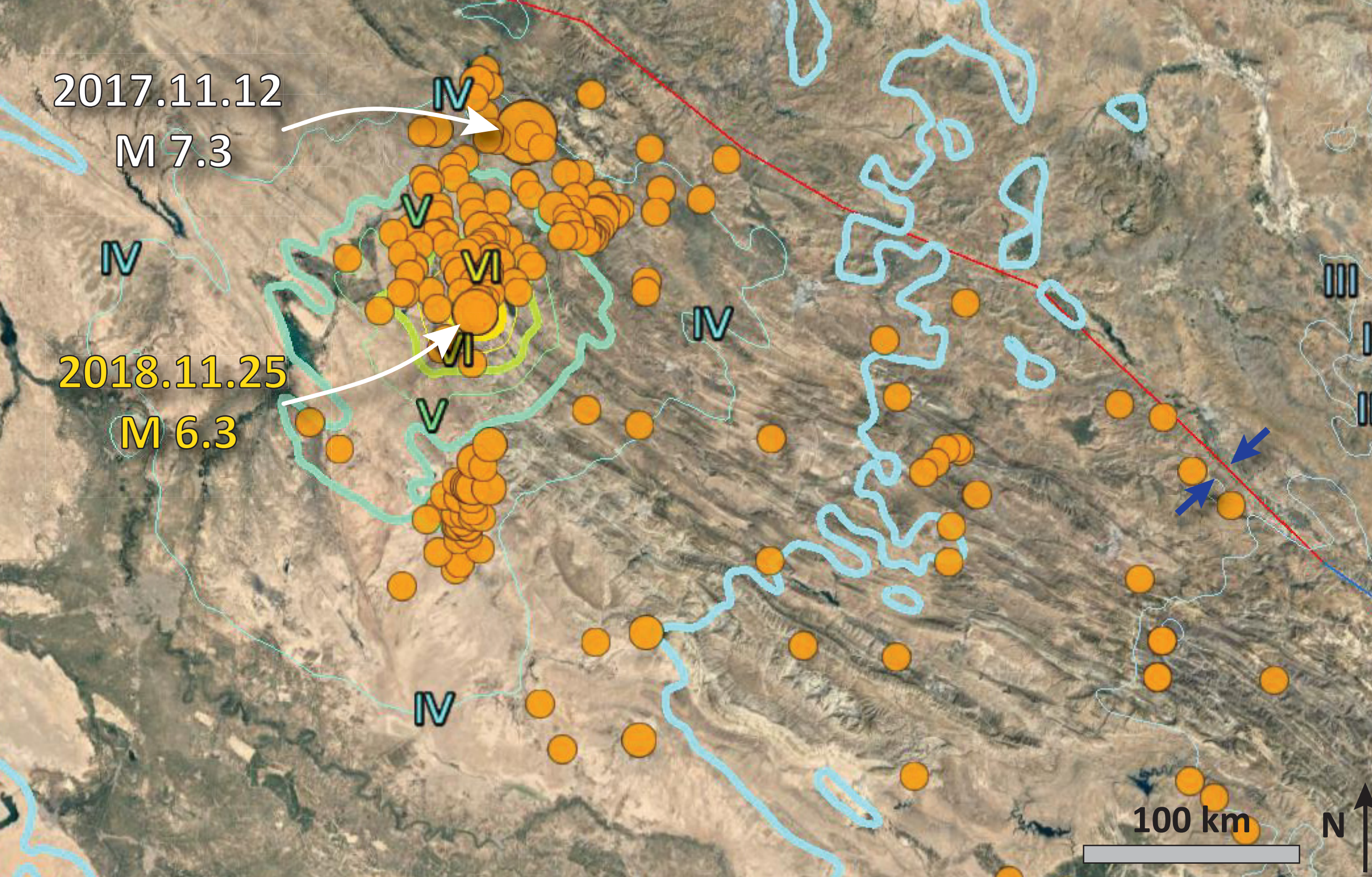
Aftershocks and Triggered Earthquakes from 2017.11.12 M 7.3
