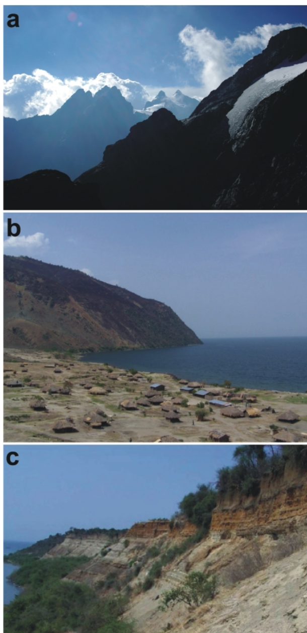
FIGURE 2: (a) Mountainous topography in the Rwenzori Mountains of west Uganda south of Lake Albert. The Rwenzori Mountains are a promontory of the Albertine Rift shoulder and rise to 5109 m.a.s.l. (photo courtesy Daniel Koehn). (b) Rift shoulder of Lake Albert in the Albertine Rift of west Uganda, Western Branch of East African Rift System. Unlike other rift lakes of the Western Branch, Lake Albert is not deep and has a maximum depth of 51 m, and a surface elevation of 619 m.a.s.l. (photo courtesy Friederike Bauer). (c) Late Miocene to Quaternary lacustrine and fluvial sediments are common in the East African Rift System (photo courtesy Friederike Bauer).
