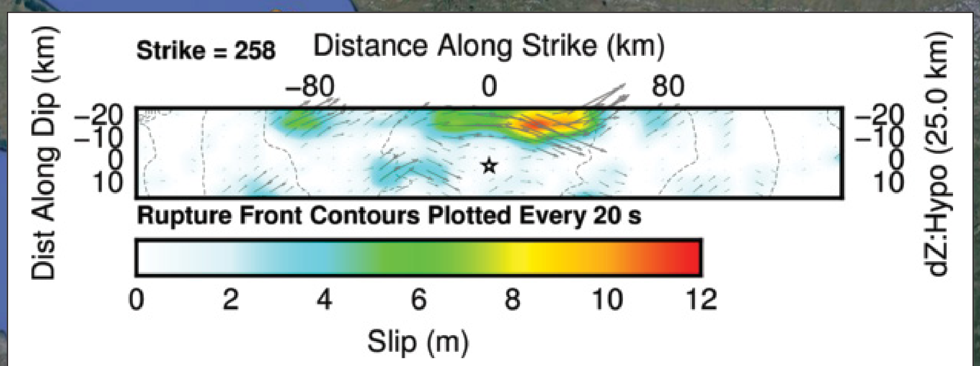
USGS Slip Model
