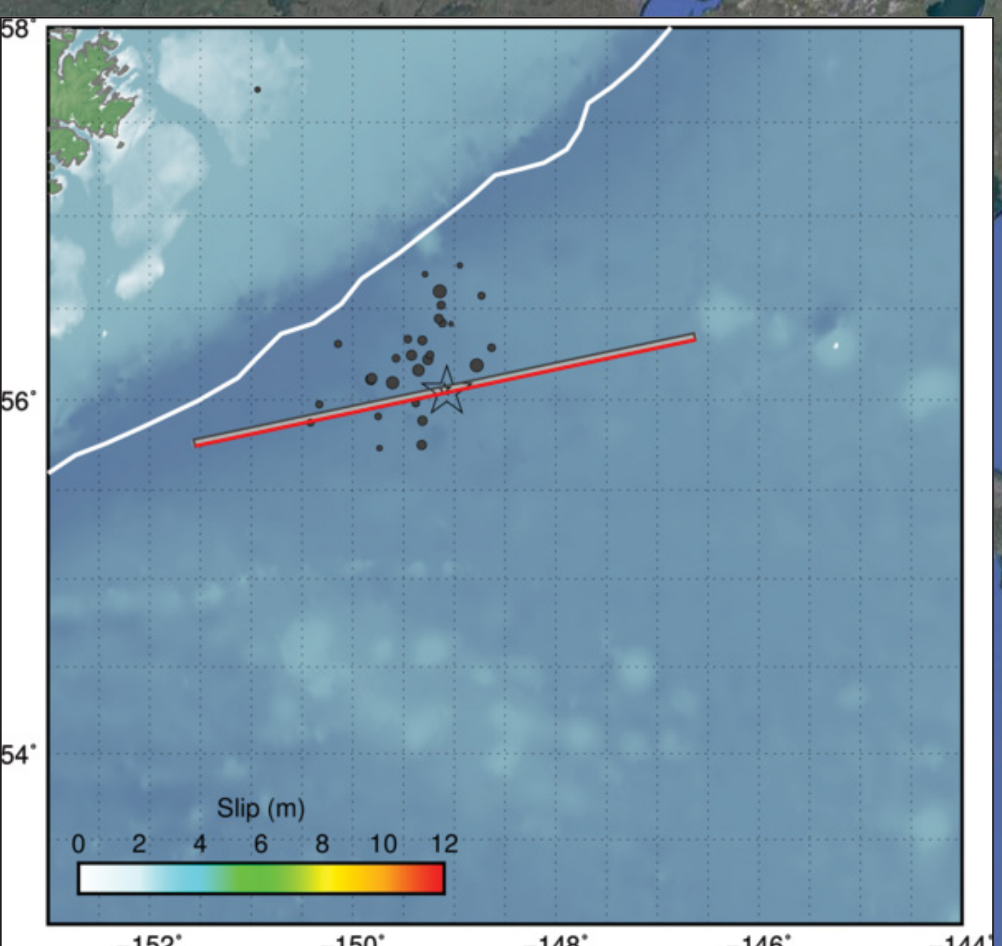
USGS Fault Model
