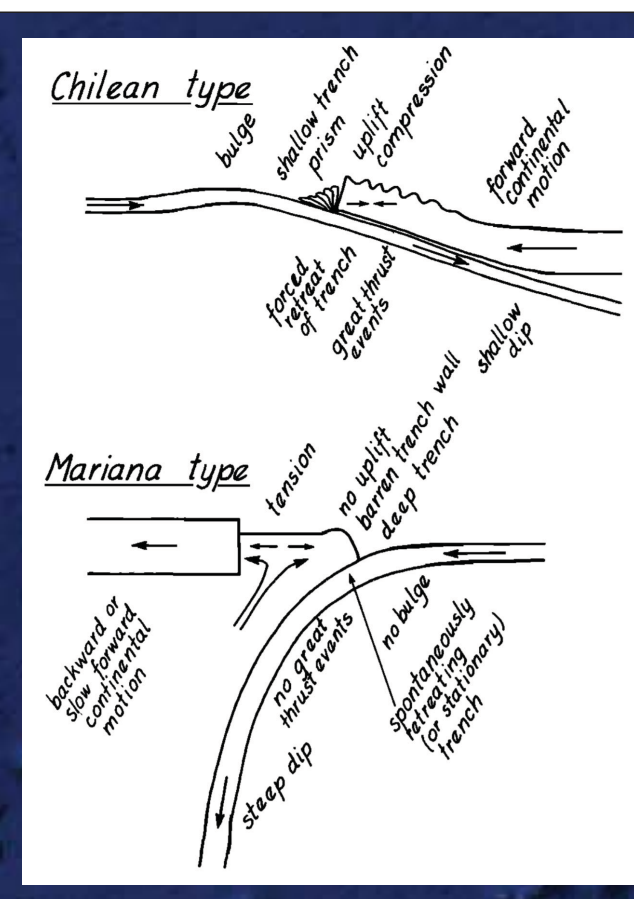
Uyeda & Kanamori, 1979
