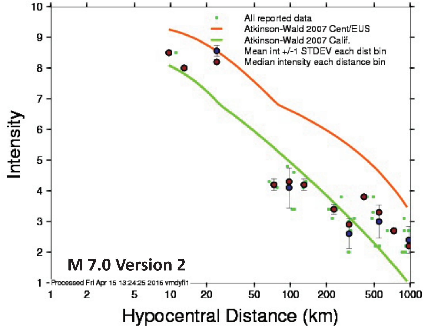
Intensity vs. Distance Plot (ID us20005iis)
