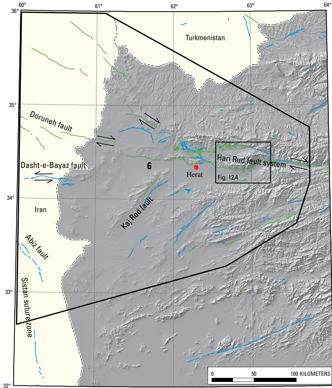
Figure 12. Tectonic domain 6—the Western Hari Rud fault system outlined in black. In this domain, the right-lateral motion on the eastern and central parts of the Hari Rud fault system transitions into a structural style that is more typical of the Basin-and-Range province of the western U.S. East of Herat, the narrow valley of the Hari Rud or Herat River widens at a left-step in the right-lateral fault system. West of this left-step, the valley is bounded by mountains that have steep range fronts and broad alluvial piedmonts. Arrows show directions of movement on lateral-slip faults. Fault categories are category B, green; and category C, blue.
