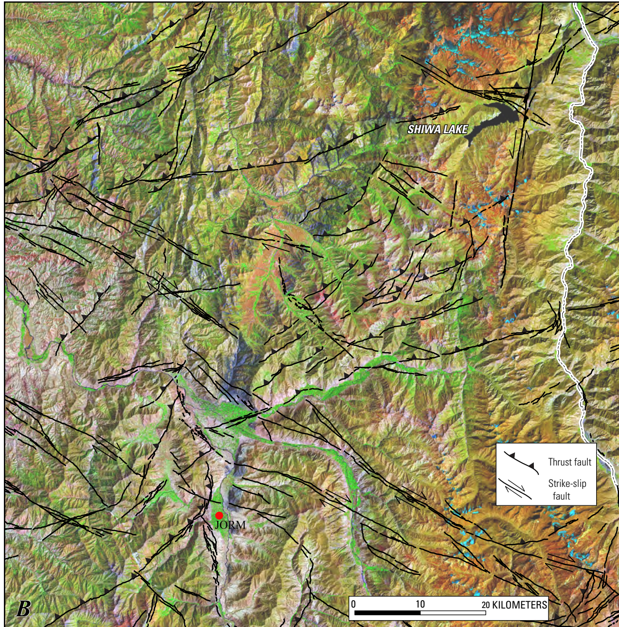
Figure 8B. Map of features associated with active tectonics, central Badakhshan. The Quaternary deformation in this region appears to be partitioned between southeast-directed thrust faults and northwest-trending right-lateral strike-slip faults. The faults are predominantly classified as category C faults (pl. 1, no. 23 and 25). Image is a panchromatically enhanced Landsat image that merges bands 7+4+1. See figure 8 for location.
