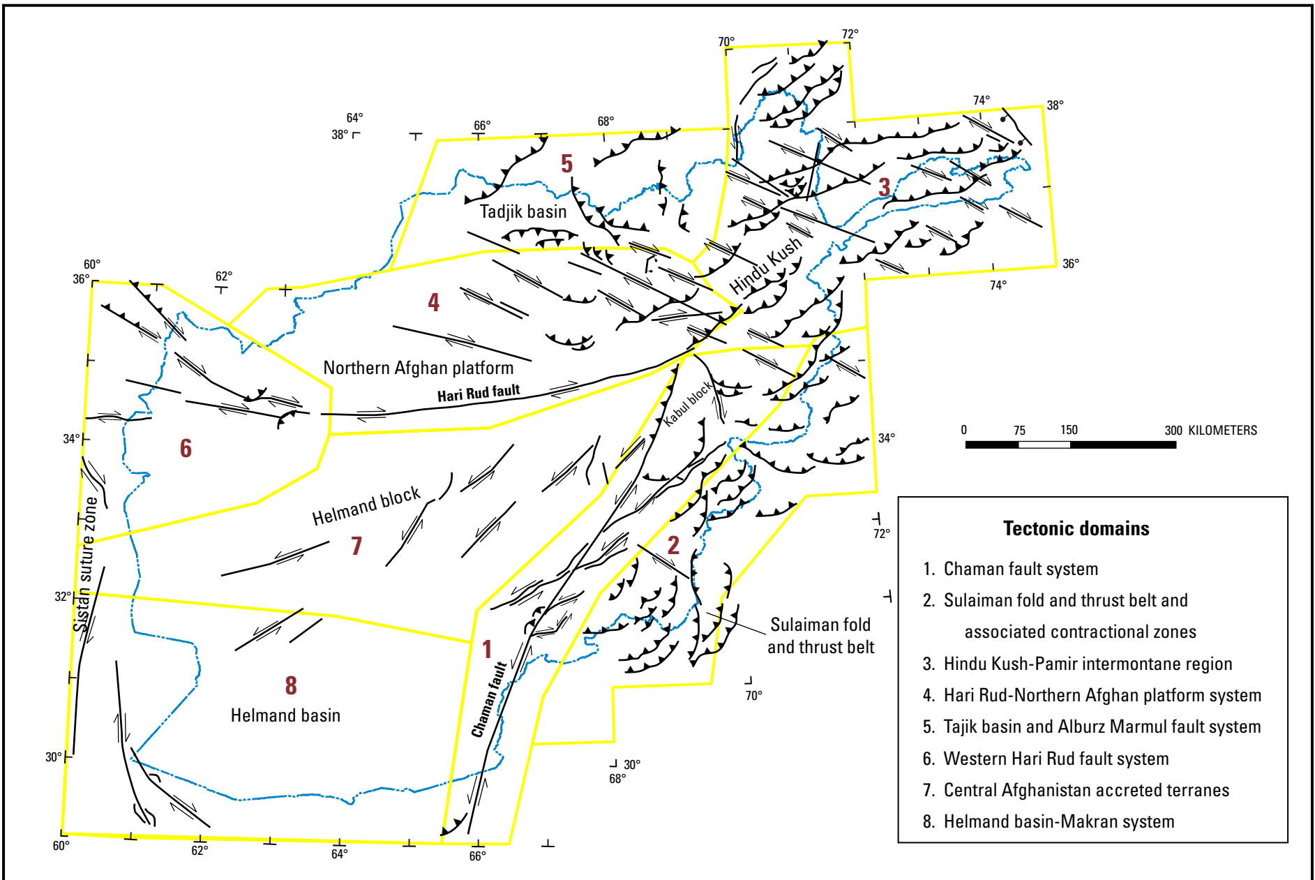
Figure 15. Schematic map of probable and possible Quaternary faults in Afghanistan showing kinematic relations and nationwide patterns of deformation. Each domain is numbered as discussed in text and boundaries are shown in yellow. Solid lines with arrows denote strike-slip faults, arrows show directions of movement. Solid line with teeth denote thrust faults, teeth on upthrown block. Ball-and-bar symbol denotes normal faults with symbol on downthrown block.
