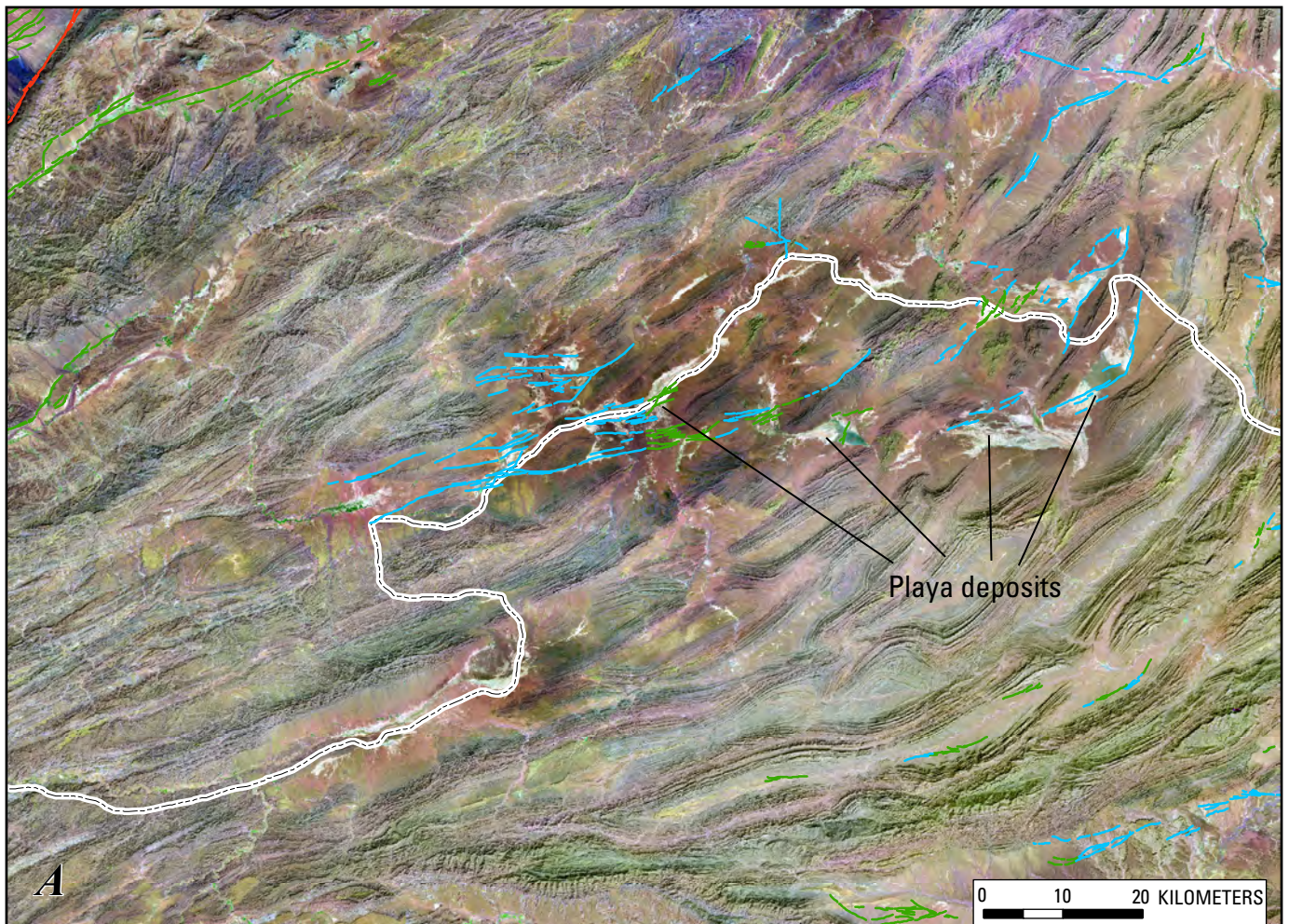
Figure 7A. Landsat image of the Sulaiman fold-and-thrust belt (pl. 1, no. 90) composed of intensely folded Eocene and Oligocene rocks in the Katawaz basin. Dissected and uplifted playa deposits indicate that active thrust faulting is advancing southeastward and uplifting and faulting older basin-fill deposits. Fault categories are category A, red; category B, green; and category C, blue. Image is a panchromatically enhanced Landsat image that merges bands 7+4+1. White dashed line is border between Afghanistan and Pakistan. See figure 7 for location.
