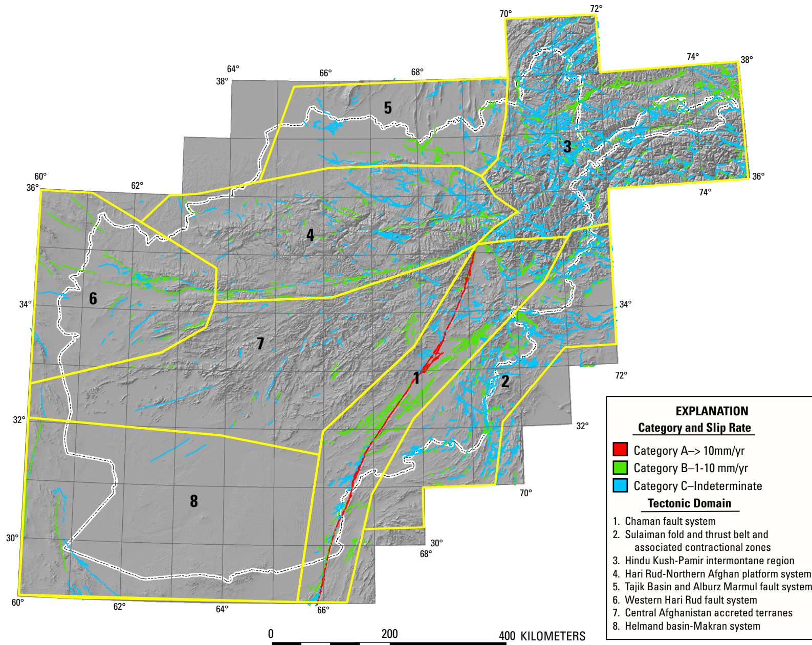
Figure 5. Probable and possible Quaternary faults and eight tectonic domains (shown by yellow boundaries) of Afghanistan. Domains are defined by regions having a similar structural style of deformation and, as a result, a similar physiographic expression. See the text for discussions of each domain.
