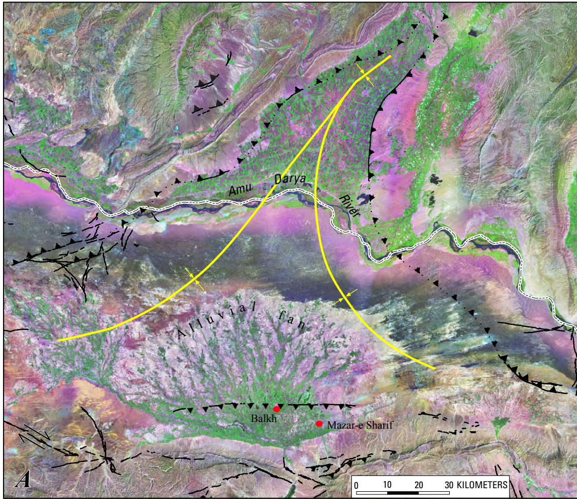
Figure 11.4. Probable and possible active features in the area around Mazar-e Sharif, north-central Afghanistan. The large alluvial fan is filling a basin that is located in front of active folds to the south. Yellow lines and arrows show the approximate axis of the syntaxial basin. Features inferred to be thrust faults are shown with teeth on the upthrown side; faults are dotted where concealed. Amu Darya River and white dashed line are the northern border of Afghanistan. Image is a panchromatically enhanced Landsat image that merges bands 7+4+1. See figure 11 for location.
