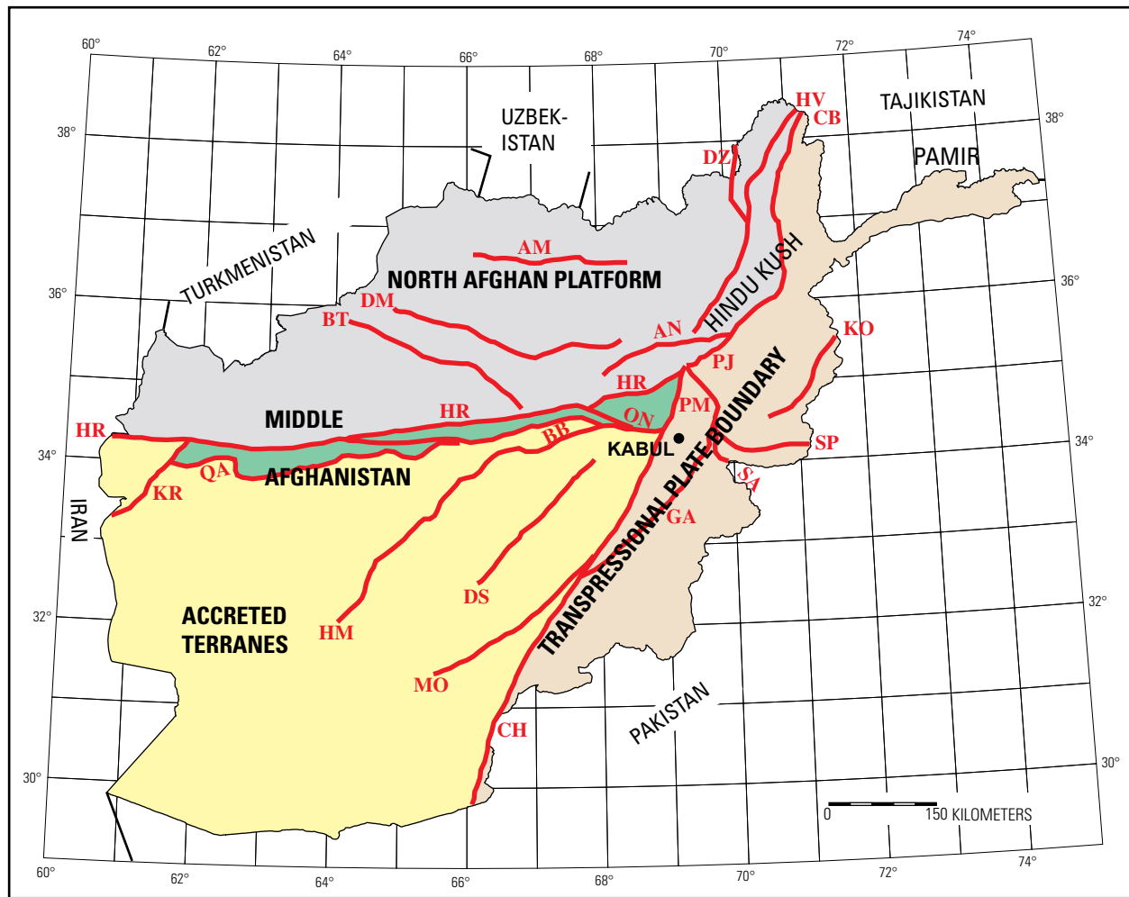
Figure 3. Seismotectonic provinces and major fault zones (bold red lines). Abbreviations of fault names: AM, Alburz Marmul; AN, Andarab; BB, Bande Bayan; BT, Bande Turkestan; CH, Chaman; CB, Central Badakhshan; DS, Dorafshan; DZ, Darvaz; DM, Dosi Mirzavalan; GA, Gardez; HR, Hari Rud; HM, Helmand; HV, Henjvan; KR, Kaj Rod; KO, Konar; MO, Mokur; ON, Onay; PM, Paghman; PJ, Panjshir; QA, Qarghanaw; SA, Sarobi; SP, Spinghar. Modified from Wheeler and others (2005).
