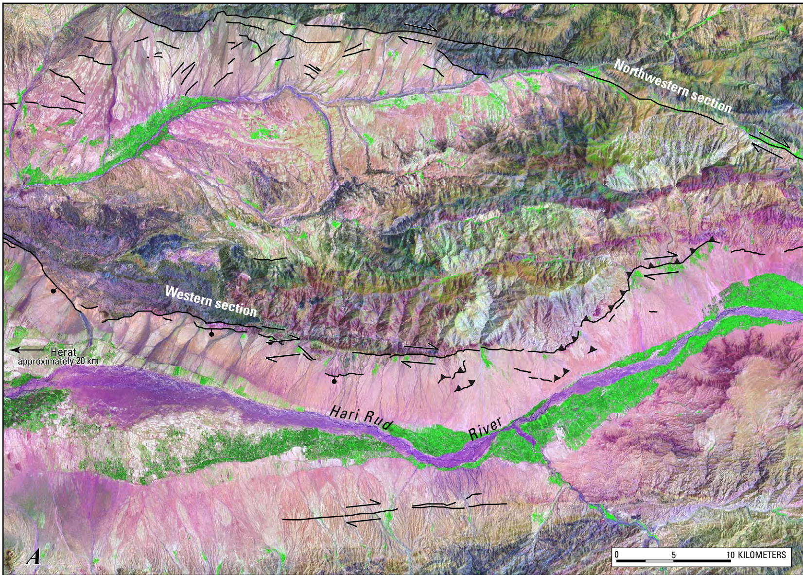
Figure 12.4. Map of features along the western part of the Hari Rud fault system. To the east of this view, the fault system separates into a northwestern section that extends through the bedrock range and into basins north of Herat, and a western section that continues along the northern margin of the Hari Rud River Valley. Inferred thrust faulting occurs at a left step (to the southwest) in the right-lateral, strike-slip fault system. Black lines are faults, with teeth on the upthrown side of thrust faults; arrows indicate directions of movement on strike-slip faults; bar-and-ball is on downthrown side of normal faults. Image is a panchromatically enhanced Landsat image that merges bands 7+4+1. See figure 11 for location.
