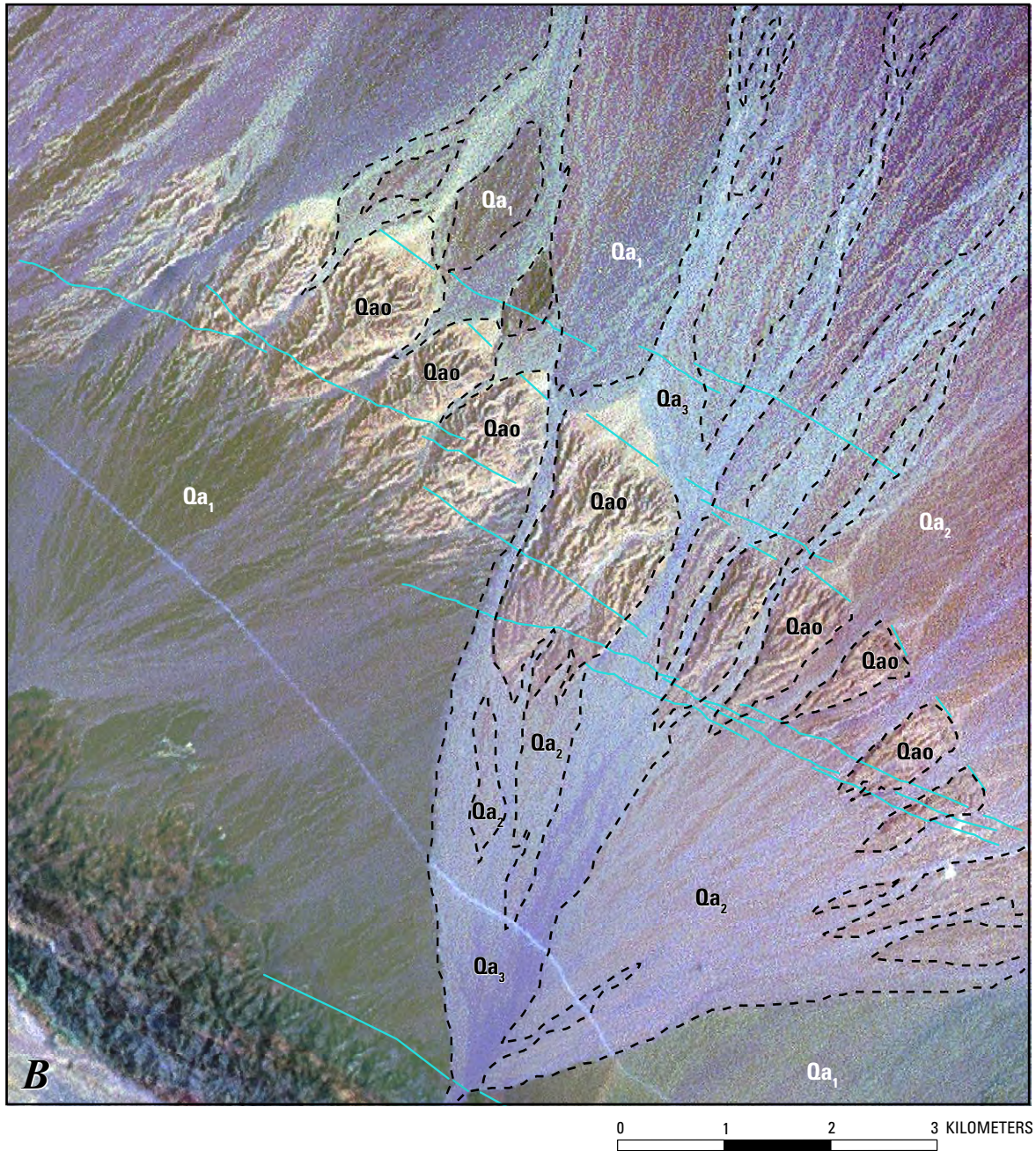
Figure 14B. Surface expression of category C faults shown by blue lines (pl. 1, no. 130 and 132) in the Helmand basin in northwestern Pakistan across the border from southwestern Afghanistan. Surface expression of the fault traces is generally discontinuous. The fault has uplifted an old alluvial fan (Qao) or bedrock(?), and younger alluvium (Qa 1 , Qa 2 , and Qa 3 ) has eroded and buried parts of the fault. These relations indicate that there are relatively long time intervals between surface-rupturing earthquakes on this fault. Drainages that cross the fault do not appear to be laterally offset, which indicates that displacement is primarily vertical, probably on thrust faults. Image is a panchromatically enhanced Landsat image that was created by merging bands 7+4+1. See figure 14 for location.
