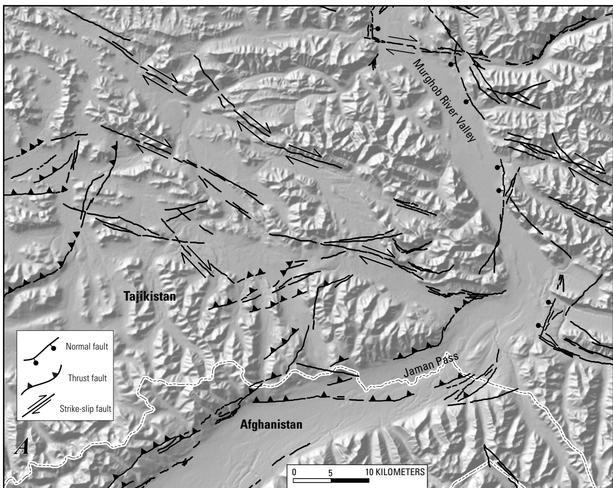
Figure 8A. Map of features associated with active tectonics in northeastern Afghanistan and the Jaman Pass-Murghob River region of Tajikistan (pl. 1, no. 1 and 3). Features thought to have strike-slip movement have arrows showing directions of movement. Thrust faults have teeth on upthrown side. Normal faults in the Murghob River Valley have a bar and ball on the downthrown side. These features are predominantly category B structures and have inferred slip rates of 1–10 mm/yr. Base map is from SRTM (Shuttle Radar Topographic Mission) data. White dashed line is boundary between Afghanistan and Tajikistan. See figure 8 for location.
