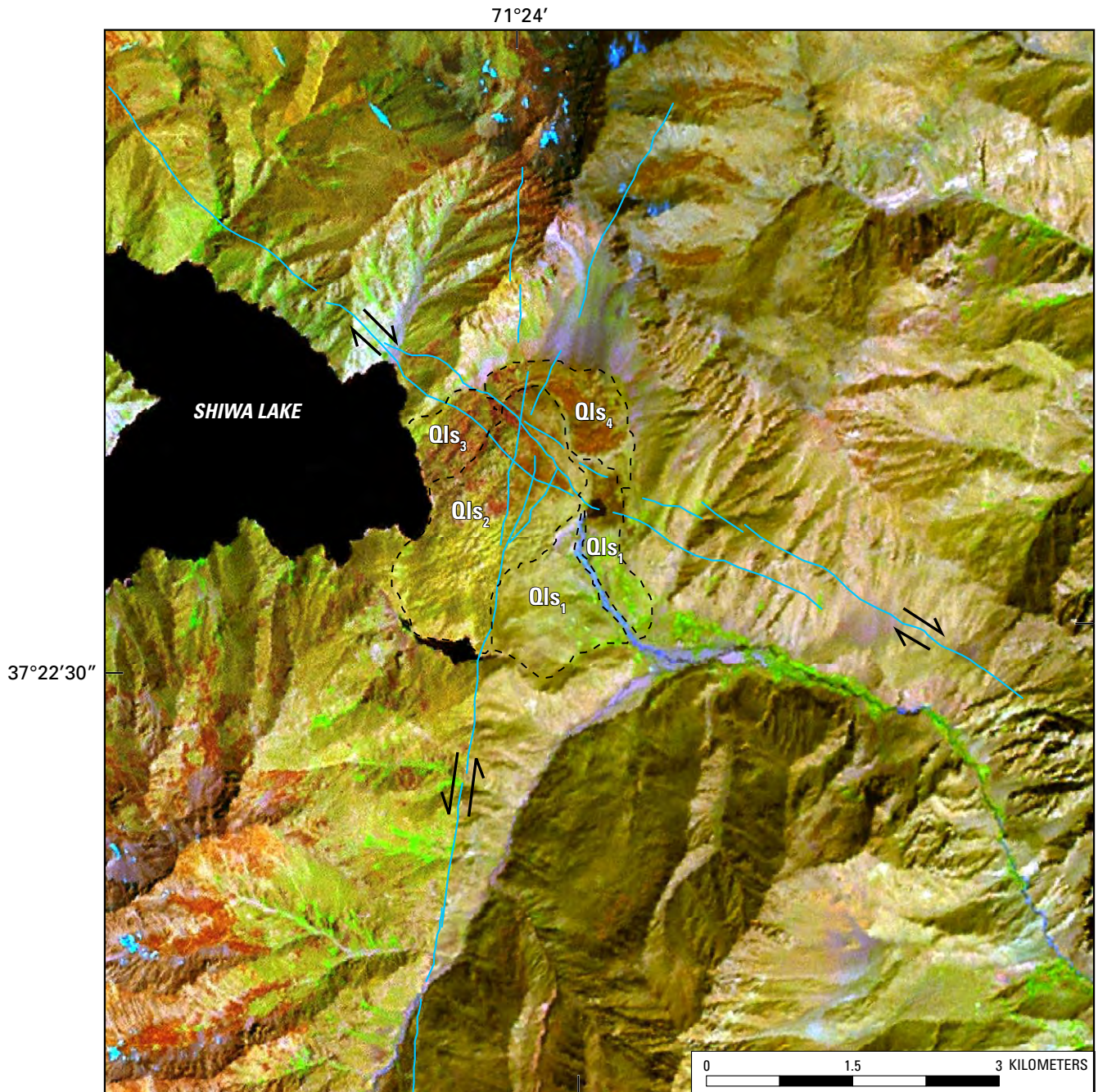
Figure 9. Surface expression of category C faults east of Shiwa Lake in the Hindu Kush, northeastern Afghanistan (pl. 1, no. 23). Shiwa Lake formed because several generations of landslides have dammed the valley. Landslides range in age from oldest ( Qls_1 ) to youngest ( Qls_4 ). These landslides are likely caused by earthquakes (that is, seismogenic landslides). The faults (blue lines with black arrows showing directions of movement) mainly cross bedrock slopes, but their expression on the surface of the landslides Qls_1 , Qls_2 , and Qls_3 indicates that recent movement on the faults is younger than the landslides and that the faults are active. The amount of fault displacement on the landslides could not be measured because of limited resolution of the imagery. Image is a panchromatically enhanced Landsat image that merges bands 7+4+1.
