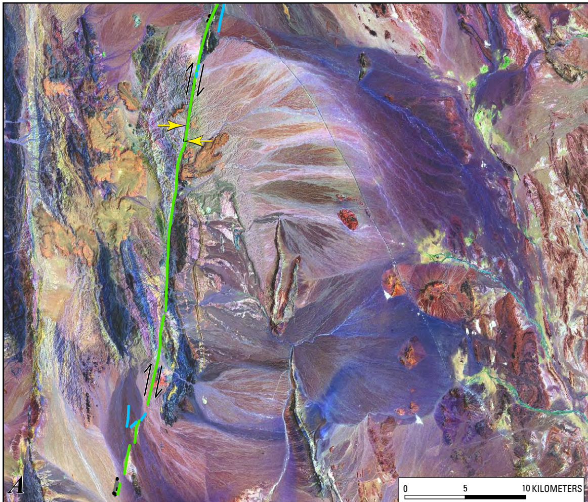
Figure 14A. Landsat image showing evidence of right-lateral movement on East Neh-West Asagie fault (pl. 1, no. 129) of the Sistan suture zone, Iran. Yellow arrows show a major drainage that is right-laterally offset. Black arrows adjacent to faults show directions of movement. Fault categories are category B, green; and category C, blue. Image is a panchromatically enhanced Landsat image that merges bands 7+4+1. See figure 14 for location.
