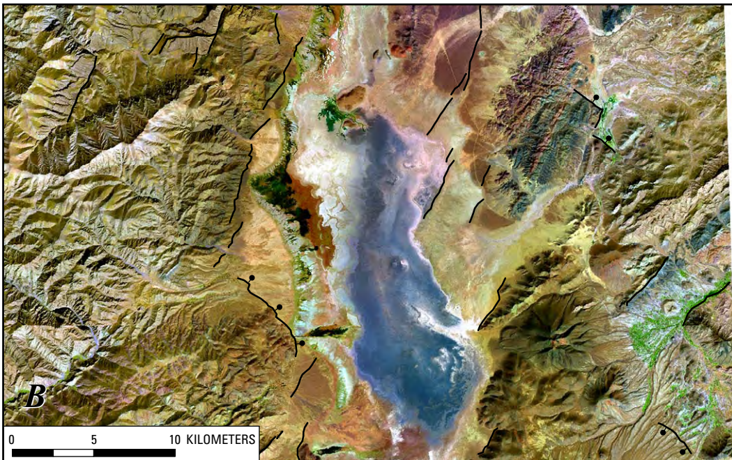
Figure 13B. Image showing pull-apart basin associated with Navar basin system fault (pl. 1, no. 63). This basin is between the northeast-striking, left-lateral Chaman and Dorafshan fault systems. Pull-apart basins commonly form at left steps in left-lateral systems. Faults are black lines; normal faults are shown by a bar-and-ball on the downthrown side. Image is a panchromatically enhanced Landsat image that merges bands 7+4+1. See figure 13 for location.
