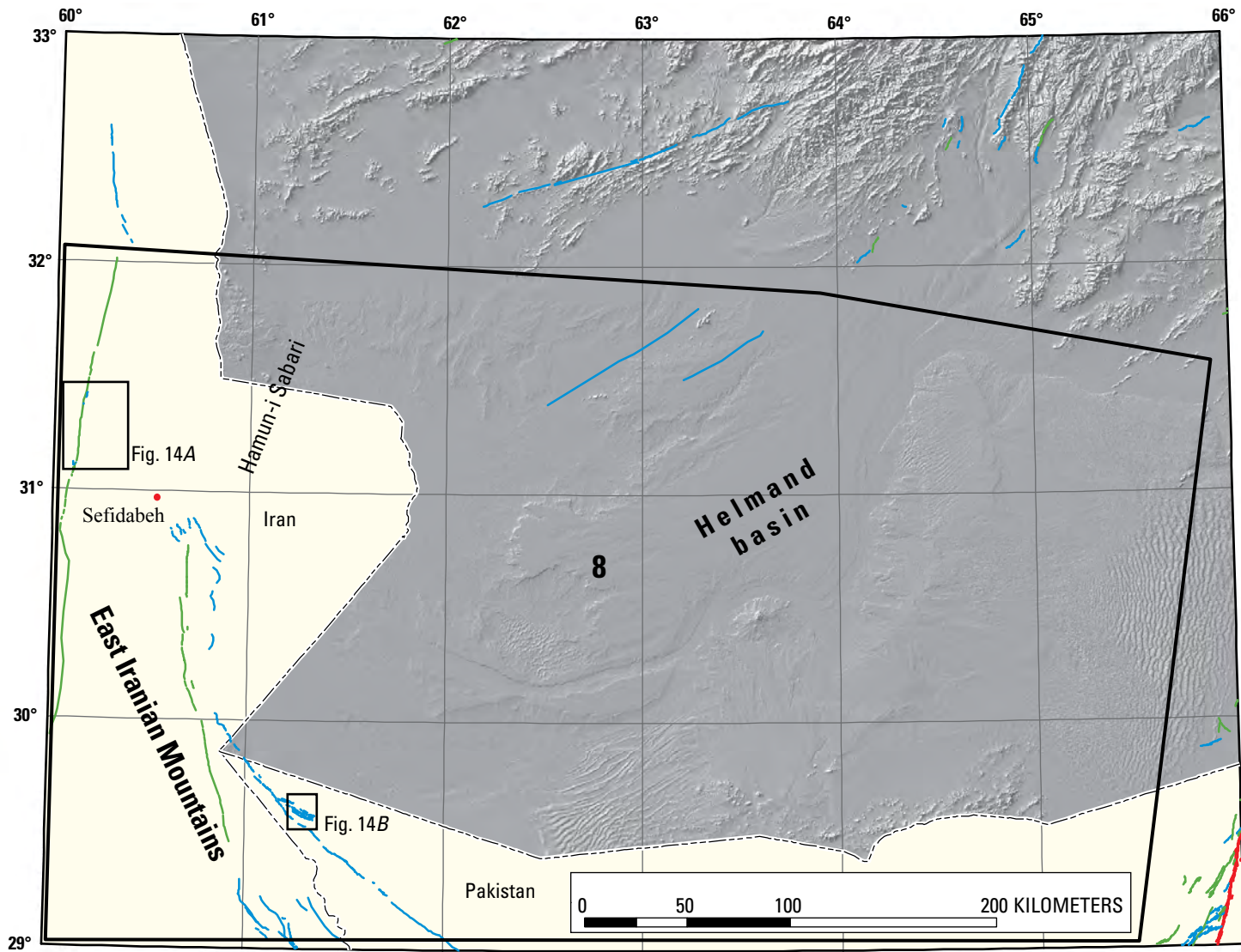
Figure 14. Tectonic domain 8—Helmand basin-Makran system outlined in black. This domain contains little evidence of active faulting and has very little seismicity in Afghanistan. Active faults and historical earthquakes in eastern Iran are part of the Sistan suture zone. Large areas of domain 8 in Afghanistan are covered by complexes of active sand dunes, which could bury and conceal evidence of active faults. Fault categories are category A, red; category B, green; and category C, blue.
