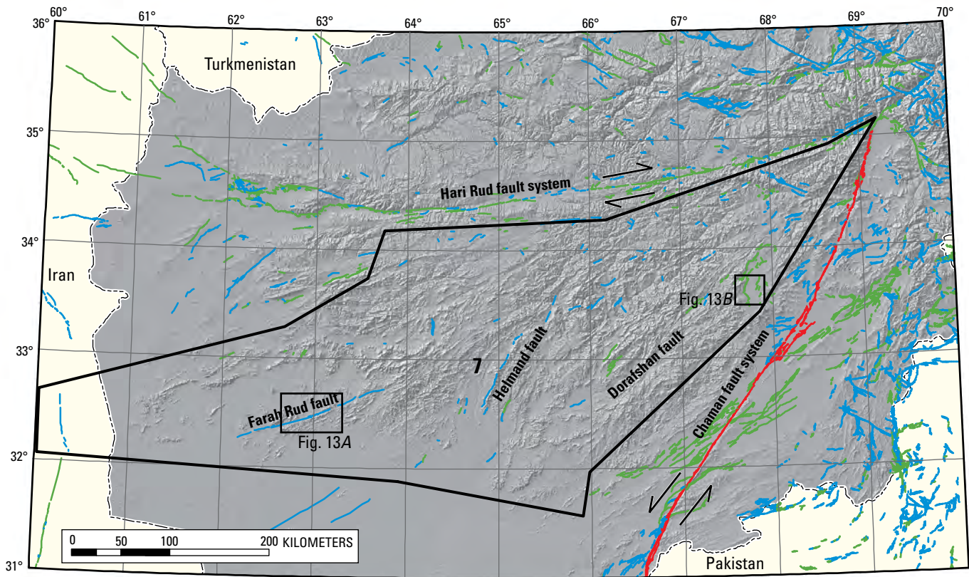
Figure 13. Tectonic domain 7—Central Afghanistan Accreted Terranes and the Helmand-Dorafshan fault system outlined in black. This structurally complex region consists of rugged northeast-trending mountains interspersed with valleys and basins. The region may be actively extruding to the southwest between the left-lateral Chaman fault system to the east and the right-lateral Hari Rud fault system to the north. Arrows indicates directions of movement on fault systems. Fault categories are category A, red; category B, green; and category C, blue.
