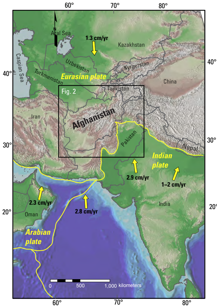
Figure 1. Location of study area in the greater Alpine-Himalaya orogenic belt of Asia. Vectors show relative plate motions and velocities between the Indian, Eurasian, and Arabian plates (plate boundaries shown and labeled in yellow). Plate velocities from Jade (2004), Bird (2003), Vernant and others (2004), and Sella and others (2002). Box shows area of figure 2.
