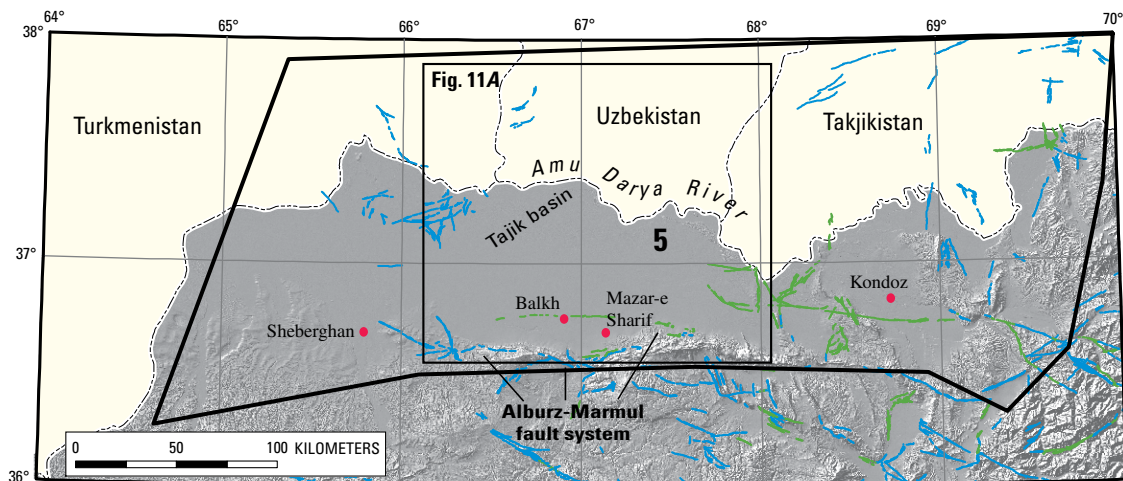
Figure 11. Tectonic domain 5—Tajik basin and Alburz-Marmul fault system outlined in black. The Amu Darya River is the northern boundary of Afghanistan in this area and major meanders in the river coincide with areas that show evidence of Quaternary faulting. Fault categories are category B, green; and category C, blue.
