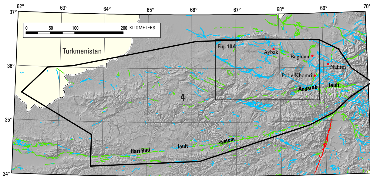
Figure 10. Tectonic domain 4—Hari Rud-Northern Afghan platform system outlined in black. The Andarab and Hari Rud fault systems in this domain probably play an important role in the westward extrusion of this region as a result of the Indian and Eurasian plate collision. In March 2002, a M 6.1 earthquake in Nahrin caused more than 1,000 fatalities and widespread damage. Fault categories are category A, red; category B, green; and category C, blue.
