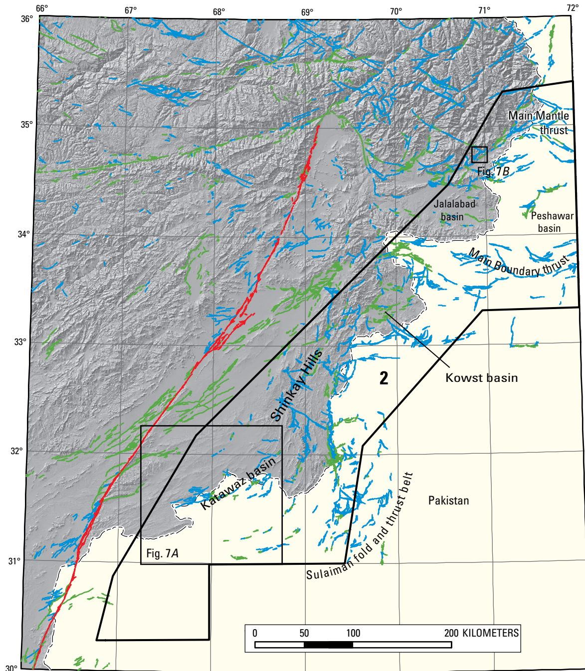
Figure 7. Tectonic domain 2—the Sulaiman fold-and-thrust belt and associated contractional zones outlined in black. Deformation in this domain is driven by west- to northwest-directed contraction related to the collision between the Indian and Eurasian plates. Fault categories are category A, red; category B, green; and category C, blue.
