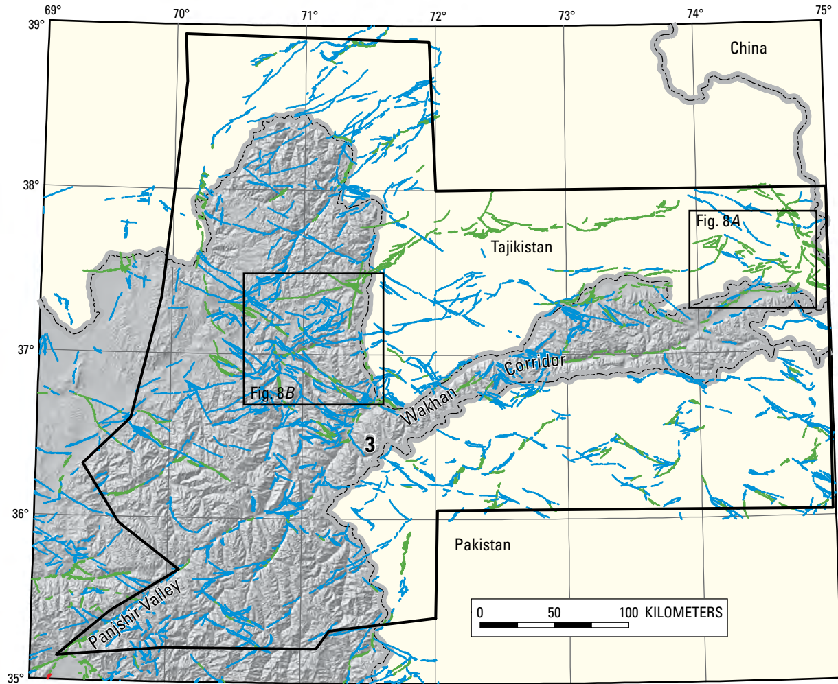
Figure 8. Tectonic Domain 3—Northeastern Afghanistan-Hindu Kush region outlined in black. The northeast-trending structures in this region appear to be part of an older structural grain, and the young structures are northwest-trending strike-slip faults. Fault categories are category A, red; category B, green; and category C, blue.
