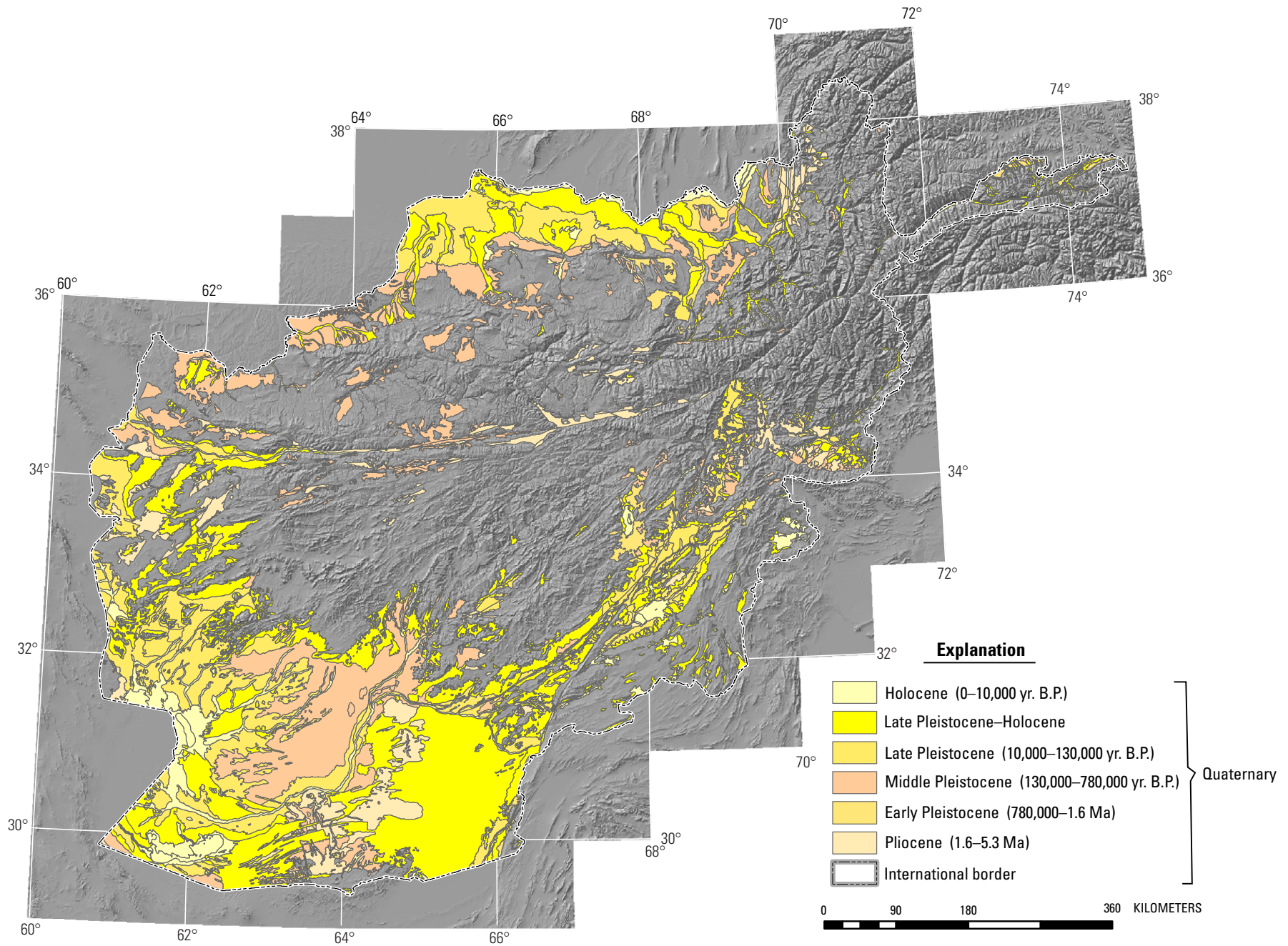
Figure 4. Quaternary geologic map of Afghanistan (from Doebrich and Wahl, 2006). Units are listed chronologically in the explanation. The Quaternary geology was previously mapped by Abdullah and Chmyriov (1977) and is primarily confined to large basins in southwestern and north-central Afghanistan. The lack of previously mapped Quaternary deposits in central and northeastern Afghanistan required that we rely on the geomorphic expression of features on the high-resolution imagery to identify active faults. B.P., before present; Ma, million years.
