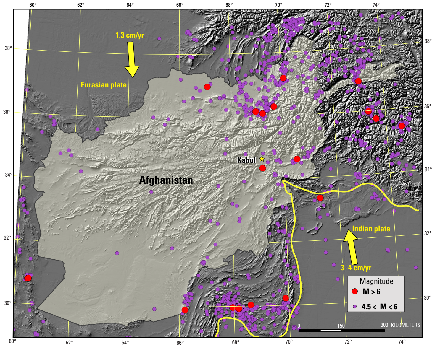
Figure 2. Shallow (< 35 km deep) historical earthquakes (Dewey, 2006) in and surrounding Afghanistan (light-shaded region). Open arrows show direction and rate of relative plate motion between Indian and Eurasian plates (Sella and others, 2002; Bird, 2003). Plate boundaries are shown in yellow. The abundant earthquakes and active faulting in Afghanistan are caused by the Indian plate moving northward beneath Eurasia at a rate of approximately 3–4 cm/yr. This collision has uplifted the Himalayan, Hindu Kush, and Pamir Mountains (unlabeled high terrain in northeastern section of map).
