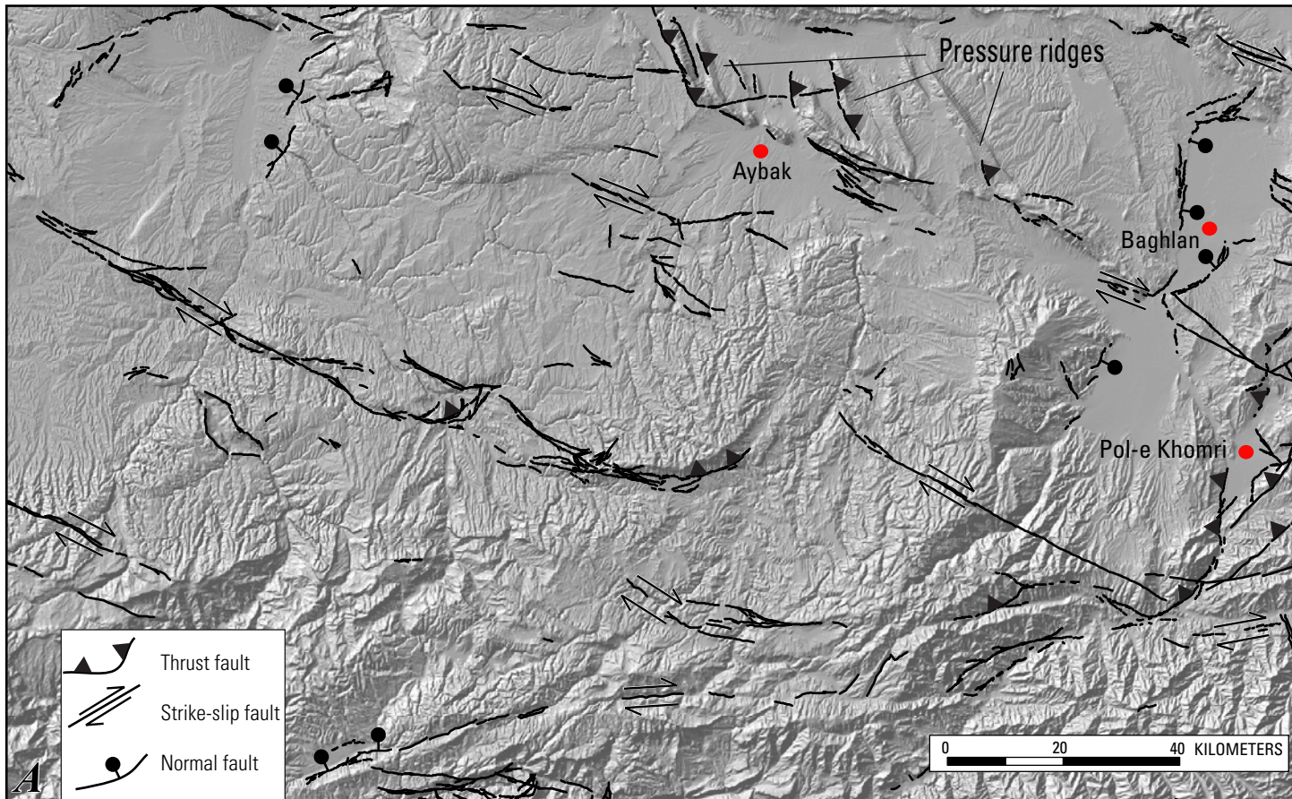
Figure 10A. Features in the Northern Afghan platform that are probably and possibly active, and that play a role in the area's tectonics. A network of northwest-trending, right-lateral strike-slip faults appear to be the main features in this area. Thrust faults develop where there are left steps in these strike-slip faults. Base map is from SRTM (Shuttle Radar Topographic Mission) data. See figure 10 for location.
