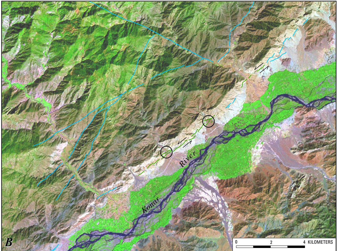
Figure 7B. Landsat image of part of the Konar fault system (pl. 1, no. 52). The range-bounding thrust fault shows evidence of left-lateral offset (indicated by arrows), whereas lineaments in the adjacent mountains are preserved on rapidly eroding bedrock hillslopes, which suggests that they are probably active and involve multiple fault strands. Fault categories are category B, green; and category C, blue. Image is a panchromatically enhanced Landsat image that merges bands 7+4+1. See figure 7 for location.
