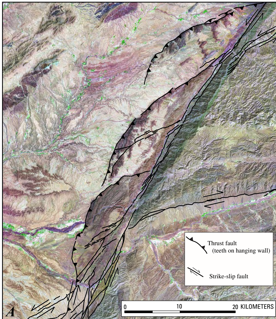
Figure 6A. Active frontal thrust faults along western margin of the left-lateral strike-slip Chaman fault (pl. 1, no. 94). Image is a panchromatically enhanced Landsat image that merges bands 7+4+1. The strike-slip strands of the Chaman fault system extend from the upper right to the bottom left of the view. The arcuate, northwest-directed, frontal thrust faults are second-order structures that result from the combination of compression and strike-slip motion on the Chaman fault system. See figure 6 for location.
