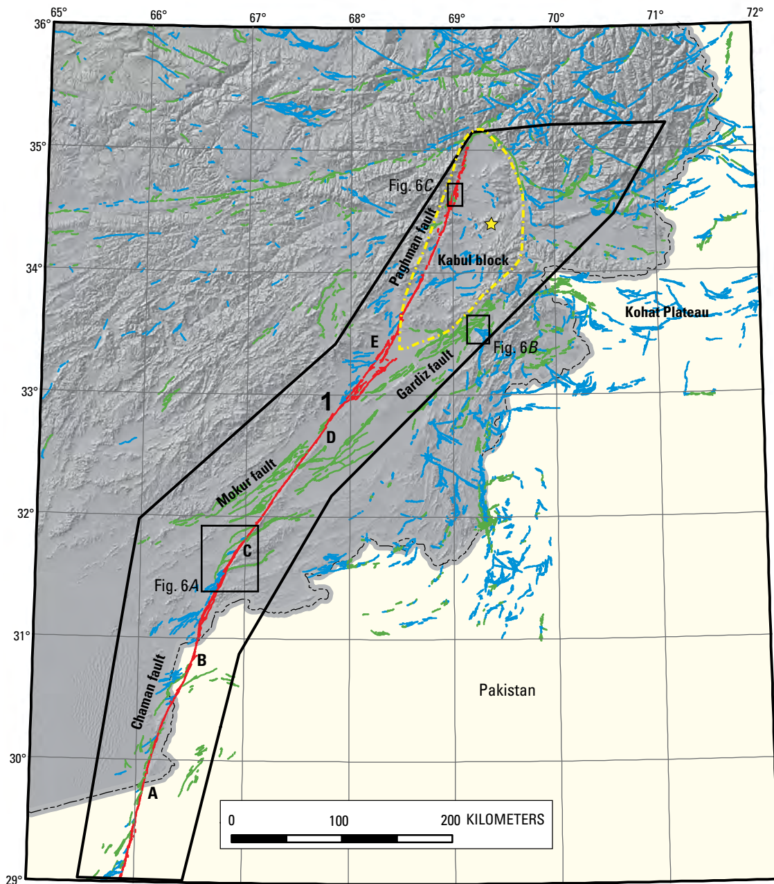
Figure 6. Tectonic domain 1—the Chaman fault system outlined in black. Dashed yellow line shows approximate boundary of the Kabul block. Sections of Chaman fault shown by letters A–E . Fault categories are category A, red; category B, green; and category C, blue. Yellow star shows location of Kabul.
