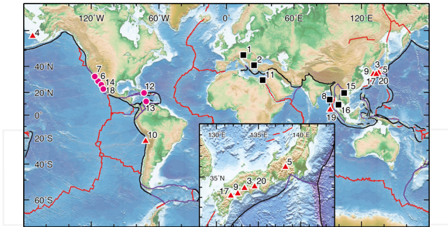
Figure 5. Strike-slip basins at plate convergent margins. Red triangles, trench-linked; black squares, indent-linked; purple circles, plate-boundary transform faults. Numbers correspond to those in Table 1
