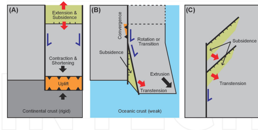
Figure 7. Typical geometry of termination areas of strike-slip faults. (A) If the block collides with a rigid continental crust, it shortens and is uplifted, accompanied by thrusts. At the opposite side to the uplift, upper crust is mechanically pulled away, leading to subsidence. (B) If the block extrudes with a rotational component into a weak oceanic crust (a transtensional setting), a sedimentary basin forms at the end of the strike-slip fault. Examples include the Yinggehai Basin, which is related to the extrusion of the Indochina Block, and the Gulf of California, which is related to the transtensional movement of the Baja California Peninsula. (C) The strike-slip fault diffuses its displacement through splayed extensional normal faults at its end [44]. An example is the Cerdanya clastic basin formed by late Miocene normal faulting at the termination of the La Tet strike-slip fault, Spain [51].
