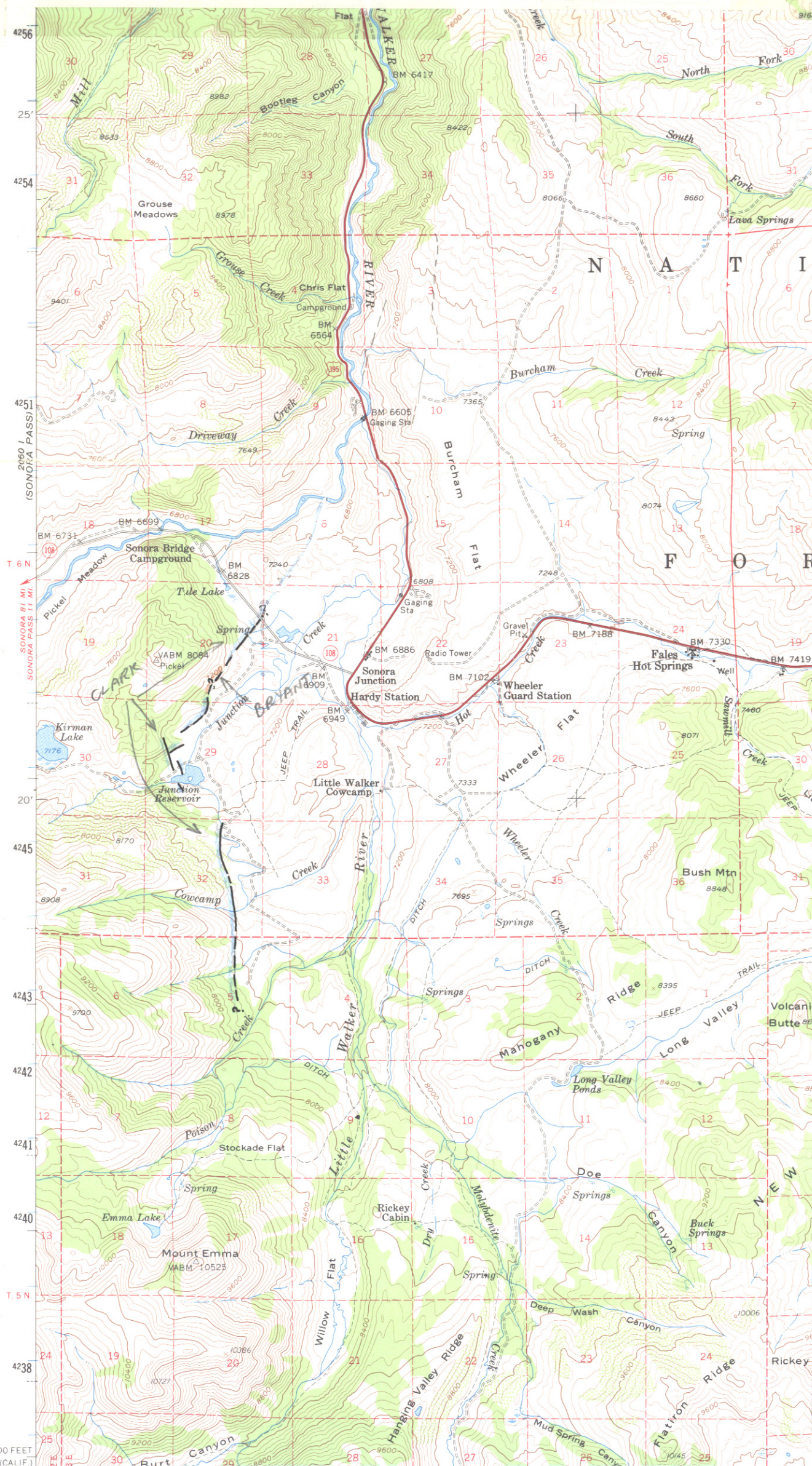
Figure 5c (to FER-154). Faults in the Fales Hot Springs quadrangle recommended for zoning for special studies.
