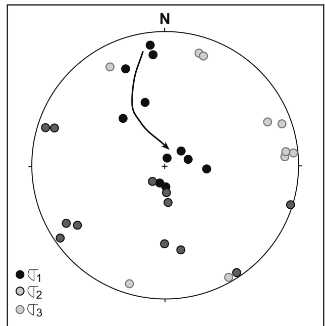
Fig. 7 Stereographic plots of fault slip data for the KMG. Note the migration of principal stress direction (confirmed by the most confident minimum stress direction) from N-S compression to NE-SW extension.
