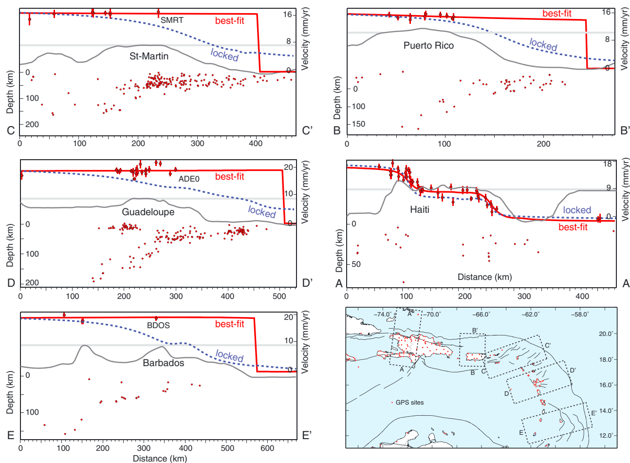
Figure 14. Sections across the Lesser and Greater Antilles subduction showing topography (grey line), earthquake hypocenter [Engdahl et al., 1998], velocity magnitude at the GPS sites (red circles with 95% confidence error bar), velocity predicted by the best fit model (solid red line), and velocity predicted by a forward model where we impose full coupling on the subduction interface (dashed blue line). The misfit of the data to a fully locked plate interface is apparent on the three Lesser Antilles cross sections.
