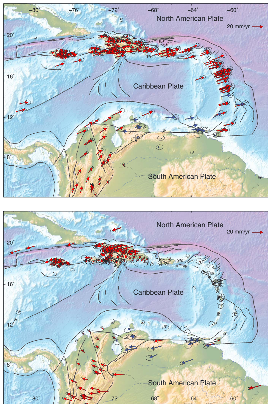
Figure 2. (top) GPS velocities used in the model shown with respect to the North American plate defined by the velocity of 25 GPS sites located in the stable interior of the plate [Calais et al., 2006]. (bottom) GPS velocities shown with respect to the Caribbean plate as defined in the best fit block model described in the text. Error ellipses are 95% confidence. Blue arrows show GPS velocities from Pérez et al. [2001] in Venezuela because of their large uncertainty and the lack of common sites with our solution, which prevents us from rigorously combining them to our solution. They are not used in the model but used to show that they are consistent with the rest of the velocity field.
