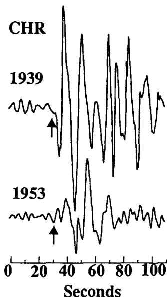
Fig. 13. Plot of P waveforms recorded at CHR for the 1939 (Dist = 81.2°) and the 1953 (Dist = 80.5°) earthquakes. The P waveforms are plotted with a 30 s noise window before the first arrival as indicated by the arrows. The 1939 event has a dilatational first motion and the 1953 event has a more nodal but compressional first motion.
