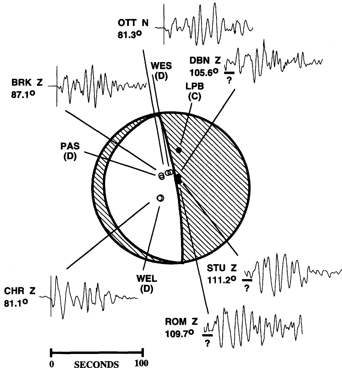
Fig. 10. P -wave first motion focal mechanism and waveforms for the 1939 earthquake. The shallow plane is completely unconstrained from the first motions. Note the difficulty in picking the first motions at stations in Europe (ROM, STU and DBN).
