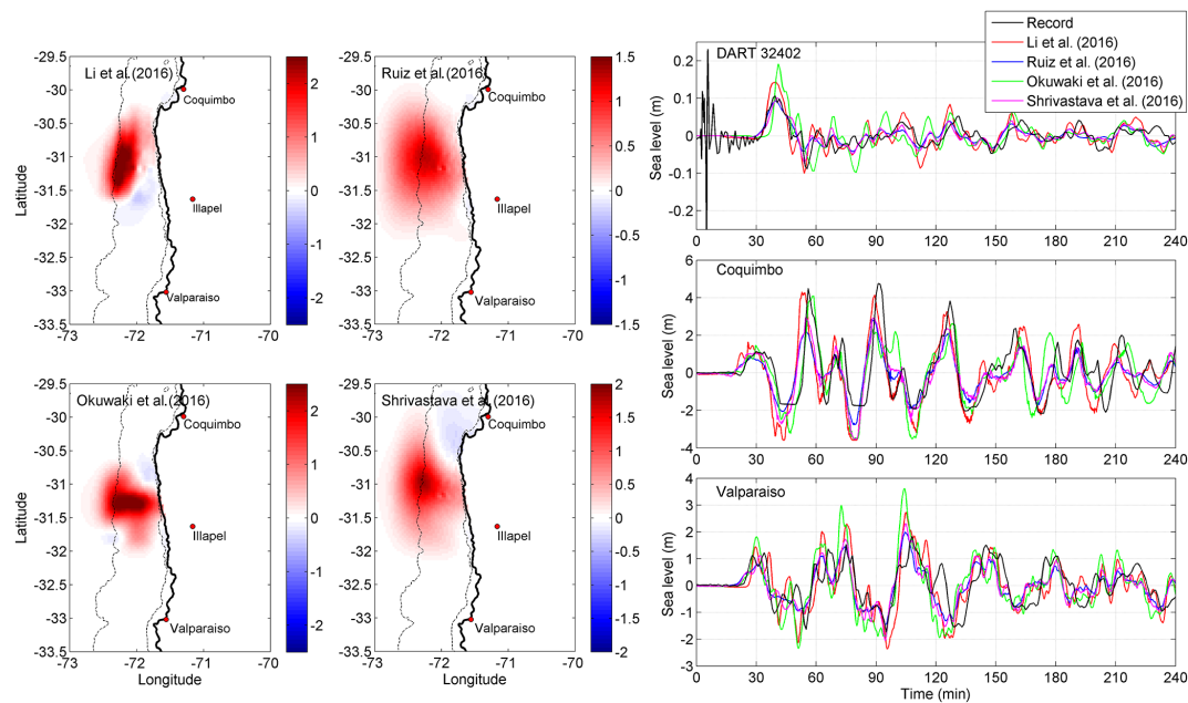
Figure 5. Tsunami initial conditions of four source models and comparison of tsunami records with simulated tsunami waveforms at DART 32402, Coquimbo and Valparaíso.
