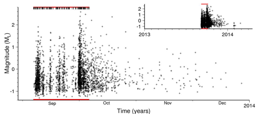
Figure 2. Magnitude of earthquakes in Harrison County (crosses) identified from template matching using nearby station O53A. Red bars indicate duration of nearby hydraulic fracturing, with black bars showing individual stages. Inset shows the entire time frame over which the template matching was performed based on nearby EarthScope station availability.
