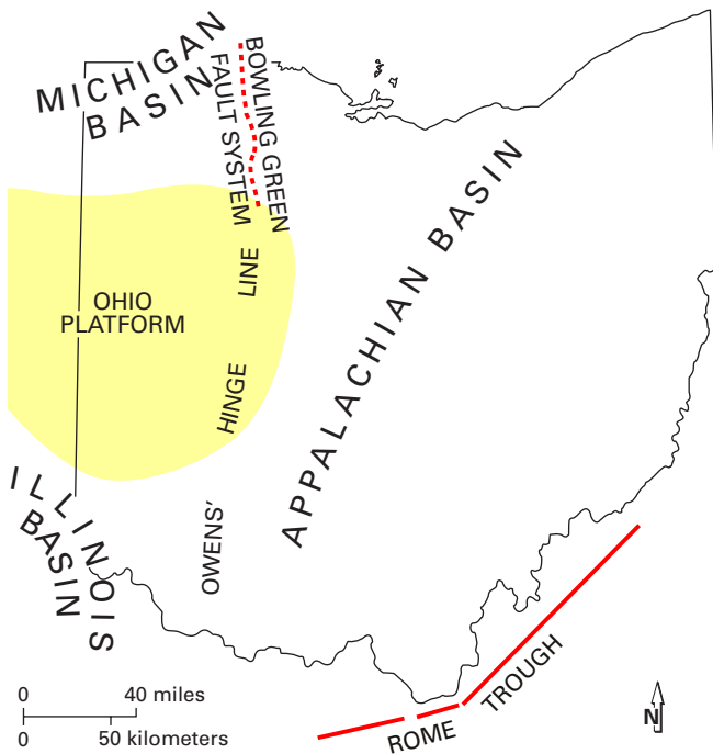
FIGURE 1.—Major deep “pre-Ordovician” structural features in Ohio and surrounding region.
