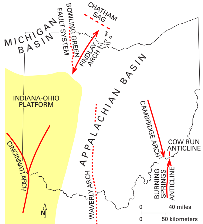
FIGURE 2.—Major shallow “post-Cambrian” structural features in Ohio and surrounding region.
