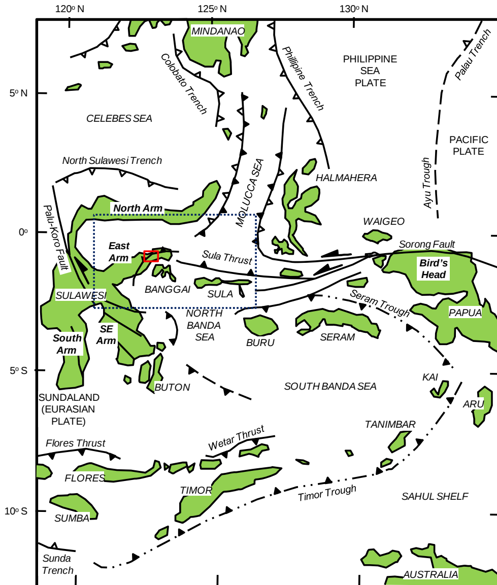
Figure 1 - Regional tectonic setting of East Indonesia (modified after Hamilton, 1979; Letouzey, 1983; Moss & Wilson, 1998; Hall, 2012). Red-line square is the study area, whilst the blue-dotted one is inset for Figure 2.
