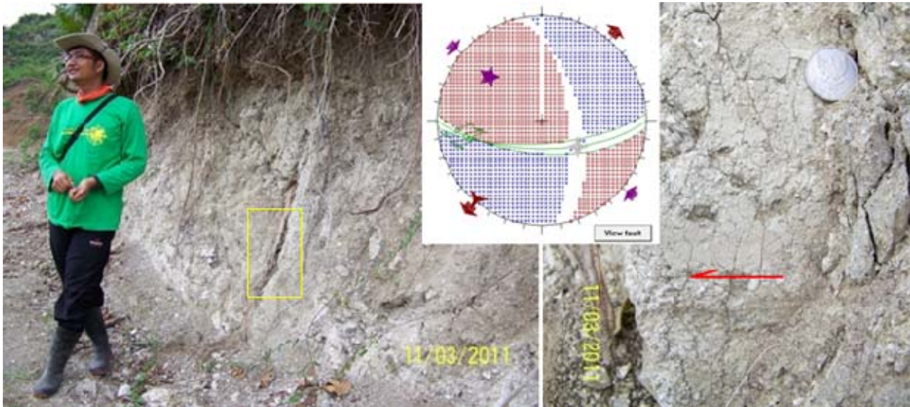
Figure 10 - Altered gabbro dissected by an E-W dextral fault, outcropped at Siuna Village. Kinematic analysis suggesting a NW-SE compression. Camera facing north, location is indicated by (c) on SRTM image at Figure 8.
