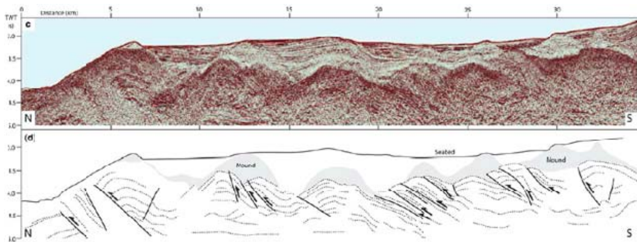
Figure 4 - Another seismic line of BS07-20 that crossing the extension of Batui Thrust offshore to the east (Watkinson et al. , 2011). A series of north-vergent thrusts can be clearly observed. Location map is depicted in Figure 2.
