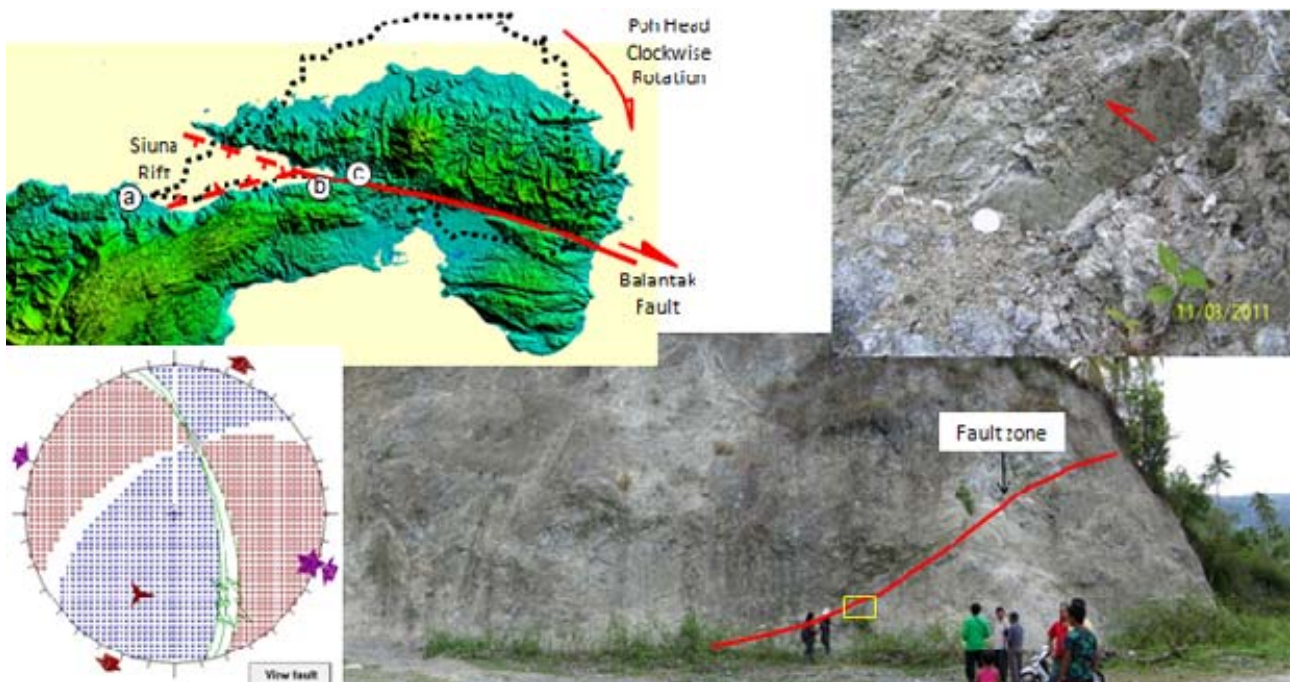
Figure 8 - Ophiolites outcrop at Pagimana, composed of highly sheared gabbro (white-green) and basalt (dark-green), with numerous magnesite veins mainly following existing fault planes. Kinematic analysis on an inverse fault (see inserted graph and photo) suggests a SE-NW compression and NE-SW extension once had working on the area. This fault zone might represents a NE extension of Siuna rifting along the western part of Balantak Fault. Camera facing south, location is indicated by (a) on SRTM image.
