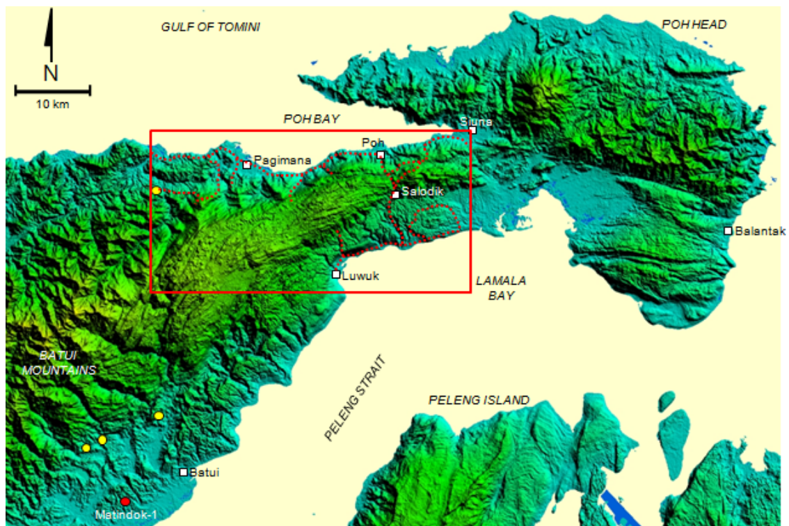
Figure 3 - Field traverse map on SRTM image. Red-line rectangle is the study area. Red-dotted lines are field traverse. Yellow circles are hydrocarbon seepages (after Rusmana et al. , 1993; Suroño et al. , 1993). Red circle is gas-producing well of Matindok Field.
