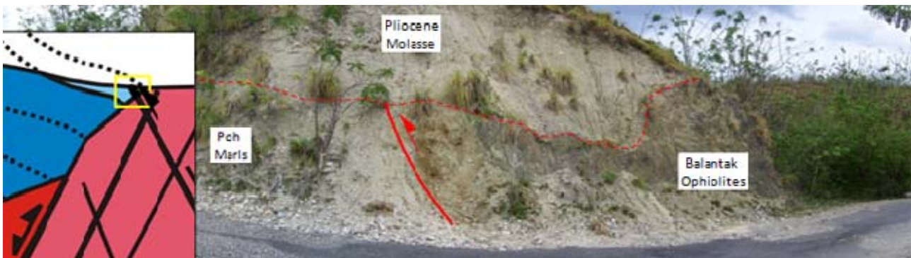
Figure 11 - Structural contact (high-angle reverse fault) between Balantak Ophiolites and the Tertiary Poh marls, both are eroded and covered by Pliocene molasse of Kintom Formation. This outcrop suggests an initial inversion of the Balantak Ophiolites at Late Miocene. Camera facing west, location is indicated by (b) on geologic map and cross-section at Figure 7.
