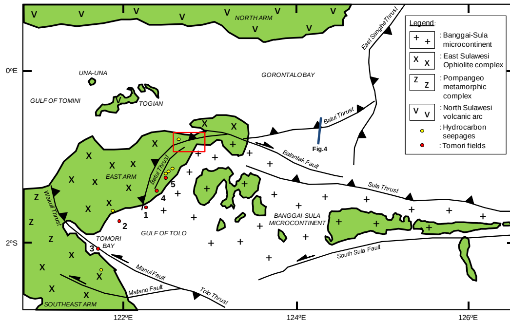
Figure 2 - Regional configuration of fundamental tectonic elements for the East Arm of Sulawesi and its hydrocarbon indication (modified after Garrard et al. , 1988; Davies, 1990; Rusmana et al. , 1993; Simandjuntak et al. , 1993; Simandjuntak et al. , 1997; Suroño et al. , 1993; Moss & Wilson, 1998; Watkinson et al. , 2011). Existing hydrocarbon fields are marked by numbers: 1 - Mantawa, 2 - Tiaka Kalamba, 3 - Dongkala Tolo, 4 - Minahaki, and 5 - Matindok. Red-line square is the study area. Blue lines are location of seismic line in Figure 4.
