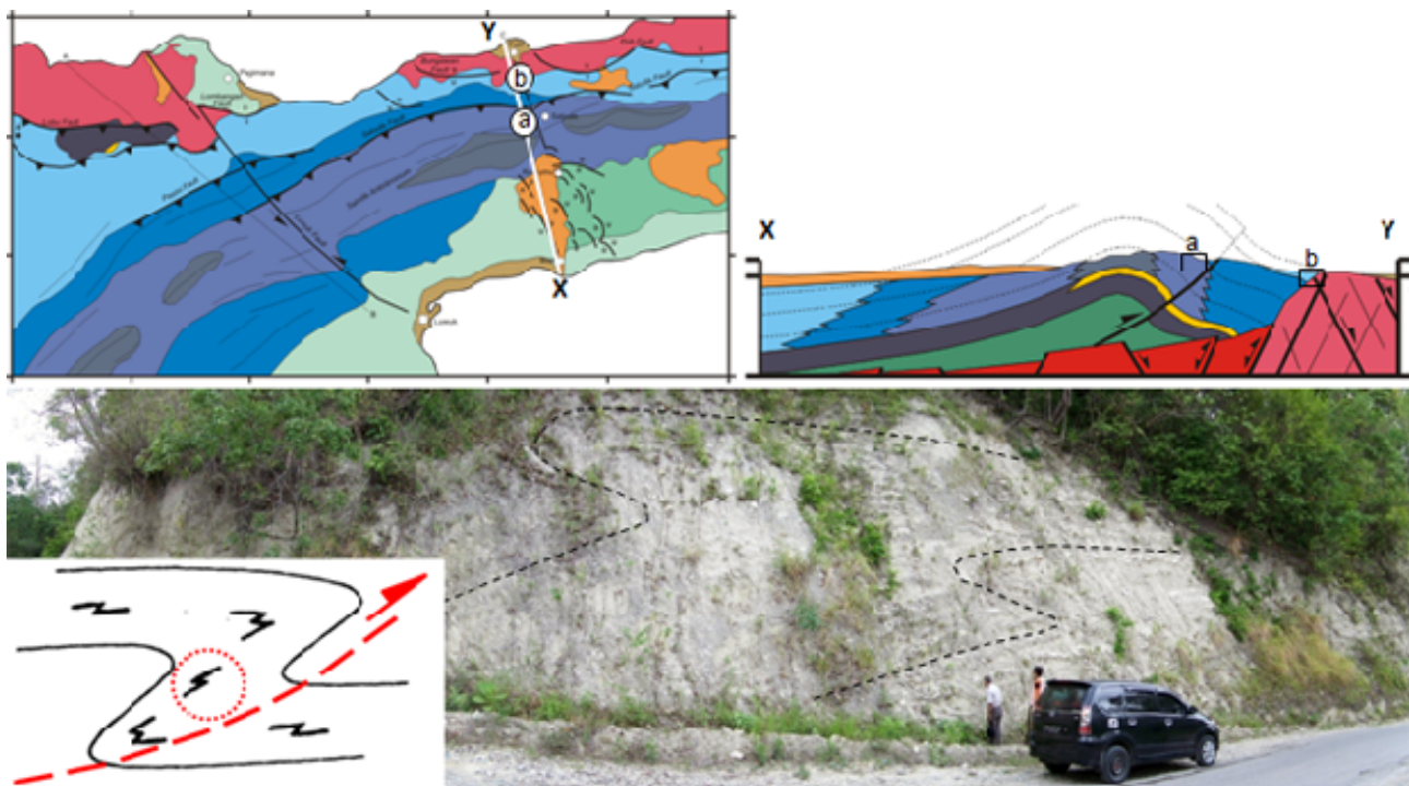
Figure 7 - S-shaped parasitic minor folds in the Tertiary Salodik grainstones, suggesting a major recumbent fold crest located to the south of the location (ref: McClay, 1987). A northwest-vergeance thrust is most likely located to the north of the location. Camera facing west, location is indicated by (a) on geologic map and cross-section.
