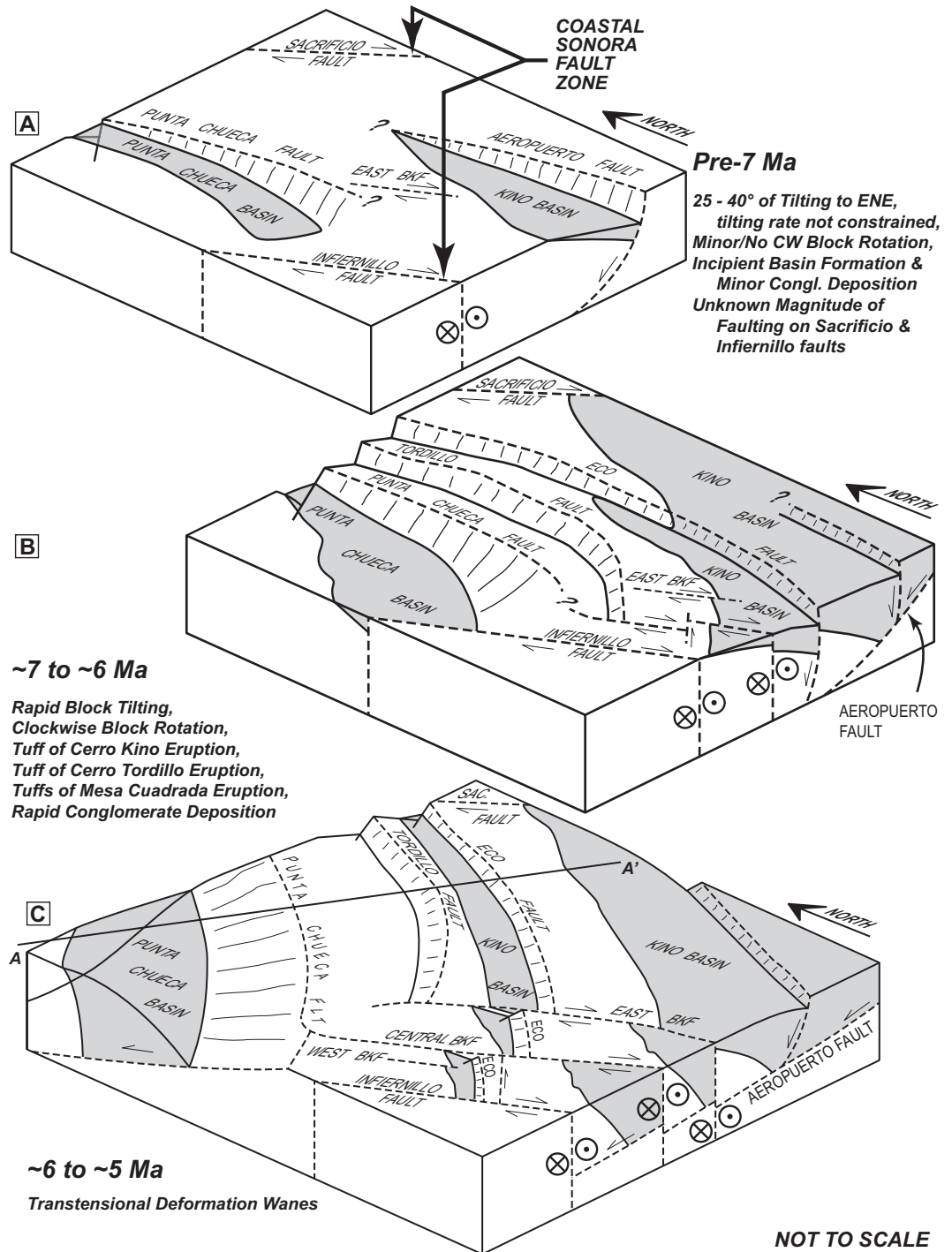
Figure 15. Oblique block diagrams showing the evolution of the transtensional Coastal Sonora fault zone. (A) Sometime after 11.5 Ma, dextral transtension initiated across the Coastal Sonora fault zone via dextral faulting on the Sacrificio and Infiernillo strike-slip faults. Associated block tilting and minor block rotations occurred in the intervening region, forming tectonic basins that began to accumulate nonmarine deposits. (B) By 7 Ma, transtensional deformation and basin sedimentation became rapid. Deformation in the south continued via block tilting and rotation, as discrete strike-slip structures began to form. First-generation normal faults slipped and rotated to lower angle (e.g., Aeropuerto fault), and new second-generation faults initiated. (C) During the final phase of transtension, dextral deformation occurred via block rotation and along discrete dextral faults in the southern and central parts of the study area, while in the north, dextral deformation continued to be accommodated entirely via clockwise rotation of the Punta Chueca basin and continued slip on the low-angle Punta Chueca normal fault. CW—clockwise; BKF—Bahía Kino fault; SAC—Sacrificio.
