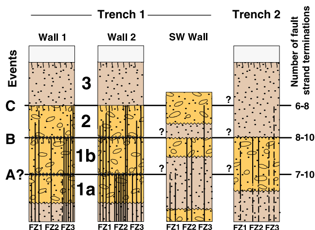
Figure 7. Vertical extent of fault strands (solid vertical lines) in fault zones relative to the stratigraphic position of surface faulting events A?, B, and C in trenches 1 and 2. Patterns, symbols, and labels for faulting events, stratigraphic sequences, and fault zones as in Figures 4 and 6. Indistinct or inferred parts of strands are dashed. The range in the number of terminations for each faulting event (right edge of figure) is the number of distinct strands and the total number of strands. Question marks indicate uncertainty in the correlation of faulting events to strands in the southwest wall of trench 1 and in trench 2. Although as many strands were mapped terminating near the position of event A? as for any other event (7–10), all but one of the distinct strands terminating at this position were in one fault zone (FZ2, wall 2). For this reason, we cannot demonstrate that event A? is a separate faulting event.
