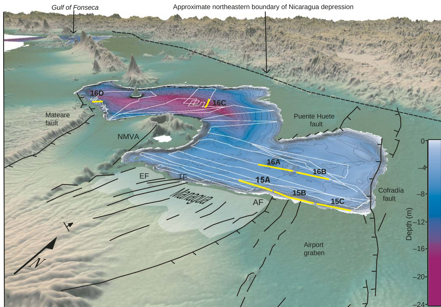
Figure 14. Oblique view of Lake Managua showing the low-lying Nicaraguan depression bounded to the northeast by the interior highlands and to the west by the Mateare fault (MF) and the axis of the Central America volcanic front. The main goals of the survey were to map the surficial expression of the Nejapa-Miraflores volcanic alignment (NMVA), Estadio fault (EF), Tiscapa fault (TF), and Aeropuerto fault (AF) into Lake Managua. Figures 15, 16A, and 16B show examples of scarps found near the southern lake shoreline indicating the large number of parallel and closely spaced faults projecting outward from the capital city Managua (Woodward-Clyde Associates, 1975). Figures 16C and 16D show vertical offsets typical of the Momotombito fault and Mateare fault, respectively.
