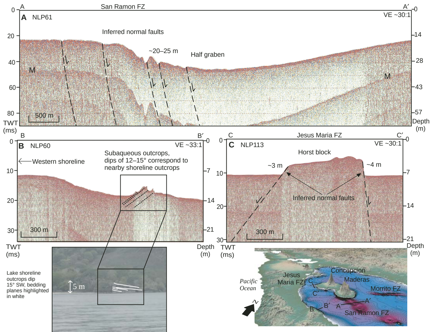
Figure 19. (A) 3.5 kHz subbottom profiler line NLP61 crossing San Ramon fault zone (FZ) in Lake Nicaragua. This area forms the deepest part of the lake, ~40 m in depth near the southern coast of Maderas volcano. The fault forms a linear trend approximately N45°W and controls an asymmetrical depocenter to the southwest. (B) This line near the western shore of the lake exhibits rock subcrops that are most likely part of the adjacent, onshore Rivas Formation. Based on the profile and outcrops seen near the shoreline during the survey, the bedding planes of the Rivas Formation dip 12°–15° to the west-southwest. (C) The second major fault zone in Lake Nicaragua, the Jesus Maria fault zone, trends approximately east-west and is associated with an anomalously uplifted, elongate ridge on the lake floor. Both sides of this linear feature appear to be fault bounded, show 3–4 m of vertical offset, and appear to be uplifted near the center of a more broad bathymetric high between Concepcion volcano and the western shoreline of the lake. VE—vertical exaggeration.
