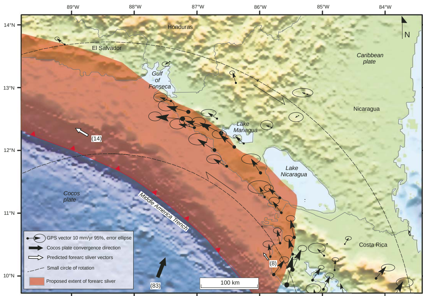
Figure 4. Global positioning system (GPS) plate convergence vectors from DeMets (2001) superimposed on bathymetry and topography from Sandwell and Smith (1997). GPS vectors in Nicaragua are from Turner et al. (2007), and vectors in Costa Rica are from Lundgren et al. (1999) and Norabuena et al. (2004). Most vectors show a uniform pattern of trench-parallel motion of a forearc sliver at 14 \pm 5 mm \text{yr}^{-1} in Nicaragua and 8 \pm 3 mm \text{yr}^{-1} in Costa Rica relative to a fixed Caribbean plate. Small circles of rotation are based on the Euler pole ( 8.9^\circ\text{N} , 88.4^\circ\text{W} ) from Turner et al. (2007).
