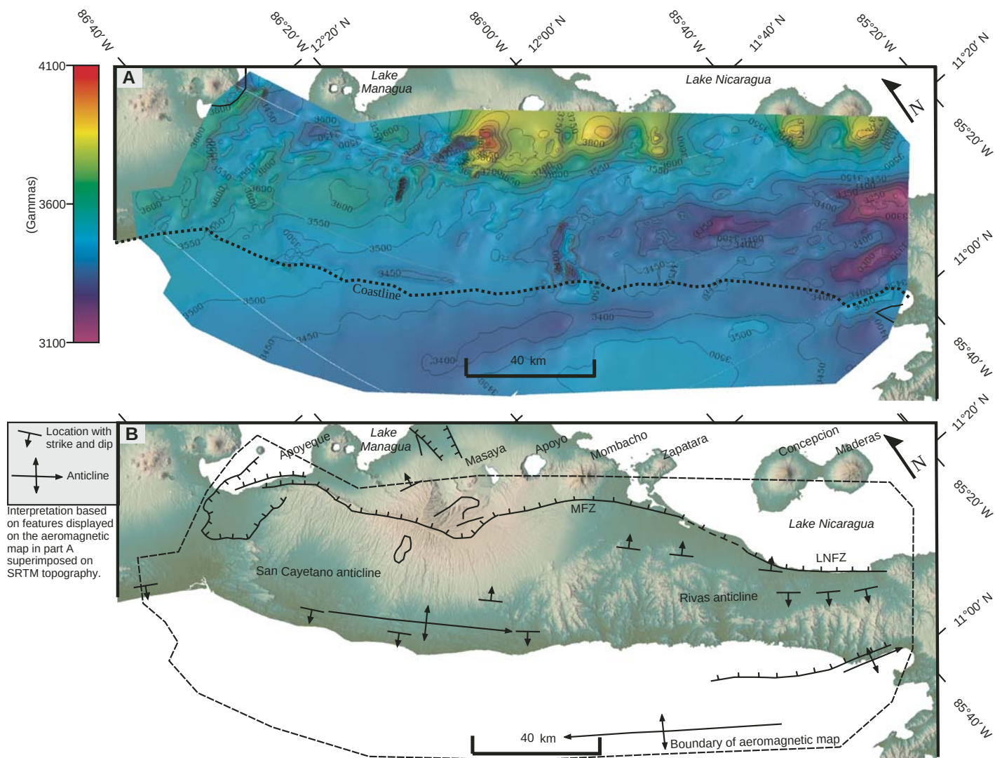
Figure 21. (A) An aeromagnetic data set (contour interval 50 gammas) acquired in 1969 by Superior Oil Associates covering the Pacific coast and the western regions of Lake Managua and Nicaragua. (B) Aeromagnetic interpretation is critical in correlating known offshore faults and folds with the onshore geology and helps constrain the location of the poorly known southwestern boundary fault of the Nicaraguan depression, the Morrito fault zone (MFZ) and the Lake Nicaragua fault zone (LNFZ). Faults and folds are based on the interpretation of aeromagnetic data from the Lake Nicaragua and Managua surveys and previously published geologic maps.
