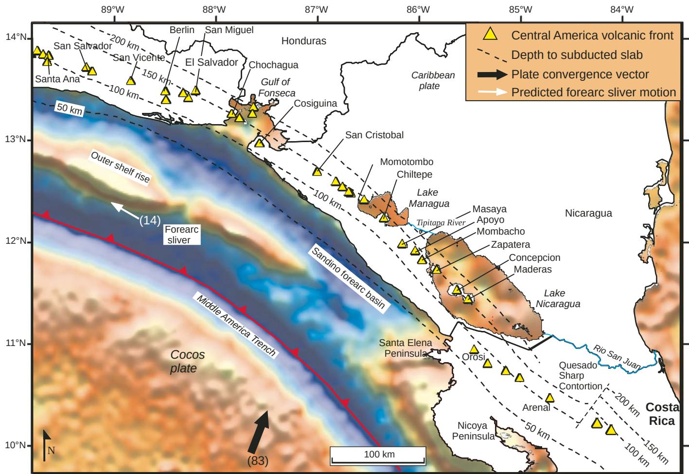
Figure 3. Geosat marine gravity map showing the change in strike of the Middle America Trench, the outer shelf rise, Sandino forearc basin, major Quaternary volcanoes, and trends of Lakes Managua, Nicaragua, and Gulf of Fonseca, which occupy the Nicaraguan depression. Major stratovolcanoes along the Central America volcanic front are marked by yellow triangles. The trend of the Central America volcanic front shows discrete, right-lateral offsets that range in length from 15 to 25 km. Slab contours from Syracuse and Abers (2006).
