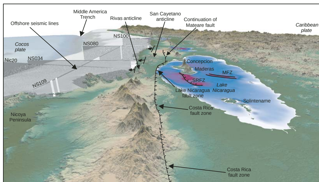
Figure 18. Inferred trace of the Costa Rica–Lake Nicaragua fault that offsets the northwestern edge of the Quaternary Central America volcanic front in Costa Rica and projects along the southwestern shore of Lake Nicaragua. This fault system exhibits ~300–800 m of vertical topographic relief in Costa Rica and forms a continuous scarp for ~50–60 km. The Costa Rica fault zone is responsible for southwesterly tilts in Quaternary volcanic deposits in the area south of Lake Nicaragua. Southwestward dips on strata protruding from the coastal plain south of Lake Nicaragua support the presence of the Lake Nicaragua fault zone near the present lake coastline. MFZ—Morrito fault zone, SRFZ—San Ramon fault zone.
