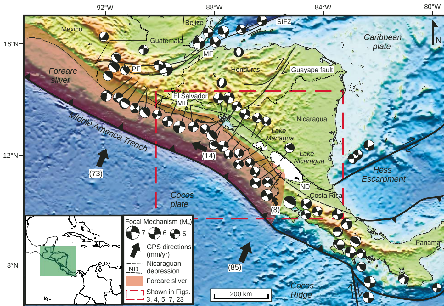
Figure 1. Tectonic setting of Central America displayed on satellite topography and bathymetry from Sandwell and Smith (1997). Subduction of the Cocos plate beneath the Caribbean plate occurs along the Middle America Trench. Global positioning system (GPS)-based plate velocities are relative to a fixed Caribbean plate, and focal mechanisms are from the Harvard Centroid Moment Tensor (CMT) catalog for all events from 1976 to 2007. Northwestward arc-parallel translation of the Central America forearc sliver (red shading) occurs at 7–8 mm yr -1 on Nicoya Peninsula of Costa Rica (Norabuena et al., 2004) and 14 mm yr -1 in Nicaragua (DeMets, 2001). The boundary between the Caribbean and North American plate occurs along the left-lateral strike-slip Swan Islands fault zone (SIFZ), Polochic fault (PF), and Motagua fault (MF).
