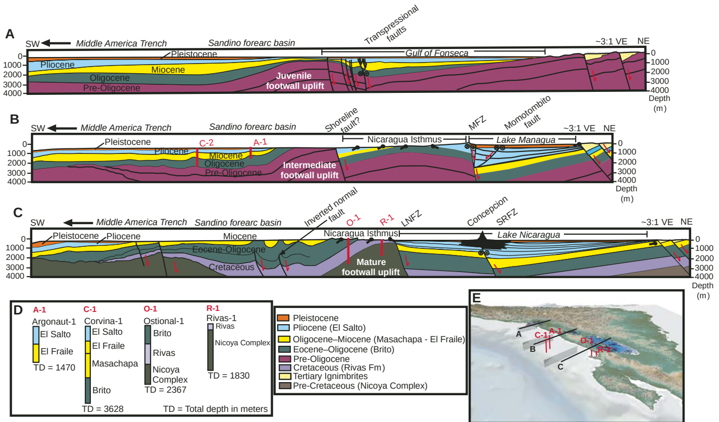
Figure 23. (A) The Gulf of Fonseca segment exhibits a half-graben structure with northeastward-dipping normal faults bounding the Nicaraguan depression. There is no offshore folding trenchward of the Central America volcanic front along this segment. Offshore seismic data and wells interpreted from Ranero et al. (2000) and Stephens et al. (2007) and volcanic dating (Ehrenborg, 1996; Balzer, 1999; Plank et al., 2002) indicate an uplift event occurred prior to the Oligocene–Miocene; however, the least amount of erosion and youngest rocks exposed suggest it is in juvenile stage of footwall uplift. VE—vertical exaggeration. (B) The Lake Managua segment exhibits a half-graben structure bound to the southwest by northeasterly dipping normal faults. The Mateare fault bounds the Nicaragua depression as a deeply rooted, steeply dipping normal fault; the antithetic Momotombito normal fault to the northeast is inferred to dip to the southwest. These faults may represent weak zones of the Central America volcanic front that have been preferentially reactivated during the current transtensional strike-slip phase of deformation (Weinberg, 1992). MFZ—Morrito fault zone. (C) The Lake Nicaragua segment shows localized folding and thrust faulting in the offshore region and two main normal faults bounding the Nicaraguan depression. The Rivas anticline underlies much of the narrow Nicaraguan Isthmus area and may represent a normal footwall block bounding the southwestern edge of the highly asymmetrical Nicaraguan depression. The San Ramon fault zone (SRFZ) is interpreted as a synthetic normal fault to the main bounding normal fault of the depression (Lake Nicaragua fault zone [LNFZ]) that produces the overall basin asymmetry. (D) Core data modified from Ranero et al. (2000) were used to construct cross-sections B and C. (E) Oblique view of the Cocos-Caribbean subduction zone showing locations of the cross sections and wells.
