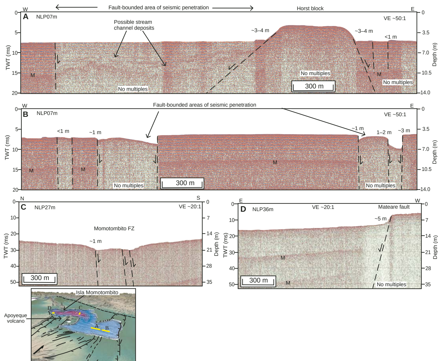
Figure 16. Subbottom profiler lines acquired in Lake Managua that achieved limited seismic penetration. (A) The fault-bounded areas of seismic penetration represent a poorly understood change in the seismic characteristics of the lake bottom. There is a drastic difference inside and outside of these “acoustic windows,” which are commonly bounded on at least one side by an active fault. The only positive bathymetric feature is a horst block with a north-south trend. (B) These fault offsets in the eastern part of the lake have a unique geometry. Offsets occur along a set of faults with a convex-concave asymmetry and exhibit between 1 and 3 m of vertical offset. (C) The central deep of Lake Managua is controlled by the Momotombito fault, which terminates before reaching Isla Momotombito and before wrapping entirely around Apoyeque volcano on the peninsula in the southern part of the lake. (D) Previous workers proposed that the onshore Mateare fault represents a fault line scarp that has been eroded from a scarp located more to the northeast. However, results from this survey suggest that the scarp found along the western boundary of the lake is most likely a synthetic normal fault to the main Mateare normal fault found further onland. This lake edge fault exhibits ~5 m of vertical offset at the lake bottom and is proposed to be the southwestern boundary of the Nicaraguan depression, which also exhibits a prominent lineament on the aeromagnetic map shown in Figure 21. VE—vertical exaggeration.
