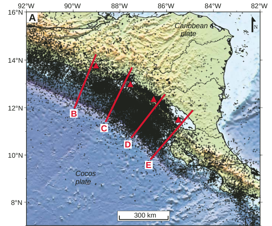
Figure 2. (A) Earthquake locations are from the National Earthquake Information Center (NEIC) and, in Nicaragua, were recorded by the local Nicaragua network from 1995 to 2003 operated by the Instituto Nicaraguense de Estudios Territoriales (INETER). (B–E) Earthquake profiles are perpendicular to the Middle America Trench (MAT) and extend to the interior volcanic highlands of Central America. These profiles merge all earthquakes within a 50-km-wide swath along each transect. Seismic activity beneath the volcanic front in Nicaragua is more evident because of more data from local stations of the Nicaraguan seismic network. These shallow crustal earthquakes commonly occur within the upper 30 km of the crust and are concentrated within ~25 km of the active Central America volcanic front (CAVF).
