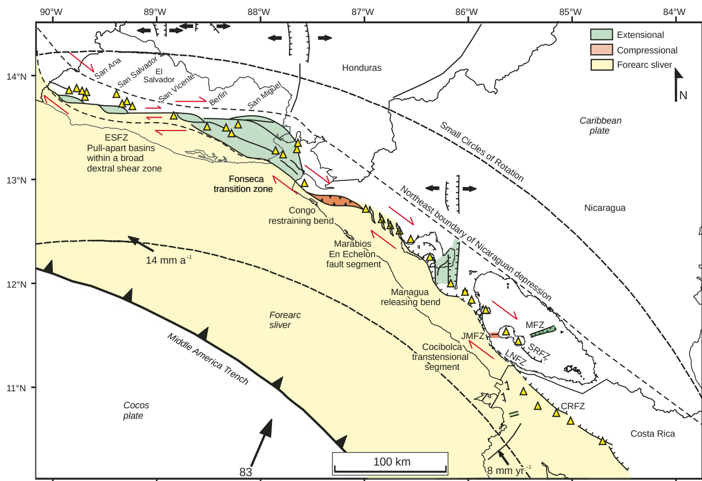
Figure 22. Regional tectonic map of Central America emphasizing key structures described in this paper. The El Salvador fault zone (ESFZ) is characterized by a broad right-lateral shear zone accommodating transtensional motion that results in multiple pull-apart basins. A major transition zone occurs in the Gulf of Fonseca, where strike-slip fault zones along the Central American forearc sliver change strike from dominantly east-west strikes in El Salvador to northwesterly strikes in Nicaragua. A proposed restraining bend connects faults mapped in the Gulf of Fonseca with fault scarps deforming Cosiguina volcano and faults of the Central America volcanic front north of Lake Managua. Diffuse and poorly exposed faults parallel to the Central America volcanic front in northern Nicaraguan segment are inferred to represent a young fault boundary in which right-lateral shear is accommodated over a broad zone. This model proposes a young en echelon pattern of strike-slip and secondary faults based on secondary extensional features and fissure eruptions along the Marabios segment of the Central America volcanic front. Lake Managua and the Managua graben are interpreted to occur at a major releasing bend in the trend of the Nicaraguan depression and are marked by the curving surface trace of the Mateare fault interpreted from aeromagnetic data. Subsequent right-lateral strike-slip motion related to translation of the Central America forearc sliver may occur along these reactivated normal faults. The Lake Nicaragua segment of the Central America volcanic front is bounded by a normal fault (LNFZ—Lake Nicaragua fault zone) offsetting the Rivas anticline, the southeastward continuation of this normal fault into Costa Rica (CNFZ—Costa Rica fault zone), and a synthetic normal fault (SRFZ—San Ramon fault zone) that we discovered in our survey of Lake Nicaragua. Transverse faults (MFZ—Morrito fault zone, JMFZ—Jesus Maria fault zone) strike approximately east-west across the Central America volcanic front. North-south-trending rift zones are abundant in El Salvador but less common in Nicaragua and may also be controlled by regional east-west extension affecting the northwestern corner of the Caribbean plate.
