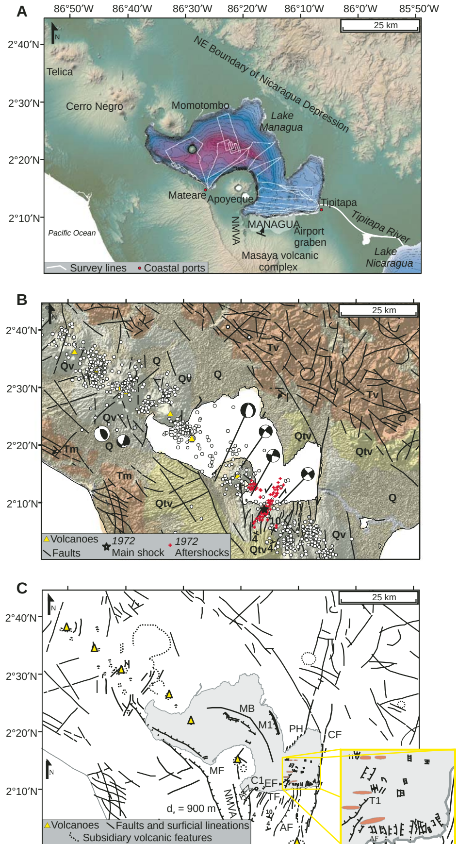
Figure 13. (A) Shuttle Radar Topography Mission imagery of Lake Managua and the Central America volcanic front in northern Nicaragua. Bathymetric data set was created from Nicaraguan Hydrographic Department of the Instituto Nicaraguense de Estudios Territoriales (INETER, 1979) and new bathymetric data collected during this survey using a subbottom profiler. (B) Geologic map from Case and Holcombe (1980) and Cowan et al. (2002) overlain on topography. Shallow earthquakes less than 33 km depth (white circles) are from the local Nicaragua seismic network operated by INETER from 1995 to 2003 and focal mechanisms are from the Harvard Centroid Moment Tensor (CMT) catalog, indicating a concentrated seismic belt along the Central America volcanic front. Aftershocks calculated from the 1972 ( M = 6.2 ) Managua earthquake occurred along the left-lateral northeast-striking slip-plane of the Tiscapa fault (TF) and the parallel, left-lateral Estadio fault (EF). (C) Interpretation from the 2006 NicLakes survey of Lake Managua based on 38 lines of 3.5 kHz subbottom profiler and sidescan sonar, and four multi-channel seismic-reflection lines. The inset is a close-up view near the southern shores showing intense faulting within the Airport graben and faults terminating against the Airport graben, including the fault labeled T1. These lines show several faults scarps on the lake bottom with vertical throws on the order of 1–7 m and an unknown component of horizontal offset. Red shading shows areas of seismic penetration that lack a prominent multiple reflector. The main results from the southern part of Lake Managua suggest that northeast-southwest-striking faults are bound to the west by the Nejapa-Miraflores volcanic alignment (NMVA) and to the east by the north-south-striking faults of the Airport graben. AF—Aeropuerto fault, CF—Cofradía fault, PH—Puente Huete fault, MF—Mateare fault, MB—Momotombito fault, AFZ—Asososco-Acahualinca fault zone.
