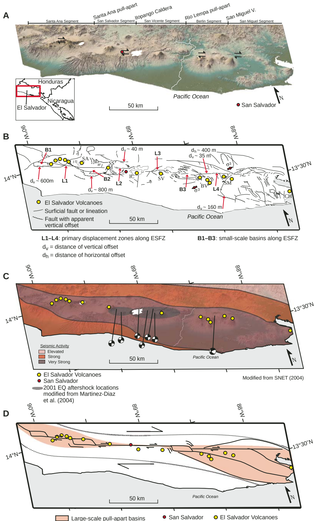
Figure 8. (A) Oblique view on Shuttle Radar Topography Mission topographic map of the El Salvador fault zone (ESFZ) extending from the Gulf of Fonseca to the western border of El Salvador. (B) Interpretation of the El Salvador fault zone based on the SRTM topography and satellite images from LANDSAT and Google Earth. SA—Santa Ana volcano, SS—San Salvador volcano, SV—San Vicente volcano, BV—Berlin volcano, SM—San Miguel volcano, CH—Chochagua volcano, IC—Ilopango caldera. (C) Map from Servicio Nacional de Estudios Territoriales SNET (2004) displaying the distribution of seismicity across El Salvador. Focal mechanisms are from the Harvard Centroid Moment Tensor (CMT) catalog for all events from 1976 to 2007. The main aftershocks from the February 2001 San Salvador earthquake occurred primarily along the San Salvador and San Vicente segments of the El Salvador fault zone (Martinez-Diaz et al., 2004). (D) Proposed transtensional pull-apart model from this paper. Two main deformation zones are characterized by large-scale pull-apart basins along a straight right-lateral strike-slip fault passing through Ilopango caldera. Within the large pull-apart basins, there are several smaller-scale pull-apart basins. Late Quaternary volcanic deposits likely obscure many recent faults.
