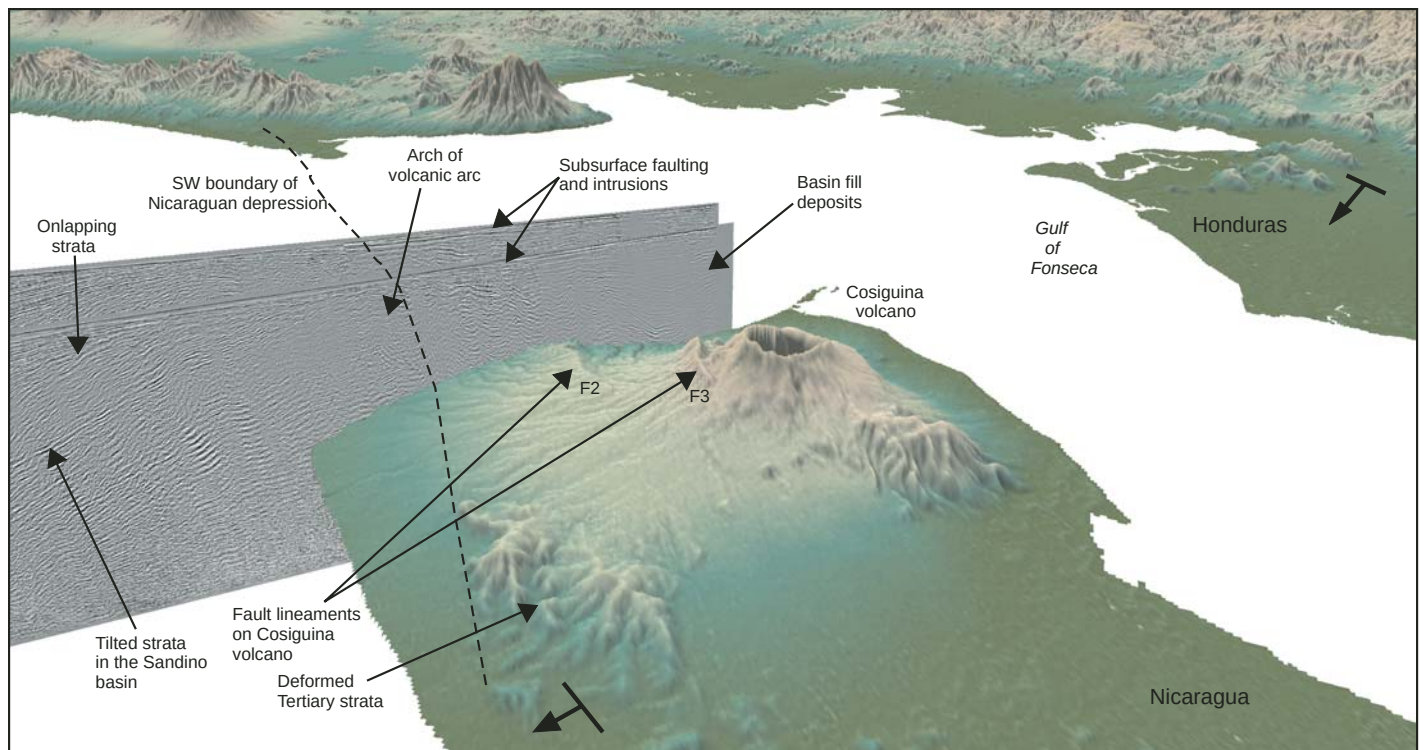
Figure 10. Oblique view of the Gulf of Fonseca displaying Shuttle Radar Topography Mission imagery and multichannel seismic-reflection profiles. Seismic-reflection lines in the offshore Sandino basin exhibit onlapping strata indicating an uplift event of pre-Miocene age (Stephens et al., 2007). Locally uplifted onland strata southwest of Cosiguina volcano are indicative of restraining bend deformation along a curving strike-slip segment as shown schematically on the inset in Figure 9B. Several fault lineaments (F2 and F3) trend from the inferred restraining bend area into Cosiguina volcano; these faults produce scarps with significant vertical throws that affect drainages on the flanks of the volcanic edifice. The fault lineaments project into the Gulf of Fonseca and correlate with several linear bathymetric highs along with faults and intrusive features seen on seismic profiles.
