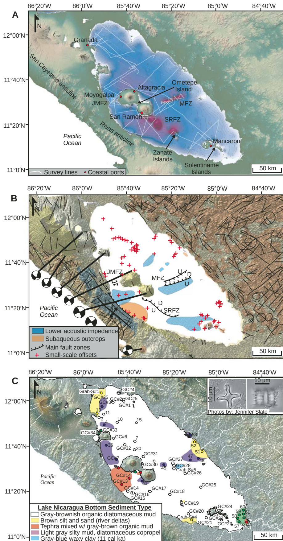
Figure 17. (A) The Shuttle Radar Topography Mission topographic image shows Lake Nicaragua bounded to the west by uplifted rocks of the Pacific coast and to the east by the interior Nicaragua Highlands. (B) Map showing geology and structure compiled by Case and Holcombe (1980) and Instituto Nicaraguense de Estudios Territoriales (INETER) with focal mechanisms from the Harvard Centroid Moment Tensor (CMT) catalog. Three main faults zones (Jesus Maria—JMFZ, Morrito—MFZ, San Ramon—SRFZ) were discovered beneath the lake, along with numerous uncorrelatable small-scale faults. (C) Bottom sediment map is compiled from 35 sediment cores collected during the NicLakes survey (Wulf et al., 2007). Bottom sediment type distribution suggests the majority of the lake bottom consists of a homogeneous, diatomaceous mud as shown in the inset (diatom photos in inset are courtesy of Jennifer Slate, North-eastern Illinois University).
