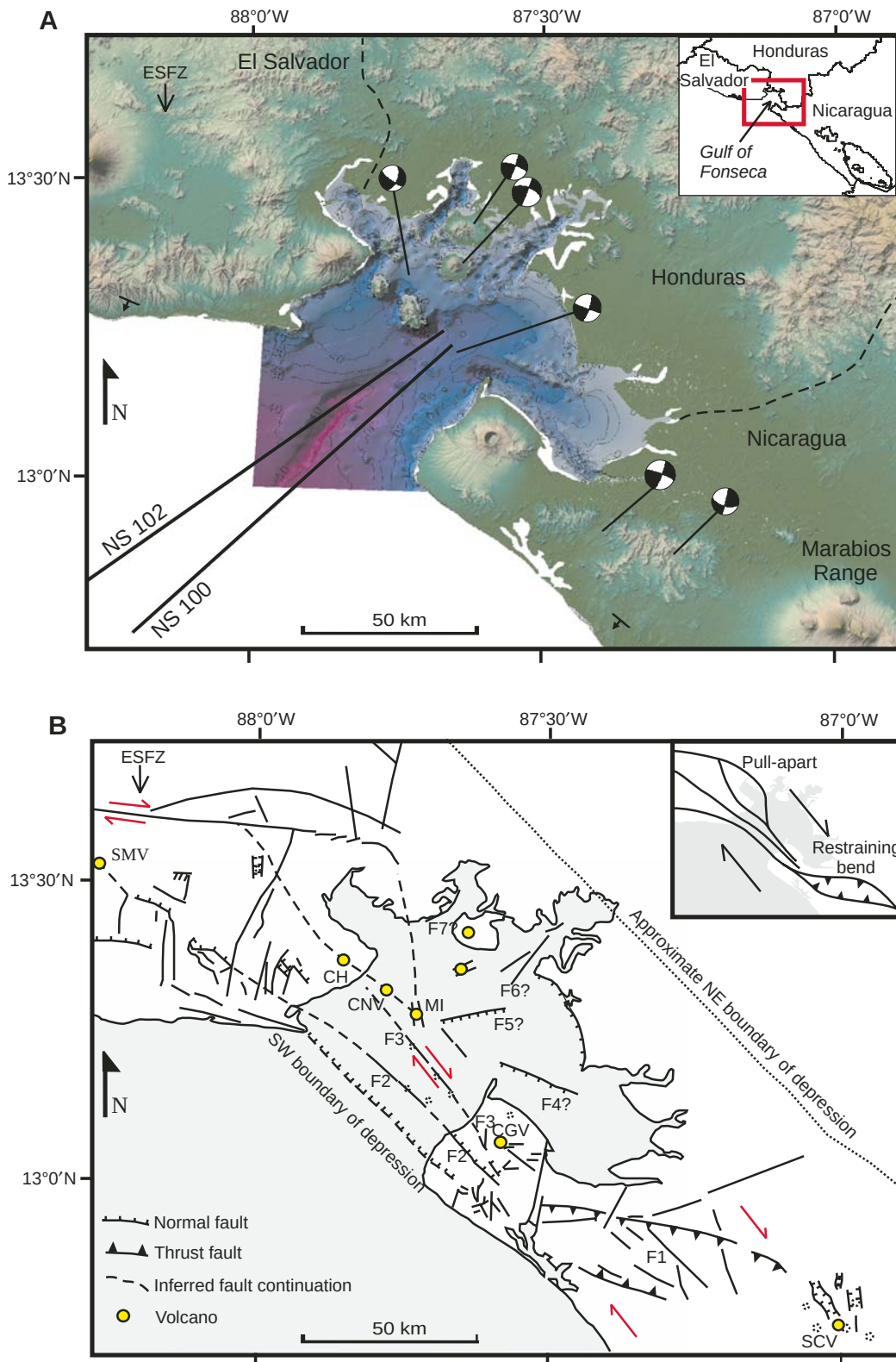
Figure 9. (A) Gulf of Fonseca showing focal mechanisms from the Harvard Centroid Moment Tensor (CMT) catalog, Shuttle Radar Topography Mission imagery, and bathymetry digitized from the Defense Mapping Agency Hydrographic Topographic Center (1996, scale 1:5000). Subsurface geology was integrated using two multi-channel seismic-reflection lines collected during the EW0412 NicStrat cruise by McIntosh and Fulthorpe (2005). (B) Structural interpretation based on Case and Holcombe (1980), SRTM and Landsat images, and subsurface faults mapped on reflection lines NS102 and NS100 (Figs. 11 and 12). F1 represents a large restraining bend as the forearc sliver boundary curves from Cosiguina volcano (CGV) to the Marabios Range, beginning with San Cristobal volcano (SCV). F2 and F3 are two large faults with significant vertical offsets on late Quaternary deposits of the Cosiguina volcano; both faults project into the Gulf of Fonseca near Meanguero Island (MI), Conchaquito volcano (CNV), and Chochagua volcano (CH). Both faults align with linear highs on bathymetric maps and subsurface faults seen on seismic-reflection lines. F4–F7 are lineaments in the Gulf of Fonseca that we interpret as either faults or fluvial channels incised during lowstands of sea level. The inset map shows a tectonic interpretation for the Gulf of Fonseca area where the proposed forearc sliver boundary changes its strike between faults of the Median Trough in El Salvador and faults of the Nicaraguan depression in northern Nicaragua. ESFZ—El Salvador fault zone, SMV—San Miguel volcano.
