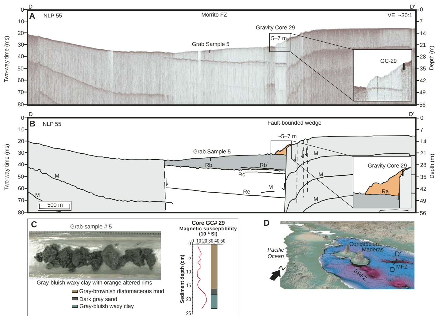
Figure 20. (A) Uninterpreted 3.5 kHz subbottom profiler line NLP55 crossing the Morrito fault zone of Lake Nicaragua. This linear depression trends approximately N75°E, exhibits 12–15 m of vertical offset, is not traceable westward to Maderas volcano, and shallows significantly to the east. VE—vertical exaggeration. (B) Interpreted 3.5 kHz subbottom profiler line NLP55. The southern margin of this fault zone appears to be covered by a clastic wedge that provides evidence for the age of active faulting; reflectors Ra–Re are the only subsurface layers imaged beneath the lake. (C) Several cores and grab samples were also taken across this profile. These cores show gray-blue waxy clay just below the surface of the upthrown block, through the clastic wedge, dated at 11,271–11,403 cal ^{14}\text{C} yr B.P. The same clay found in grab sample #5 constrains the age of fault activity and shows an average vertical slip rate of 73 cm per 1000 yr (Wulf et al., 2007). This same clay is found in a grab sample near the center of the Morrito fault zone trough, suggesting 12–15 m of vertical displacement throughout the Holocene. (D) Oblique view of Lake Nicaragua showing cross-section location. MFZ—Morrito fault zone, SRFZ—San Ramon fault zone.
