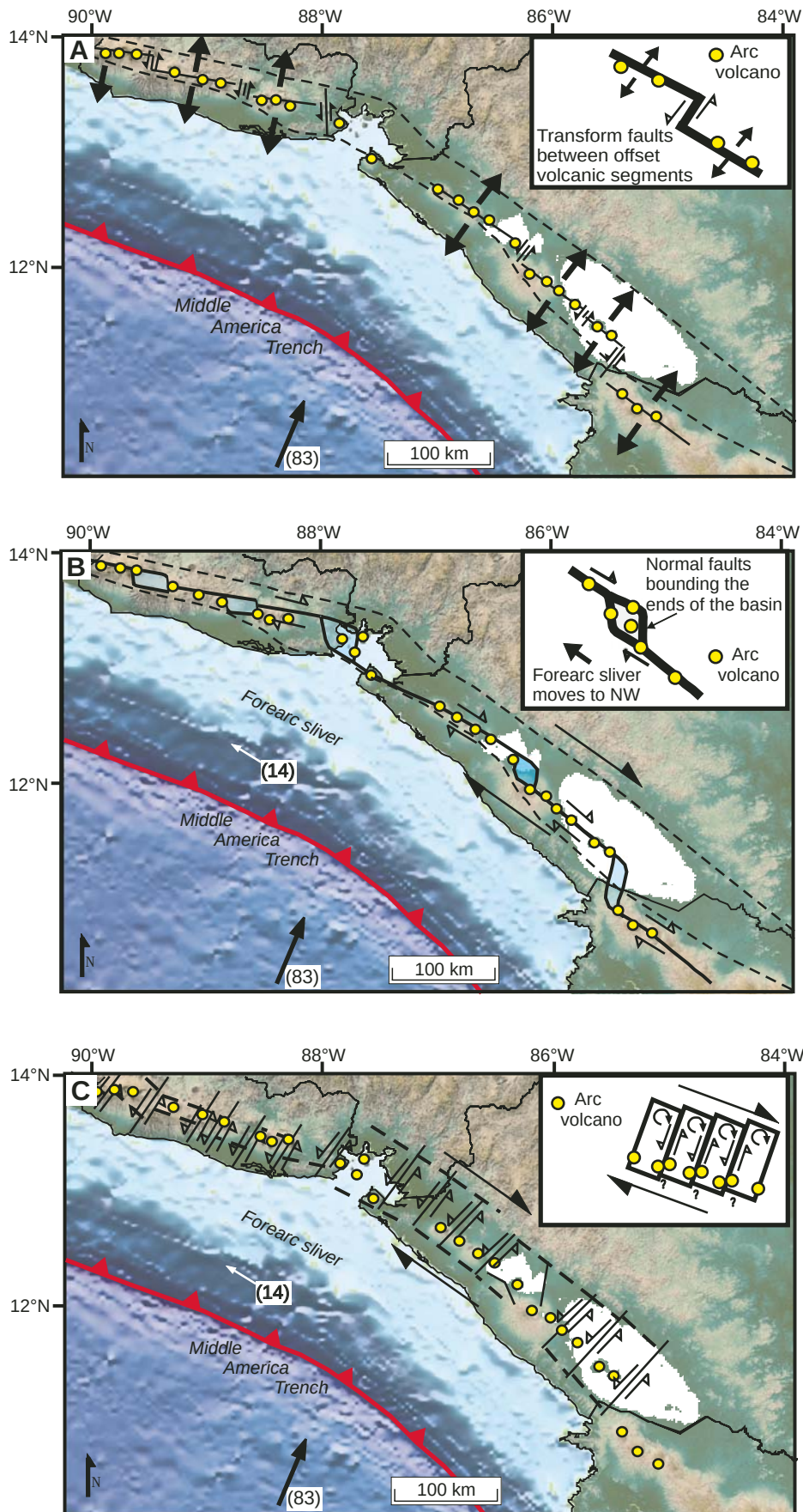
Figure 7. Previous tectonic models for the Nicaraguan depression: (A) The transform fault model was first proposed by Dewey and Algermissen (1974) to explain the segmented offsets of the Central America volcanic front by ridge-ridge transform faults. (B) The pull-apart model suggests northwestward transport of the Central America forearc sliver, which detaches from the western Caribbean plate due to right-lateral shear concentrated along the thermally weakened Central America volcanic front. Extension becomes localized at fault stepovers, resulting in pull-apart structures. (C) The bookshelf faulting model suggested by La Femina et al. (2002) explains right-lateral transport of the Central America forearc sliver by a series of rotating crustal blocks bounded by parallel, left-lateral faults.
