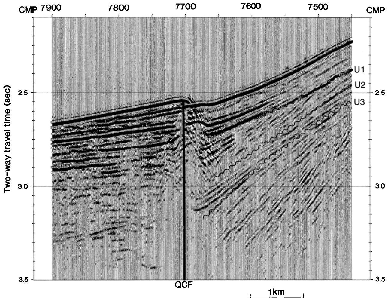
Figure 10. Detail of line 1262 migrated, no amplitude scaling. Sediments on the Pacific plate are subhorizontal, whereas sediments on the North American plate dip up to 20° and contain several unconformities. Wavy lines indicate unconformities.
