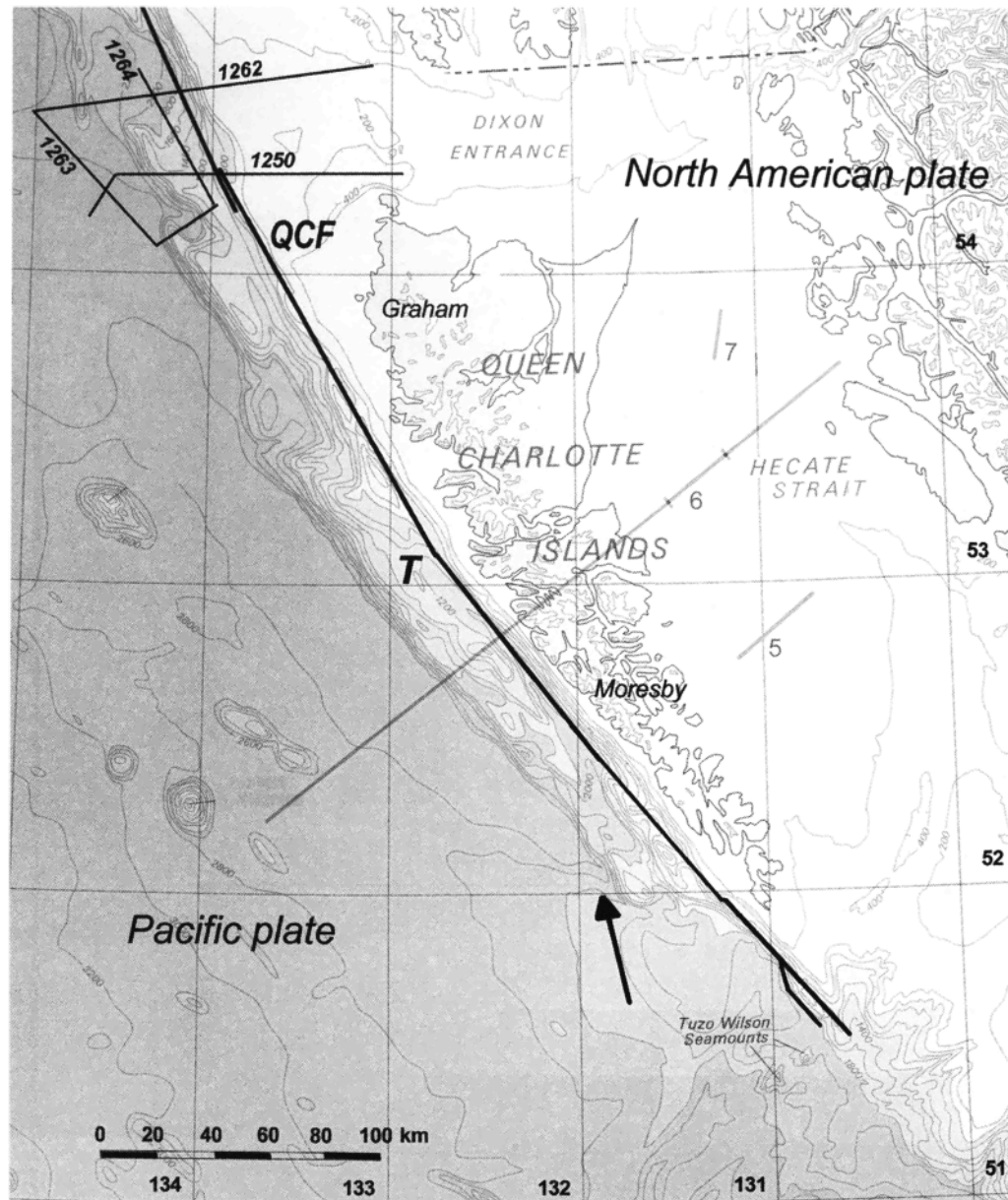
Figure 3. Regional morphology with location of new multichannel seismic reflection data: lines 1250, 1262, 1263, and 1264. T is the Queen Charlotte terrace. Arrow shows direction of relative plate motion calculated from NUVEL-1 [DeMets et al. , 1990]. Location of QCF was picked from GLORIA data (Figure 2). Light shaded line is location of cross section shown in Figure 4. Short line segments show locations of multichannel seismic reflection lines 5, 6, and 7 displayed in Figure 6.
