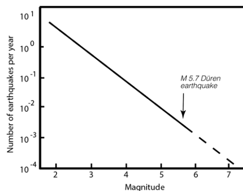
Fig. 6. Earthquake frequency–magnitude data for the Lower Rhine Embayment (Vanneste et al. 2013). Reproduced with permission of the Royal Astronomical Society.
