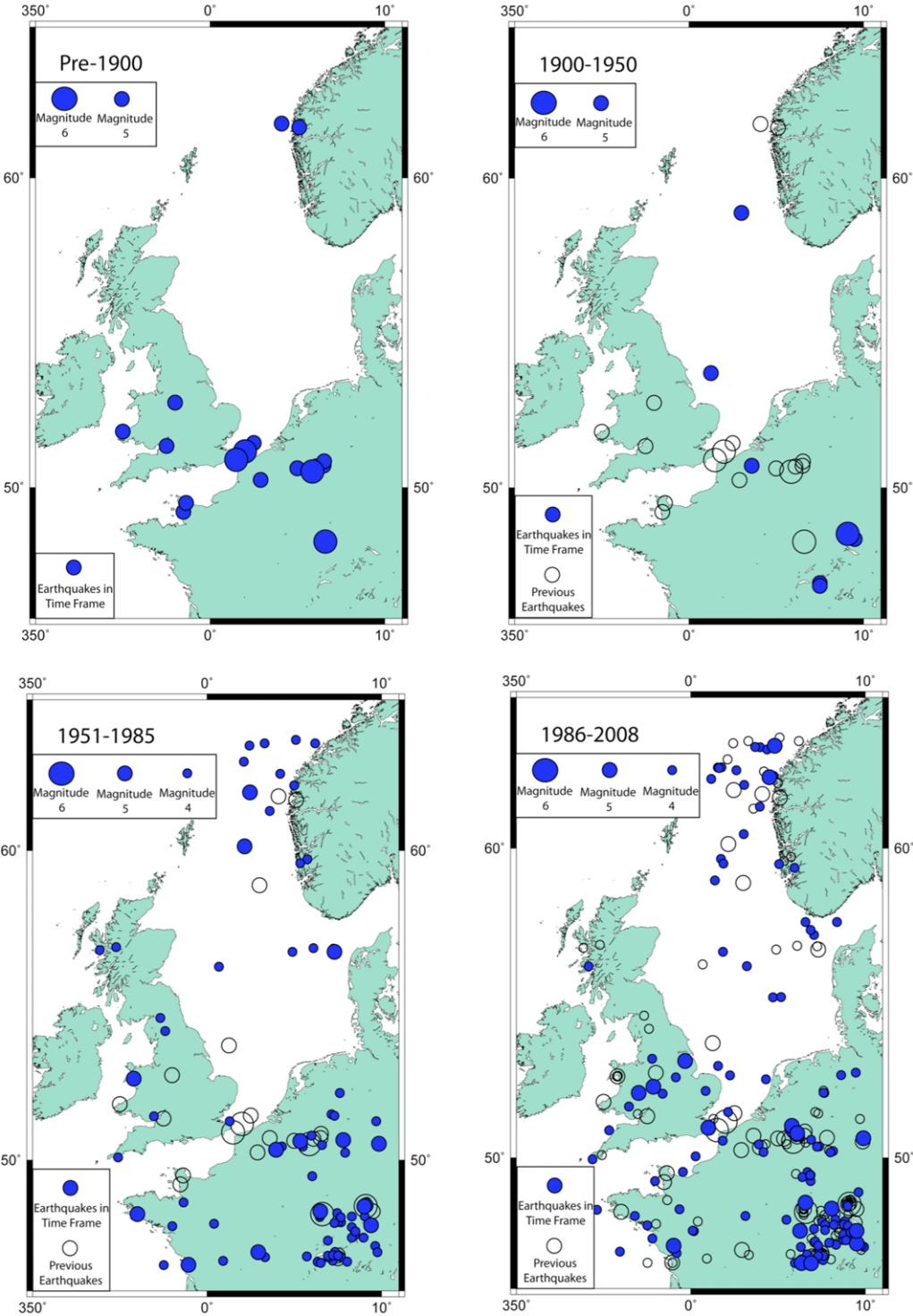
Fig. 7. Seismicity of the Lower Rhine Embayment for different periods (taken from Royal Observatory of Belgium catalogue; Kusters 2014).
