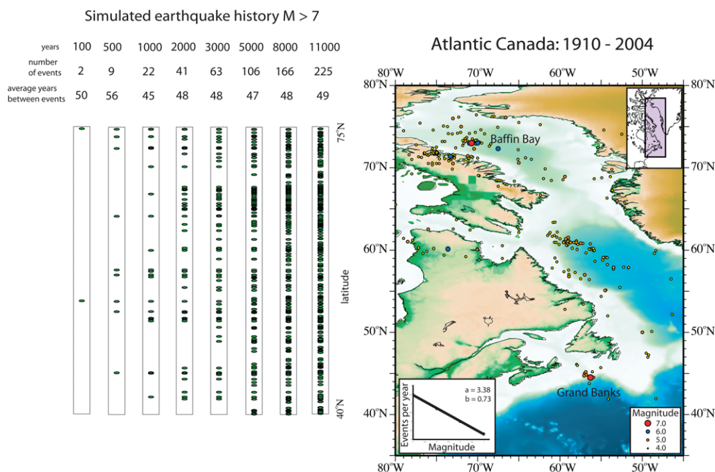
Fig. 9. Intraplate seismicity along the eastern coast of Canada. Simulations using a frequency–magnitude relation derived from these data predict that if seismicity is uniform in the zone, about 11 000 years of record is needed to avoid apparent concentrations and gaps (Swafford & Stein 2007). Reproduced with permission of Geological Society of America.
