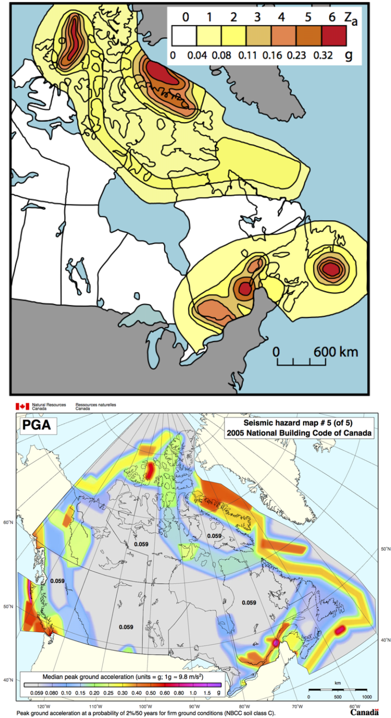
Fig. 13. Comparison of the 1985 and 2005 earthquake hazard maps of Canada (Stein et al. 2012). Reproduced with permission of Elsevier B. V.
