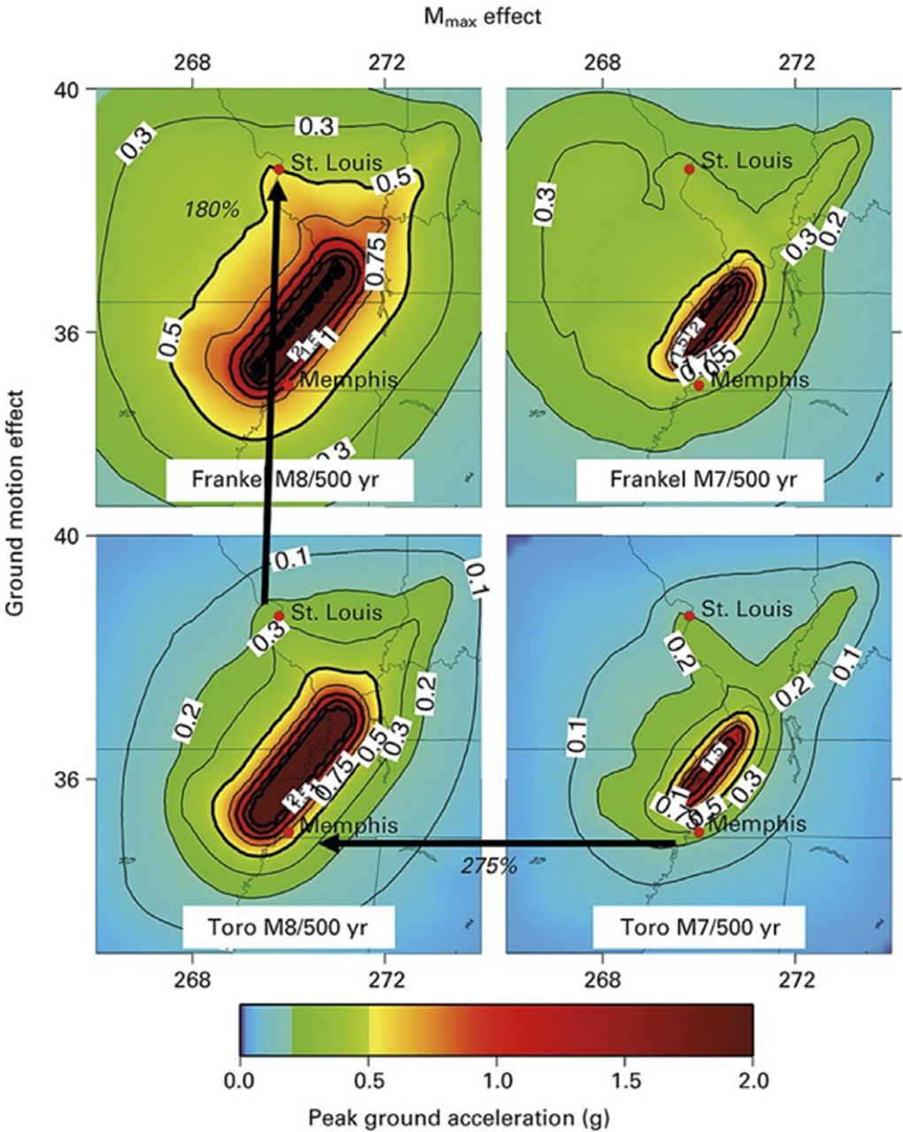
Fig. 14. Comparison of different hazard maps (2% probability in 50 years) for the New Madrid seismic zone (Newman et al. 2001).
