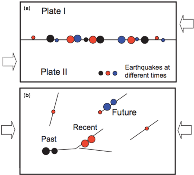
Fig. 11. Cartoon showing the difference between earthquakes (a) at plate boundary faults and (b) in mid-continents (Liu et al. 2011). Reproduced with permission of Geological Society of America.
