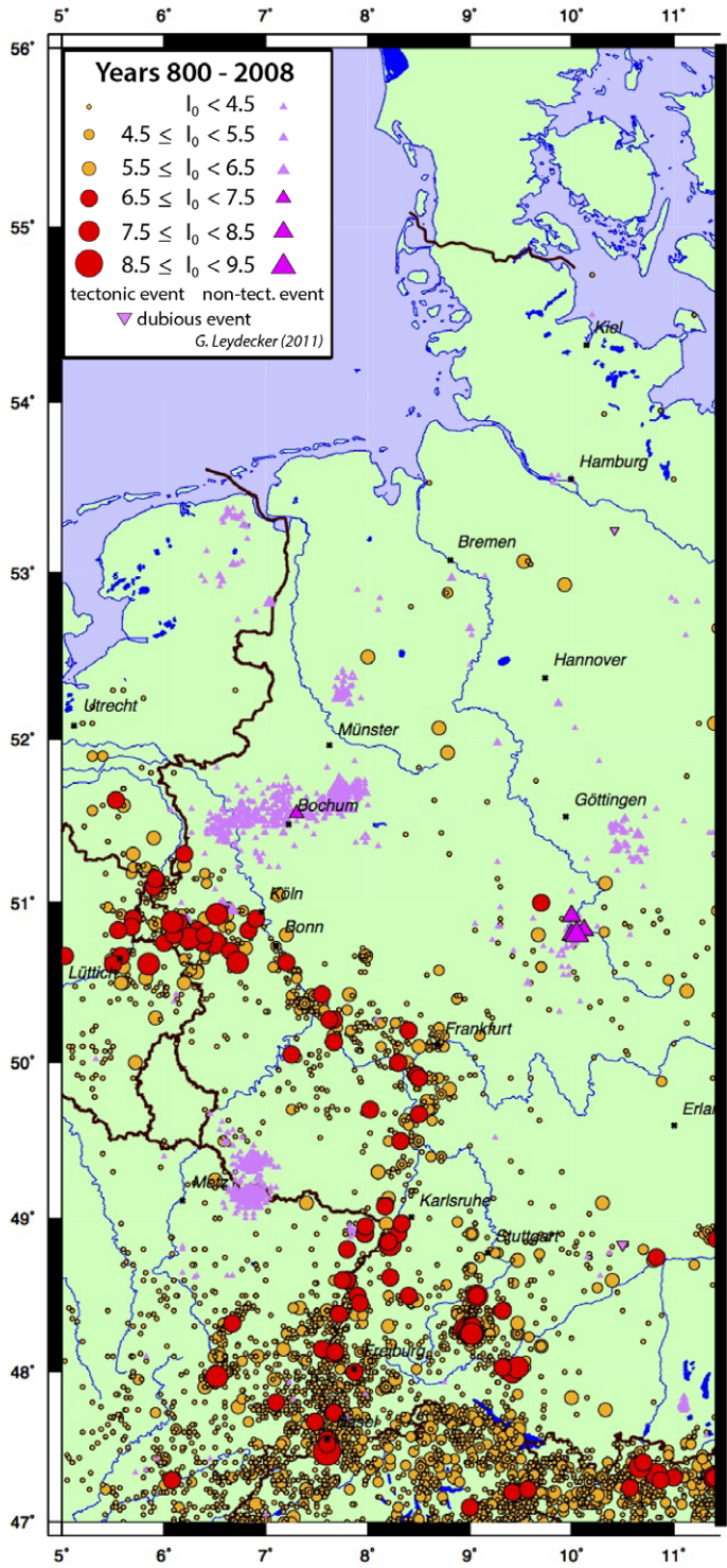
Fig. 8. Historical seismicity of the region shown by earthquakes with different epicentral intensities from 800 AD (Leydecker 2011). Reproduced with permission of Bundesanstalt für Geowissenschaften und Rohstoffe (BGR).
