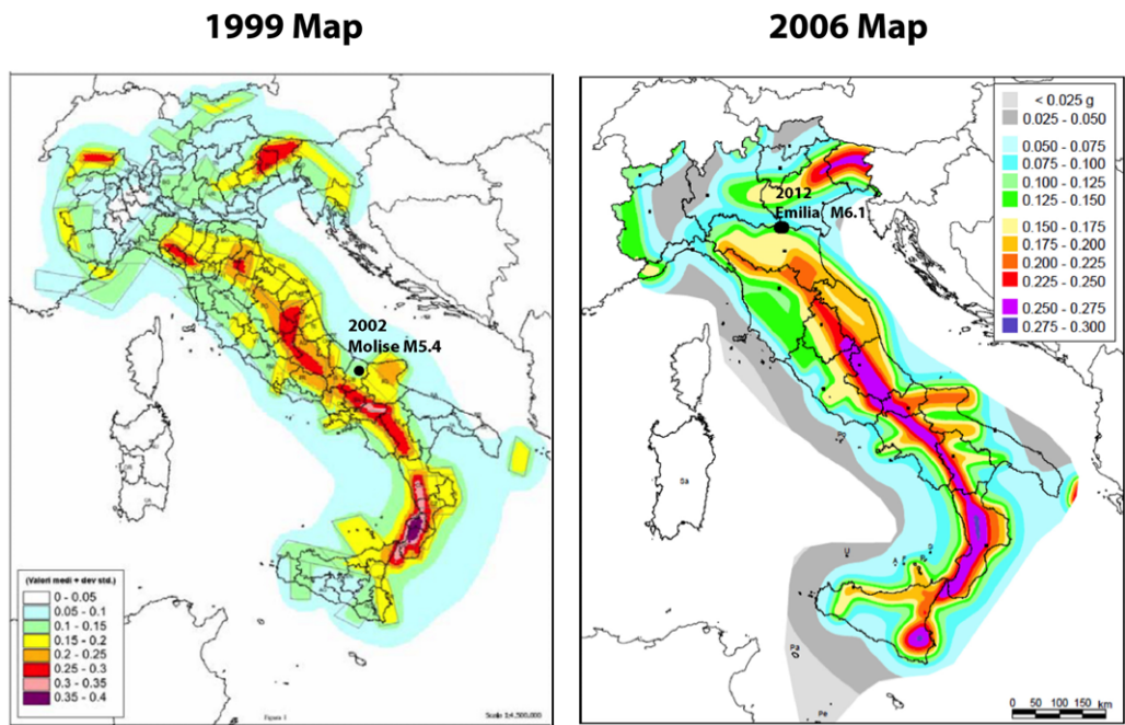
Fig. 2. Comparison of successive Italian hazard maps (Stein et al. 2015a), which forecast some earthquake locations well and others poorly. The 1999 map was updated to reflect the 2002 Molise earthquake and the 2006 map will probably be updated after the 2012 Emilia earthquake. Reproduced with permission of the Seismological Society of America.
