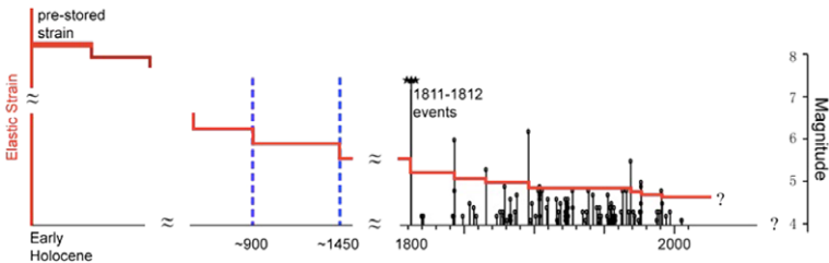
Fig. 12. Conceptual model of a decaying New Madrid seismic zone earthquake sequence showing large earthquakes during 1811–1812 and similar events around 900 and 1450, and smaller events since 1812 (Liu et al. 2014). Reproduced with permission of Springer.
