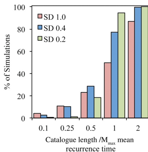
Fig. 10. Numerical simulations assessing how well earthquake catalogues of different lengths recover the actual maximum magnitude M_{\max} of earthquakes in an area. Catalogue lengths are given as a fraction of the mean recurrence time for earthquakes with magnitude M_{\max} . Colours show results for Gaussian distributions of recurrence times with standard deviation equal to the indicated fraction of the mean. The largest earthquake observed probably reflects the length of the history used, even if larger earthquakes occur, so a catalogue shorter than an earthquake’s mean recurrence time is likely to not contain an event of that size (Stein & Friedrich 2014; Merino 2014). Reproduced with permission of the Royal Astronomical Society.
