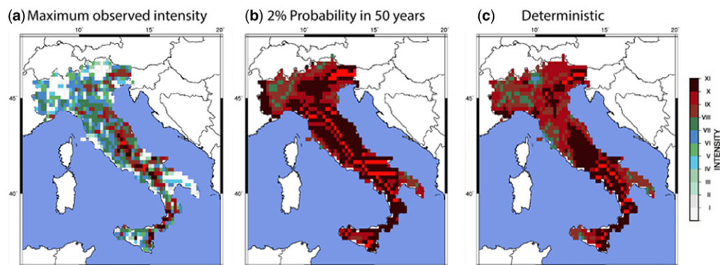
Fig. 4. Comparison of (a) historical intensity data for Italy with (b) probabilistic and (c) deterministic hazard maps, both of which over-predict the observed shaking (Stein et al. 2015a). Reproduced with permission of the Seismological Society of America.
