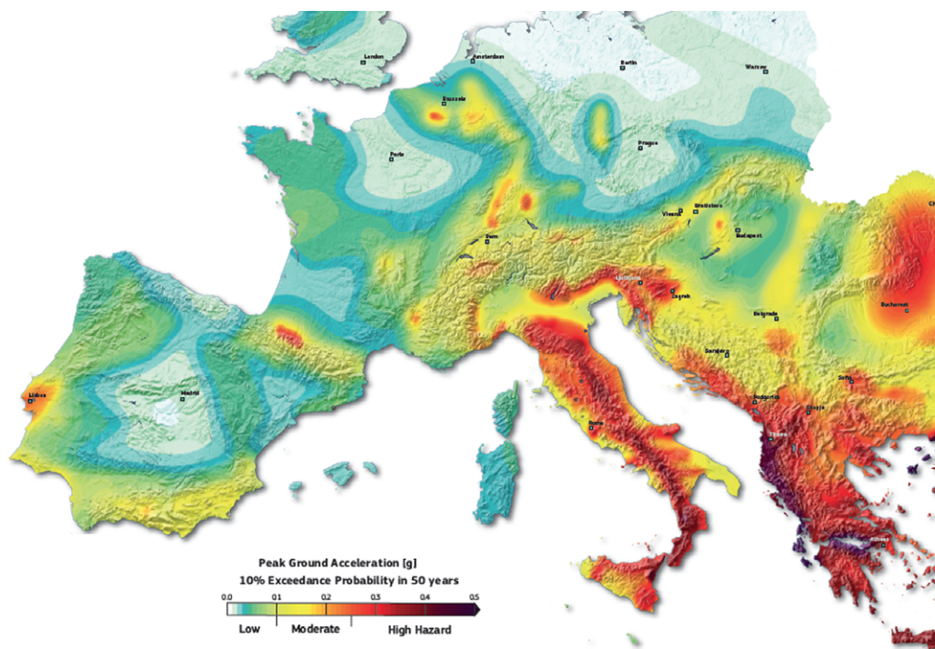
Fig. 1. Part of the 2013 SHARE earthquake hazard map (Giardini et al. 2013).
