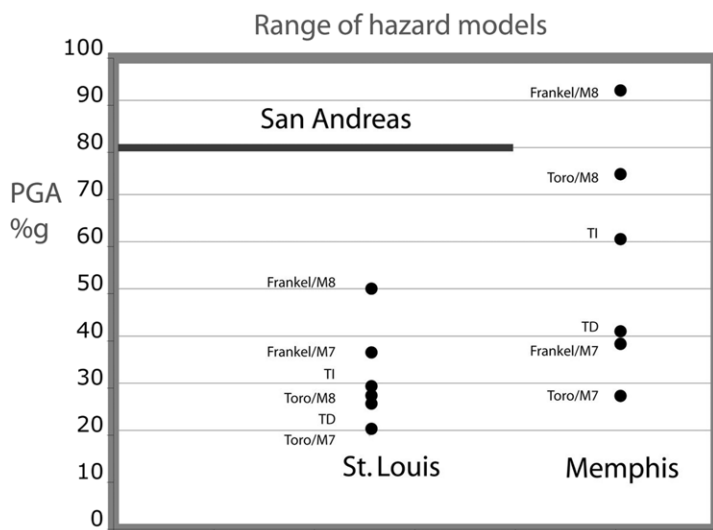
Fig. 15. Comparison of the hazard, described as peak ground acceleration (PGA) as a percentage of the acceleration of gravity expected with 2% risk in 50 yr, at St Louis and Memphis predicted by various hazard maps of the New Madrid zone, including those shown in Figure 14. For example, Frankel/M8 indicates the Frankel et al. (1996) ground motion model with a maximum magnitude of 8, and TI and TD indicate the difference between the time-independent and time-dependent models for a specific combination of maximum magnitude and ground motion model (Stein et al. 2012). Reproduced with permission of Elsevier B. V.
