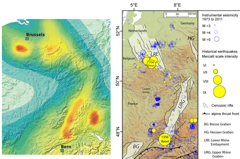
Fig. 5. Left: SHARE map section including the Upper Rhine Graben and Lower Rhine Embayment. Right: Historical seismicity of NW Europe (Kübler 2013).
