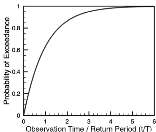
Fig. 3. Assumed probability p that during a t -year-long observation period, shaking at a site will exceed a value that is expected on average once in a T -year return period (Stein et al. 2015a). Reproduced with permission of the Seismological Society of America.
