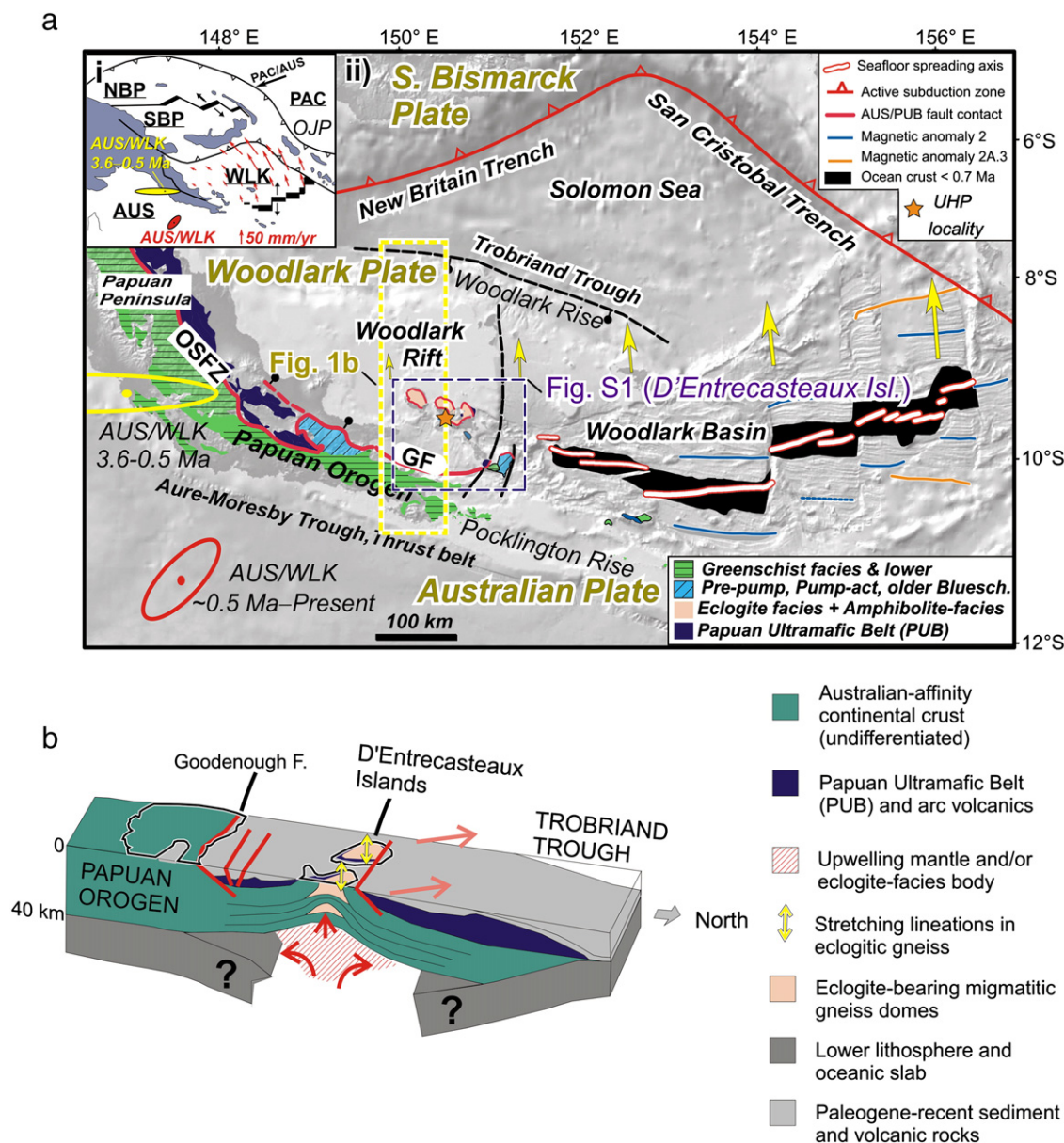
Fig. 1. Tectonic setting of the D'Entrecasteaux Islands and Woodlark Rift, Papua New Guinea. (a) Inset (i): contemporary plate tectonic map of eastern Papua New Guinea: NBP, North Bismarck Plate, SBP, South Bismarck Plate, WLK, Woodlark Plate, AUS, Australian Plate, PAC, Pacific Plate; OJP, Ontong-Java Plateau. Bold black arrow shows velocity of the Pacific Plate relative to the Australian Plate. Small red arrows depict velocities of the Woodlark Plate relative to the Australian Plate after Wallace et al. (2004). All velocity magnitudes are shown relative to 50 mm/yr key at bottom right of inset. (ii) Simplified tectonic map of southeastern Papua New Guinea modified after Webb et al. (2008), showing key tectonic features and distribution of metamorphic rocks. Background is shaded Digital Elevation Model from GeoMapApp ( http://www.GeoMapApp.org ). Geologic units are much simplified from Daczko et al. (2009) and Davies (1980b). Pre-pump = prehnite-pumpellyite facies; Pump-act = pumpellyite-actinolite facies. Pole of WLK-AUS rotation for 3.6-0.5 Ma (with error ellipse) from Taylor et al., 1999; GPS-derived pole of present-day WLK-AUS rotation from Wallace et al. (2004). Explanation: OSFZ, Owen Stanley fault zone; GF, Goodenough normal fault. Magnetic anomalies from Taylor et al. (1999). Yellow vectors indicate eastward increase in velocity associated with 3.6-0.5 Ma pole of rotation, used in this study. Yellow and blue dashed boxes outline areas shown in Fig. 1b and Supplementary Fig. S1, respectively. (b) Schematic block-model for present-day setting of D'Entrecasteaux Islands and Woodlark Basin tectonics, modified after Hill et al. (1995), Little et al. (2011), and Webb et al. (2008). Bold red lines: main active faults. Yellow double arrows: ductile stretching lineation directions in gneiss domes. Pink arrows: extension directions 3.6-0.5 Ma.
