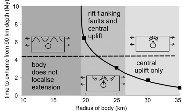
Fig. 6. Effect of subducted body dimensions on exhumation time and deformation style. Time for body to reach surface from 90 km depth, vs. initial size of circular body. Bodies below an initial radius of ca. 19 km do not localise extension and are not exhumed. Bodies with a radius of >26 km do not form initial rift-flanking faults, i.e. central uplift only (see schematised insets). Dashed horizontal line represents estimate of exhumation time from 2.4 GPa to surface from Baldwin et al. (2004).
