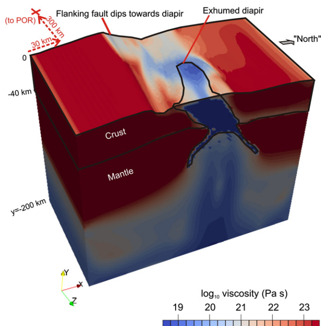
Fig. 7. Colour contours of \log_{10} (effective viscosity) for 3D model after 1.9 My extension. The model setup is shown in Fig. 2b. Eclogite-facies diapiric body outlined in bold black line. No vertical exaggeration.
