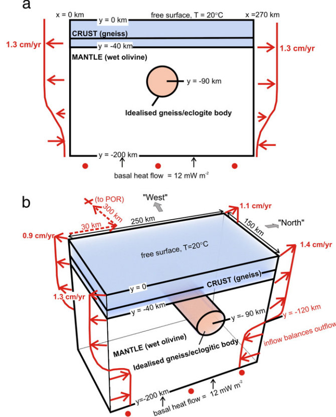
Fig. 2. Setup for the numerical models. (a) 2D model initial and boundary conditions. No vertical exaggeration. (b) 3D model initial and boundary conditions. Inflow velocity boundary conditions are prescribed to give zero net influx into model box. “to POR” means 300 km to the pole of rotation. For details of material properties, see Table 1 and Supplementary Note S1.
