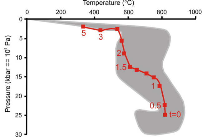
Fig. 5. Pressure-Temperature-time path for a tracer particle initially at x = 135 km, y = -90 km in the middle of the continental-affinity body (red line). Red numbers are time since exhumation started, in My. Pressure is computed as mean stress including dynamic stresses. For reference, smoothed P-T bounds for the retrograde path of exhumed rocks from Baldwin et al. (2004) are also shown (grey shading), where the estimated exhumation time (2.4 GPa to surface) was 4.3 My.
