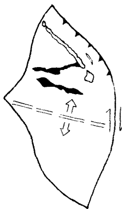
Fig. 2. Basin shape of the Philippine Sea at -17 Ma (a), -30 Ma (b), -42 Ma (c) and -48 Ma (d). Volcanic arcs are spotted and remnant arcs are filled.
