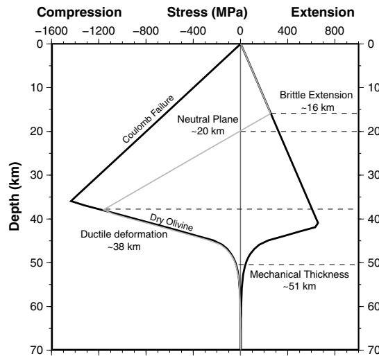
Figure 9. Yield Stress Envelope (YSE) corresponding to the distance of maximum bending moment for the best fitting flexure model in Southern Mariana. X axis gives stress values (MPa), compression (negative) to left of the origin and tension (positive) to right of the origin. Y axis is depth (km) beneath the top of the plate. Black lines outline failure envelope. Coulomb failure criteria (compression, left; tension, right) extends from the origin to depths of ~40–45 km. Ductile deformation controls deformation to depth of the mechanical thickness ~50 km. Thin gray line shows the 0 MPa trend line and the thick gray line shows the change in stress within the bending plate with depth. Dashed gray lines show depths at which the plate stress switches from brittle failure to elastic core, the neutral plane, the depth where plate stress switches from elastic to ductile deformation, and the mechanical thickness depth.
