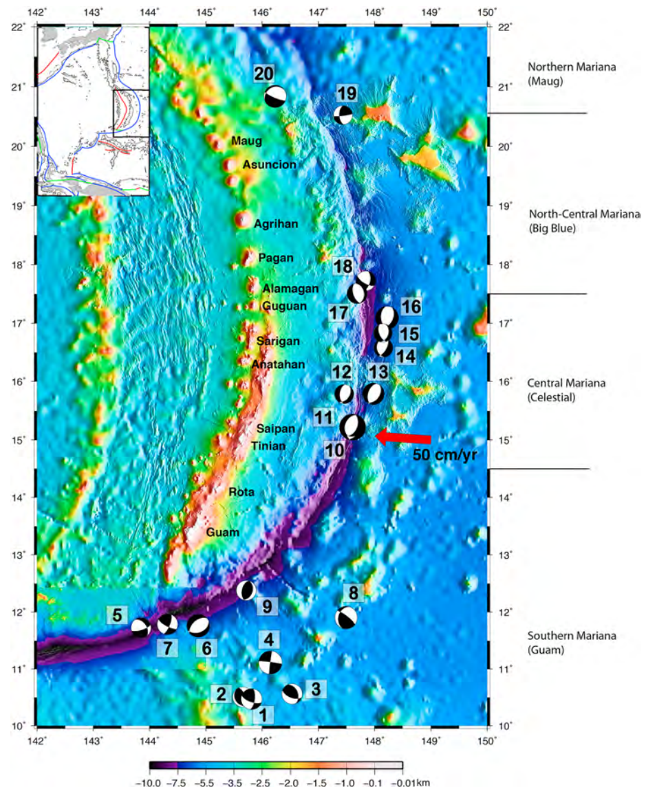
Figure 1. Relocated GCMT earthquakes in map view. Lower hemisphere stereographic projections for earthquakes are shown with compressional P wave quadrants (containing the T axis in black) and dilatational P wave quadrants (containing the P axis in white). The event numbers next to each focal mechanism correspond to Tables 2 and 4. The red arrow shows the angle of convergence of the Pacific plate relative to the Mariana fore arc as determined by Kato et al. [2003]. High-resolution bathymetry data in Northern and Central Mariana are from 2010 Mariana Law of the Sea Cruise [Gardner, 2010] and high-resolution bathymetry data in Southern Mariana are courtesy of F. Martinez. The color scale for bathymetry is positioned below and is the same for all bathymetric maps in the paper. (inset) Tectonic setting of the Philippine Sea. Bathymetry contours are shown by thin black lines. Subduction trenches are shown in blue; spreading centers are shown in red; transforms are shown in green.
