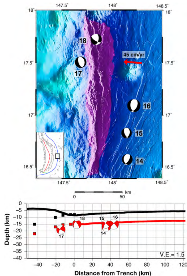
Figure 4. (top) Relocated GCMT earthquake locations in mapview. Lower hemisphere stereographic projections for earthquakes are shown with compressional quadrants (in black) and dilatational quadrants (in white). Event numbers next to each focal mechanism correspond to Tables 2 and 4. The red arrow shows the angle and rate of Pacific plate convergence relative to the fore arc as determined by Kato et al. [2003]. High-resolution bathymetry data are from Gardner [2010]. The bathymetry scale is the same as in Figure 1. Inset shows the tectonic setting of the Mariana Islands. Bathymetry contours are shown by thin black lines. The trench axis is shown in blue; back-arc spreading center is in red; transform is in green. (bottom) Trench-perpendicular cross section with the location of the subduction trench at 0 km; negative distances indicate the distance landward (or west of the trench) and positive distances indicate seaward distances (or east of the trench). Thick black lines show the bathymetry along (17.25°N, 147.3577°E) to (17.2752°N, 148.9311°E). Thick red lines show depth to the Moho used in our waveform inversion. Black squares show the depth to the plate interface at ~17°N from Oakley et al. [2008]; red squares indicate the continuation of the Moho landward from the trench. Focal mechanisms for the region are rotated 90° into cross section. Dilatational quadrants are indicated by white while compressional quadrants are indicated by red. The event numbers next to each focal mechanism correspond to Tables 2 and 4. Vertical exaggeration (VE) is 1.5.
