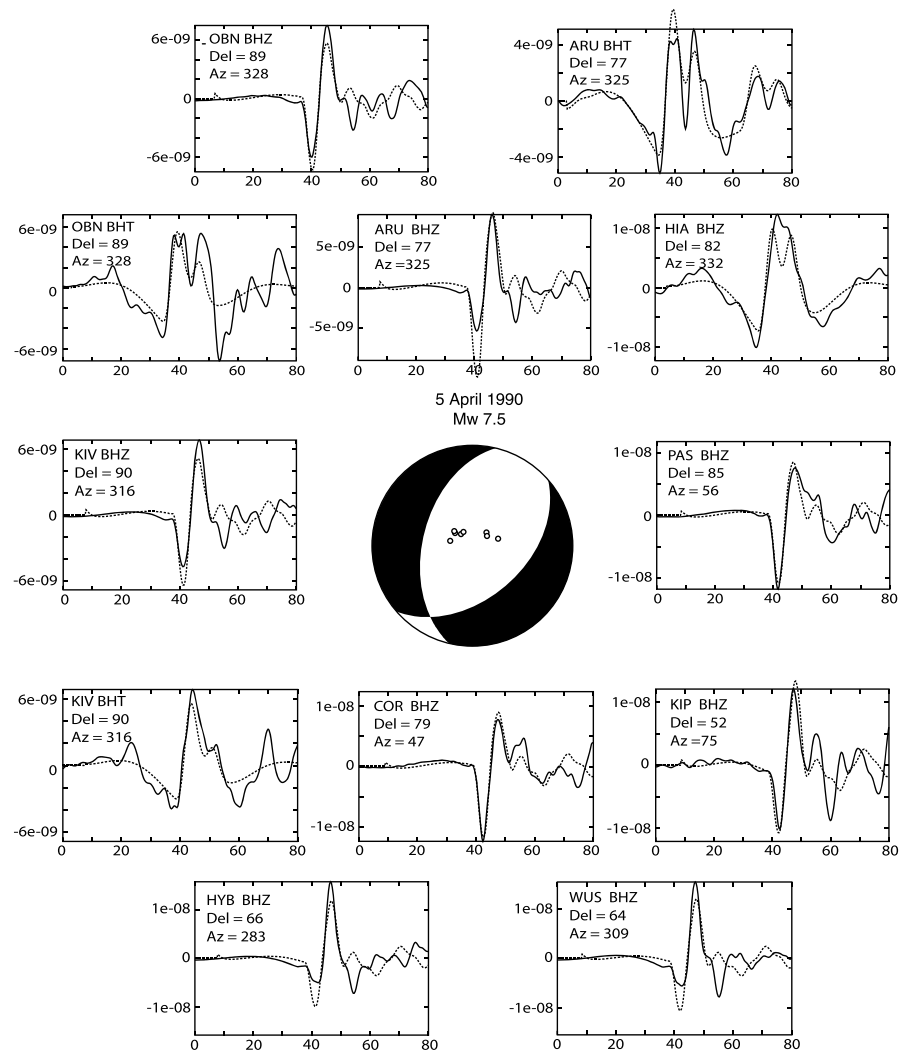
Figure 2. The best fit focal mechanism for the 5 April 1990 earthquake at 18 km depth in the Pacific plate. First-motion polarities for P wave arrivals are indicated by open circles (dilatation) and closed circles (compression). Select waveform data (BHZ and BHT) are shown as thick black lines and best fit synthetic waveforms are shown as dashed black lines. The x axis (time) is given in seconds and the y axis (displacement amplitude) is in meters. Distance (Del) and azimuth (Az) are in degrees.
