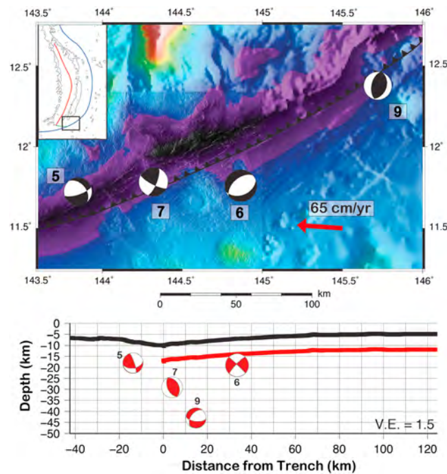
Figure 7. (top) Relocated GCMT earthquake locations from the Southern Mariana Trench in map view. Lower hemisphere stereographic projections for earthquakes have compressional quadrants (in black) and dilatational quadrants (in white). Event numbers next to focal mechanism correspond to Tables 2 and 4. Red arrow shows the angle and rate of Pacific plate convergence relative to the fore arc from Kato et al. [2003]. High-resolution bathymetry data are courtesy of F. Martinez. The bathymetry scale is the same as in Figure 1. Inset shows the tectonic setting of the Mariana Islands. Bathymetry contours are thin black lines. The subduction trench shown as a blue line; back-arc spreading center, red; transform boundary, green. (bottom) Trench-perpendicular cross section with the location of the subduction trench at 0 km; negative distances indicate the distance landward (or northwest of the trench) and positive distances indicate seaward distances (or southeast of the trench). Thick black lines show the bathymetry along (12.4708°N, 144.7513°E) to (11.1262°N, 145.4304°E). Thick red lines show depth to the Moho used in our waveform inversion. Black squares show the depth to the plate interface at ~17°N from Oakley et al. [2008]; red squares indicate the continuation of the Moho landward from the trench. Focal mechanisms for the region are rotated 90° into cross section. Dilatational quadrants are indicated by white while compressional quadrants are indicated by red. The event numbers next to each focal mechanism correspond to Tables 2 and 4. Vertical exaggeration (VE) is 1.5.
