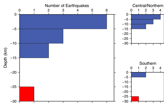
Figure 11. Distribution of earthquakes at Central/Northern Mariana with depth. (left) Depth and number of all events within the incoming Pacific plate mantle at the Mariana subduction zone. Blue bars are extensional earthquakes and red bars are compressional earthquakes. Depth is given as kilometers below the Moho. (top right) Central Mariana earthquakes. (bottom right) Southern Mariana.
