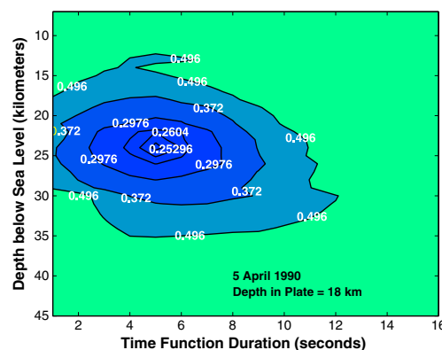
Figure 3. Misfit contours in depth versus source time function parameter space for 5 April 1990 large, extensional outer rise earthquake (Event 10, Table 2). Misfit is calculated using equations (1) and (2). Contours for the solutions at 2%, 5%, 10%, 20%, and 50% greater than the best fit solution are given. The y axis shows depth (kilometers) below sea level. The x axis represents the source time function (seconds).
