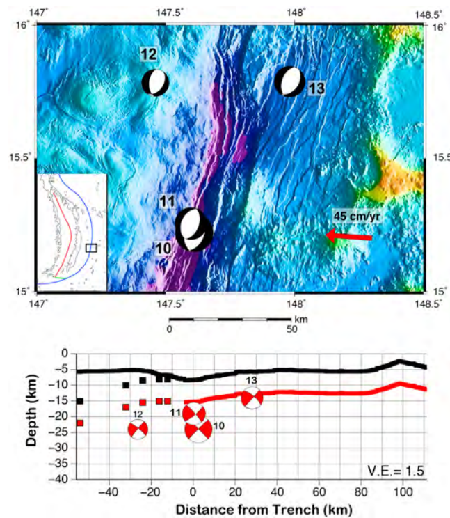
Figure 5. (top) Relocated GCMT earthquake locations in map view. Lower hemisphere stereographic projections are shown with compressional quadrants (in black) and dilatational quadrants (in white). Event numbers next to each focal mechanism correspond to Tables 2 and 4. The red arrow shows the angle of convergence of the Pacific plate relative to the Mariana fore arc as determined by Kato et al. [2003]. High-resolution bathymetry data are from Gardner [2010]. The bathymetry scale is the same as in Figure 1. (inset) Bathymetry contours are shown as thin black lines. The trench axis is in blue; back-arc spreading center is in red; transform faults are in green. (bottom) Trench-perpendicular cross section with the location of the trench axis at 0 km; negative numbers indicate the distance landward and positive values indicate seaward distances. Thick black lines show the bathymetry along (15.2236°N, 147.0582°E) to (14.9072°N, 148.5767°E). Thick red lines show depth to the Moho used in our waveform inversion. Black squares show the depth to the plate interface at ~17°N from Oakley et al. [2008]; red squares indicate the continuation of the Moho landward from the trench. Focal mechanisms for the region are rotated 90° into cross section. Dilatational quadrants are indicated by white while compressional quadrants are indicated by red. The event numbers next to each focal mechanism correspond to Tables 2 and 4. Vertical exaggeration (VE) is 1.5.
