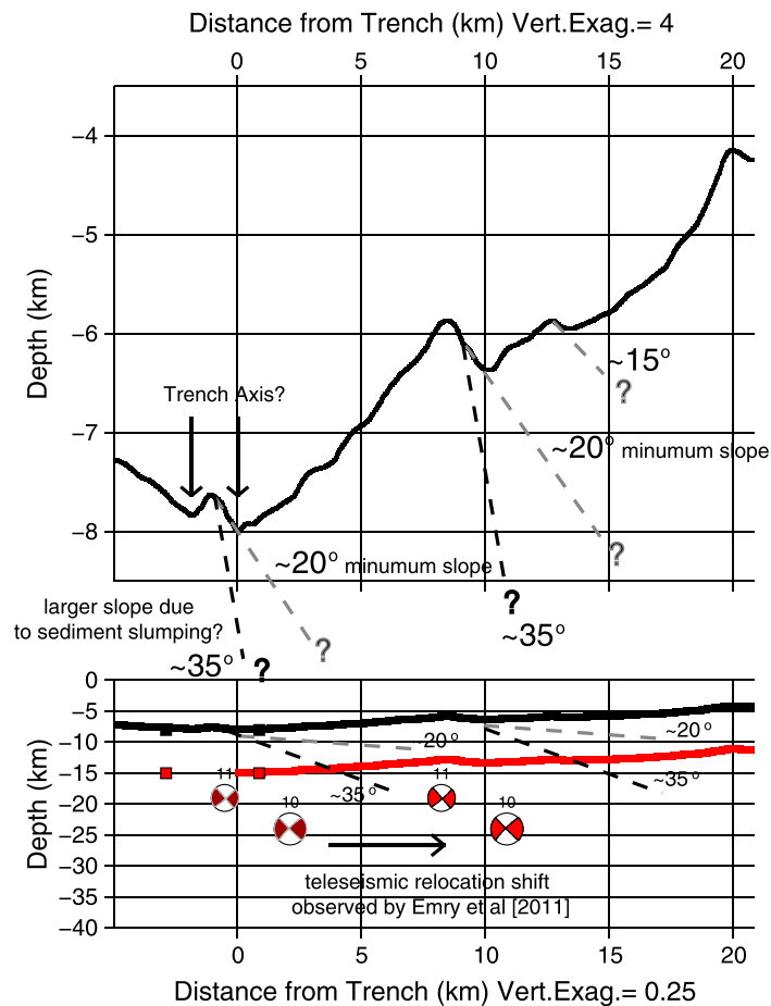
Figure 6. (top) Cross-sectional profile around the 5 April 1990 outer rise earthquake; vertical exaggeration (VE) = 4 along (15.4°N, 147.4°E) to (15.2°N, 148°E). Bathymetry is shown as thick black lines, estimated continuation of surface faults for dip measured from bathymetry (~15–20°) (gray dashed line) and for steeper-dipping faults (~35°) (black dashed line). (bottom) Same as above with vertical exaggeration (VE) = 0.25. Thick black lines indicate bathymetry; thick red line shows depth to Moho assumed by our waveform inversion technique. Black squares indicate depth to plate interface ~17°N as determined by Oakley et al. [2008]; red squares show continuation of the Moho landward from the trench. Focal mechanisms for the 5 April 1990 and 6 April 1990 earthquakes (Events 10 and 14, Table 4) are rotated 90° into cross section. Emry et al. [2011] compared local and teleseismic earthquake locations near the Mariana trench and found teleseismic locations shifted westward, so we applied a similar shift here to reduce the effects of global structure bias. Focal mechanisms at original relocation position are further west on the diagram; dilatational quadrants are indicated by white, and compressional quadrants are shown in maroon. Focal mechanisms with corrected positions are further east on diagram; dilatational quadrants are indicated by white, and compressional quadrants are indicated by red. Shallow-dipping faults are shown as dashed gray lines and steeper-dipping faults are shown as black dashed lines.
