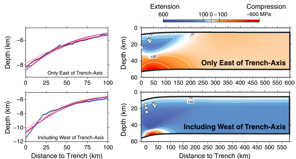
Figure 10. (top right) Stress distribution predicted by best fit flexure model for the North Central Mariana outer rise using bathymetry profile eastward of the trench axis. (bottom right) Best fit model using bathymetry eastward of trench axis and profile of the plate interface westward of the trench axis [ Oakley et al., 2008 ]. The bottom stress distribution is shifted ~20 km westward of top plot, due to inclusion of the plate profile landward of the trench. Extensional stresses correspond to blue regions and positive values (MPa); compression corresponds to red regions and negative values. Extensional earthquakes are plotted as white diamonds; strike-slip earthquakes are black crosses; compressional earthquakes are gray circles. (left column) Observed profile of the top of the plate (from bathymetry or from bathymetry and seismic reflection) is denoted by the thick blue points. The plate profiles predicted by other small misfit flexure models are plotted as shades of red and purple.
