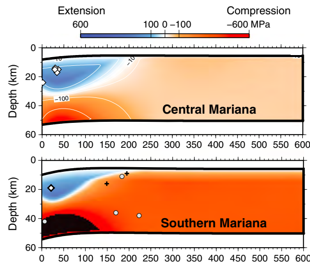
Figure 8. (top) The best fit flexure model for the Central Mariana outer rise using bathymetry seaward (east) of the trench axis. (bottom) The best fit flexure model for the Southern Mariana outer rise using bathymetry seaward (southeast) of the trench axis. Tensional deviatoric stresses correspond to blue regions and positive values (MPa); compression corresponds to red regions and negative values, and black regions indicate highly compressional stresses where the color scale has saturated. Extensional earthquakes plotted as white diamonds; strike-slip earthquakes are black crosses; compressional earthquakes are gray circles.
