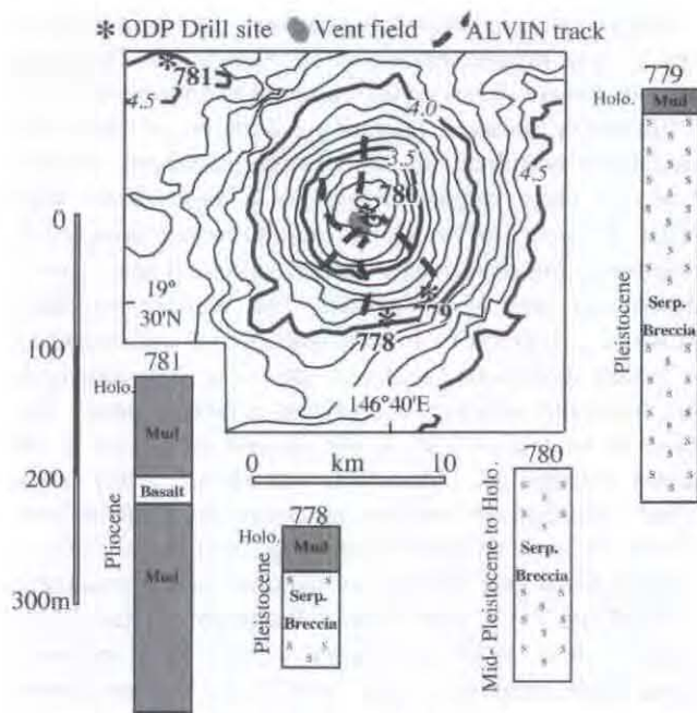
Figure 16. Conical Seamount, location shown in Figure 15. Map shows the location of active vents and chimney structures [Fryer et al. , 1995], and location of ODP drill sites and ALVIN dive tracks [Fryer et al. , 1990a]. Tracks for five dives (1851-1855) on the flanks are shown; four dives (1859-1862) on the summit are not shown. Rock sequences penetrated by ODP sites 778-781 are portrayed very schematically, along with age assignments (from ODP Leg 125 Initial Reports). Note the presence of a basalt sill at ODP site 781. Bathymetry in km.
