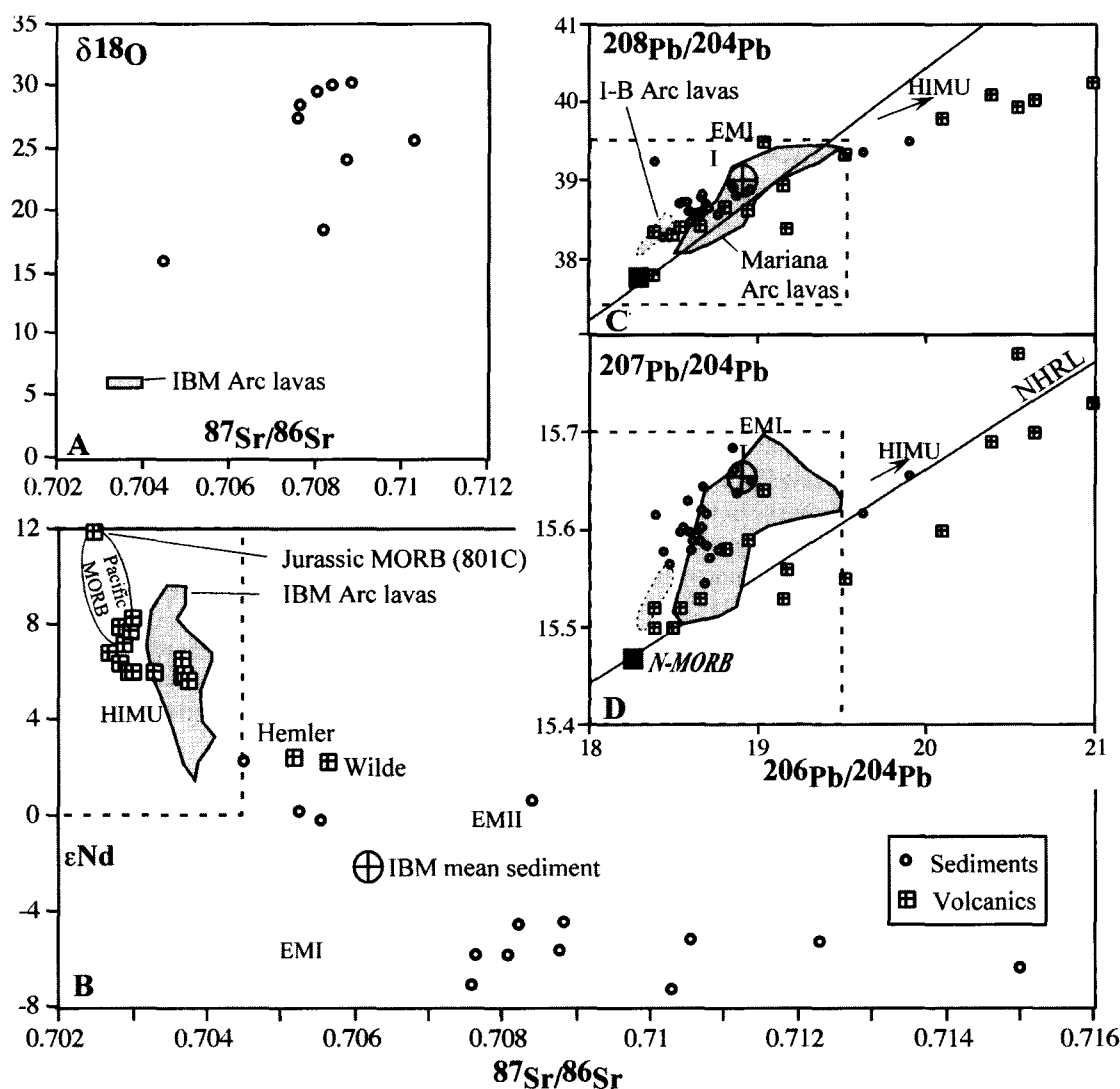
Figure 9. Isotopic composition of sediments and volcanics being fed into the IBM Subduction Factory. A) O-Sr isotopic systematics for sediments (data from Stern and Ito [1983], Woodhead and Fraser [1985], and Woodhead [1989]). B) Sr-Nd isotopic systematics for W. Pacific sediments (data from Lin [1992], Stern and Ito [1983], and Woodhead [1989]) and means calculated for Jurassic seafloor and Jurassic alkali basalt at ODP 801C [Castillo et al. , 1992]; alkalic sill at ODP 800 [Castillo et al. , 1992]; Cretaceous off-ridge tholeiites at ODP 802 [Castillo et al. , 1994], Nauru Basin (ODP 462; [Castillo et al. , 1991], and the Ontong Java Plateau [Mahoney and Spencer, 1991]; Magellan seamounts (Himu, Hemler, Golden Dragon); Wake seamounts (Wilde, Miami, Lamont, and Scripps) [Staudigel et al. , 1991]; Marshall Islands [Davis et al. , 1989]; and Caroline Islands [Hart, 1988]. Notice that data for lavas clusters about \epsilon\text{Nd} \sim +6 to +8 , ^{87}\text{Sr}/^{86}\text{Sr} \sim 0.7027 – 0.7040 except for the Jurassic MORB at 801C and Hemler and Wilde seamounts. Approximate locations of mantle reservoirs EMI, EMII, and HIMU are also shown. Sediment samples with ^{87}\text{Sr}/^{86}\text{Sr} < 0.706 contain a high proportion of volcanoclastic material. Location of weighted mean for sediment being subducted beneath IBM [Plank and Langmuir, 1998] is shown, along with fields for fresh MORB and IBM arc lavas. C) ^{208}\text{Pb}/^{204}\text{Pb} vs. ^{206}\text{Pb}/^{204}\text{Pb} for W. Pacific sediments and volcanics, data sources as above. D) ^{207}\text{Pb}/^{204}\text{Pb} vs. ^{206}\text{Pb}/^{204}\text{Pb} . Also shown is the estimated composition of IBM mean sediment from Plank and Langmuir, [1998] and the Northern Hemisphere Reference Line (NHRL) after Hart [1984]. Dashed rectangles in B–D show the areas plotted in Figure 21.
