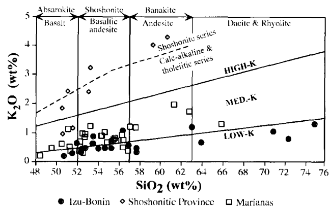
Figure 17. Potassium-silica diagram for the mean composition of 62 volcanoes along the magmatic front of the IBM arc system. Data sources discussed in text. Names for rocks indicated for calc-alkaline and tholeiitic series below the double arrows, above the double arrows for the shoshonitic series.
