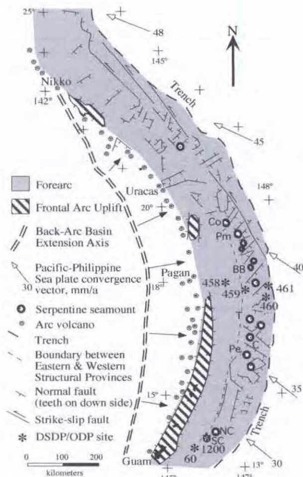
Figure 15. The IBM forearc, between 13° and 25°N, shown in gray. Generalized structural features and location of serpentine mud volcanoes are taken from Stern and Smoot [1998]. Dashed line marks the boundary between rough and smooth terrains of Stern and Smoot [1998], or between Eastern and Western Structural Provinces of Mrozowski and Hayes [1980]. Arrows radiating out from the back-arc basin extension axis show how differential extension causes decreasing radius of curvature of the arc, leading to stretching of the forearc along strike. Location of DSDP sites 60, 458, 459, 460, 461, and 1200 are shown. ODP sites 778-781 are centered on Chamorro Seamount. Names of serpentine mud volcanoes, after Fryer et al. [1999] from south to north: South Chamorro, SC; North Chamorro, NC; Blue Moon, BM; Peacock, Pe; Celestial, C; Turquoise, T; Big Blue, BB; Pacman, Pm; Conical, Co.
