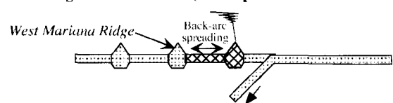
Figure 5. Simplified history of the IBM arc system. Shaded areas are magmatically inactive, cross-hatched areas are magmatically active.
