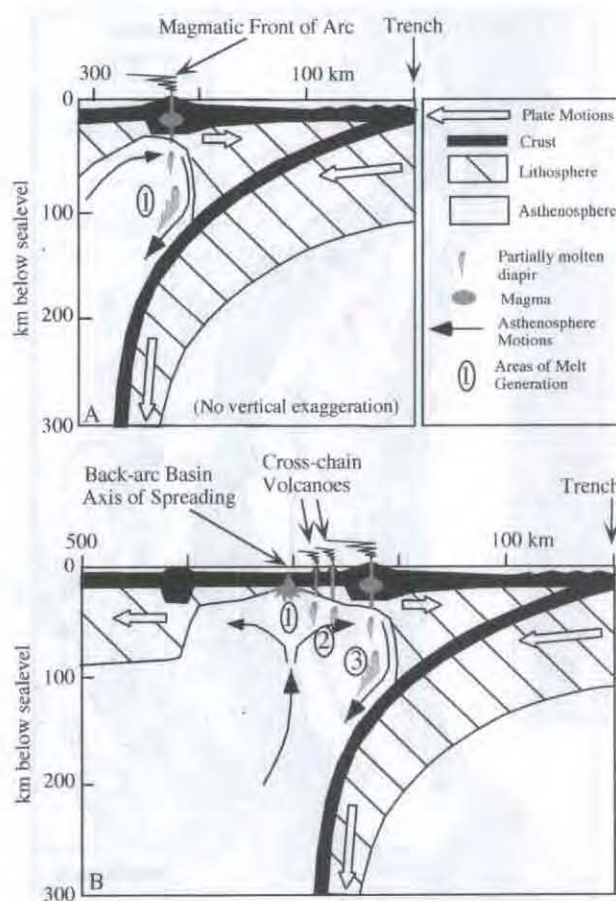
Figure 25. Conceptual models for evolution of the Subduction Factory from one lacking an actively spreading back-arc basin (A) to one associated with back-arc spreading (B). Note that magma generation and migration beneath the magmatic front occurs in a region of mantle downwelling, whereas that beneath the back-arc basin spreading axis occurs in a region of mantle upwelling. Note in (B) the multiple melting opportunities for mantle rising beneath the back-arc basin, with melt generation beneath the spreading axis (1), beneath cross-chains (2) and beneath the magmatic front (3). The IBM arc system presents all of these stages, with the Bonin segment now acting as an unrifted arc (A) whereas the Mariana segment is an outstanding example of an arc associated with back-arc spreading (B). The Izu segment represents an intermediate situation, where rifting is underway but has not proceeded to seafloor spreading.
