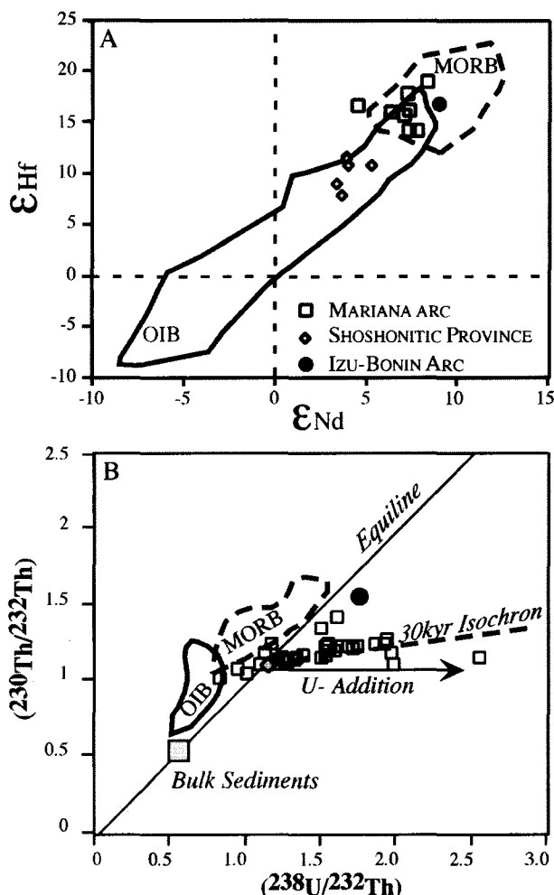
Figure 23. (A) Hf-Nd isotopic variations for the IBM arc system, data from [Pearce et al. , 1999; White and Patchett, 1984; Woodhead, 1989] (Vervoort, personal communication, 2000). Fields for OIB and MORB are from Vervoort et al. [1999] and define the mantle array. (B) U-Th disequilibrium data for IBM arc lavas. Data are not averaged for each edifice. Data from Elliott et al. [1997], Gill and Williams [1990], McDermott and Hawkesworth [1991], Newman et al. [1984], and Reagan (personal communication, 2000).
