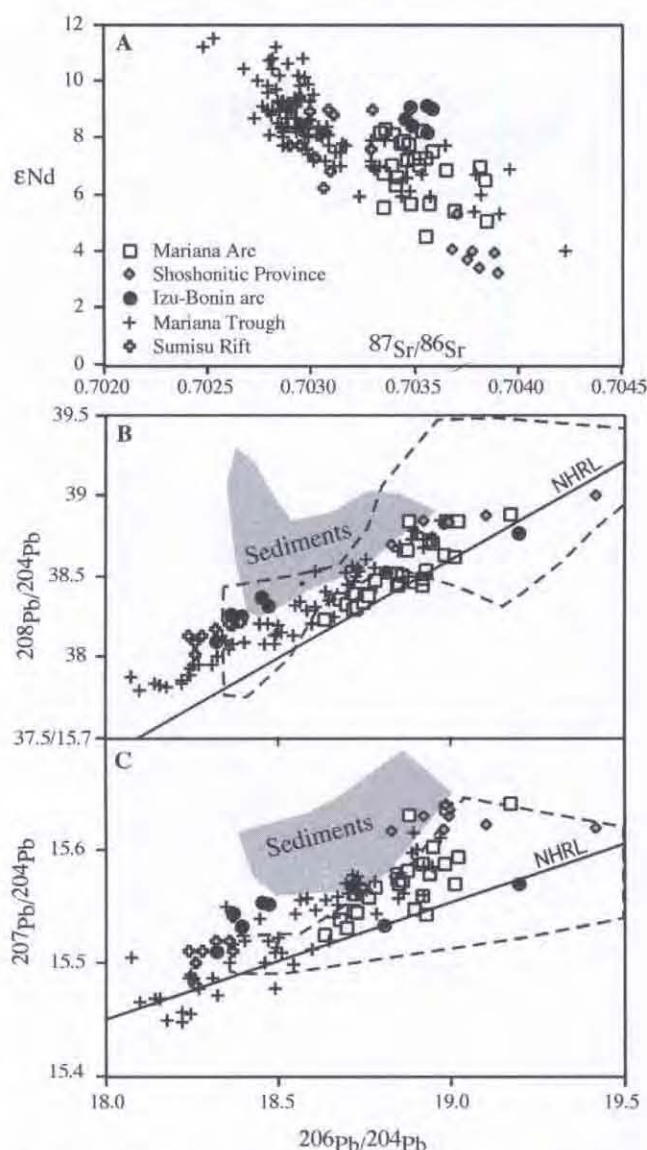
Figure 21. Isotopic composition of Sr, Nd, and Pb for IBM arc lavas, including Sumisu Rift and Mariana Trough basalts. Data for IBM arc are averages for individual volcanoes, data for Sumisu Rift and Mariana Trough are individual analyses. Fields for sediments (shaded) and W. Pacific off-ridge volcanics (dashed), taken from Figure 9, are shown in B and C. Location of these diagrams is shown with dashed boxes on Figure 9. The Northern Hemisphere Reference Line (NHRL [Hart, 1984]) is shown for comparison.
