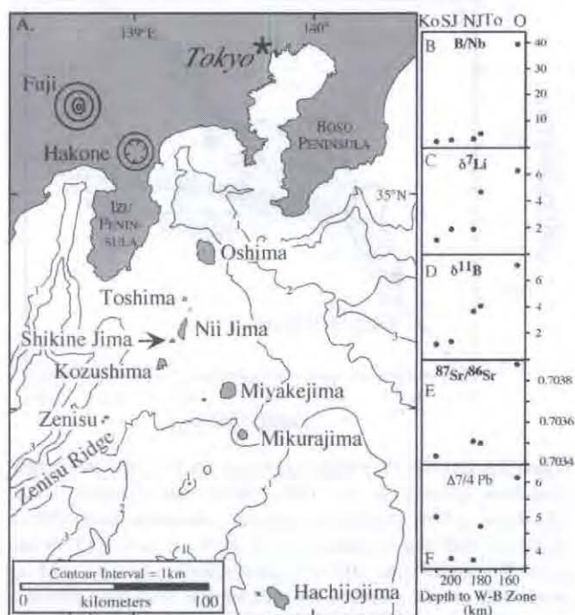
Figure 24. A) Locality map for the northern IBM arc system and the Zenisu cross-chain. B-F) plot volcano-means for parameters sensitive to fluid input (B) or contributions from the subducted slab (C-F) vs. depth to the Wadati-Benioff zone. B) Variations of B/Nb vs. depth to the Wadati-Benioff Zone. Islands Oshima (Os), Toshima (To), Nii Jima (Nj), Shikine Jima (Sj); Kozushima (Ko); C) Variations of \delta^7\text{Li} vs. depth to the Wadati-Benioff Zone; D) Variations of \delta^{11}\text{B} vs. depth to the Wadati-Benioff Zone; E) Variations of ^{87}\text{Sr}/^{86}\text{Sr} vs. depth to the Wadati-Benioff Zone; F) Variations of \Delta 7/4 \text{ Pb} vs. depth to the Wadati-Benioff Zone. Notice the decrease in all parameters sensitive to subducted inputs with greater depth to the seismic zone. Data are from Ishikawa and Nakamura, [1994], Moriguti and Nakamura [1998], and Notsu et al. [1983].
