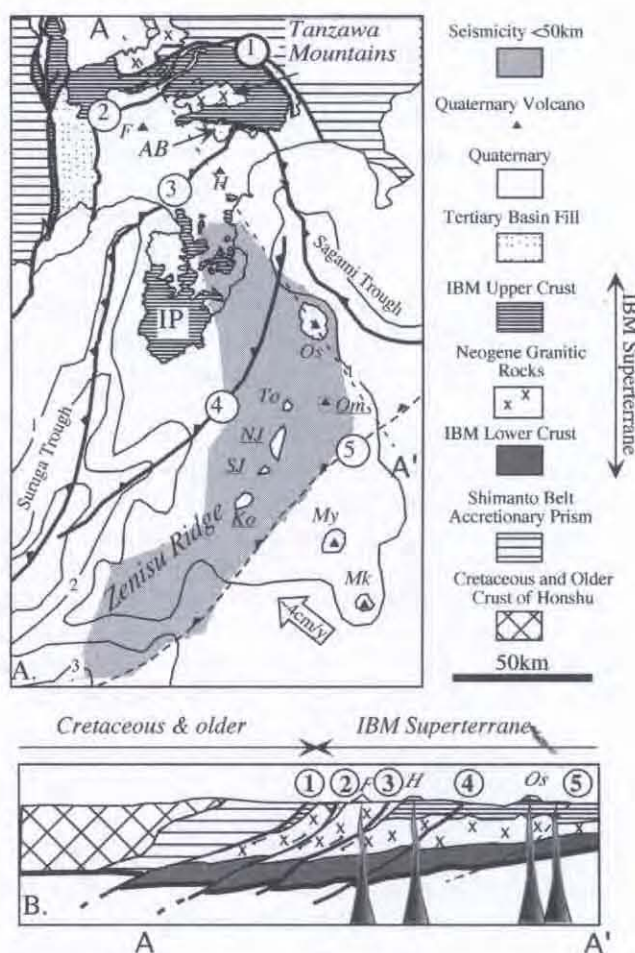
Figure 28. The IBM collision zone. A) Geologic map showing the location of major thrust faults and tectonic lines (1-5 circled) and the Tanzawa Mountains. 1= Mineoka/Tonoki-Aikawa/Itoigawa-Shizuoka Thrust; 2=Tonoki-Aikawa/Nishikatsura/Minobu Thrust; 3=Kouzu-Matsuda/Kannawa Thrust; 4=Izu-Toho Tectonic Line; 5=Zenisu-Oki Tectonic Line. Dashed line indicates incipient thrust fault. IP = Izu Peninsula; AB = Ashigara Basin. Water depth contours are labeled in km. Volcanoes are abbreviated F=Fuji, H=Hakone, Os = Oshima, Om = Omurodashi (submarine), To = Toshima, NJ = Nii Jima, SJ = Shikine Jima, Ko = Kozushima, My = Miyakejima, Mk = Mikurajima. Underlining indicates dominantly felsic volcano. Arrow labeled '4 cm/y' indicates convergence direction and rate between IBM arc and Honshu. Note the generalized location of seismicity shallower than 50\text{ km} . Dashed line A-A' shows approximate location of section shown in B. Figure modified after Kawate and Arima [1998] and Taira et al. [1998]. B) Along-arc cross-section A-A', modified after Taira et al. [1998], showing sequence of imbrications of the IBM Superterrane. No vertical exaggeration. Scales for A and B are identical.
