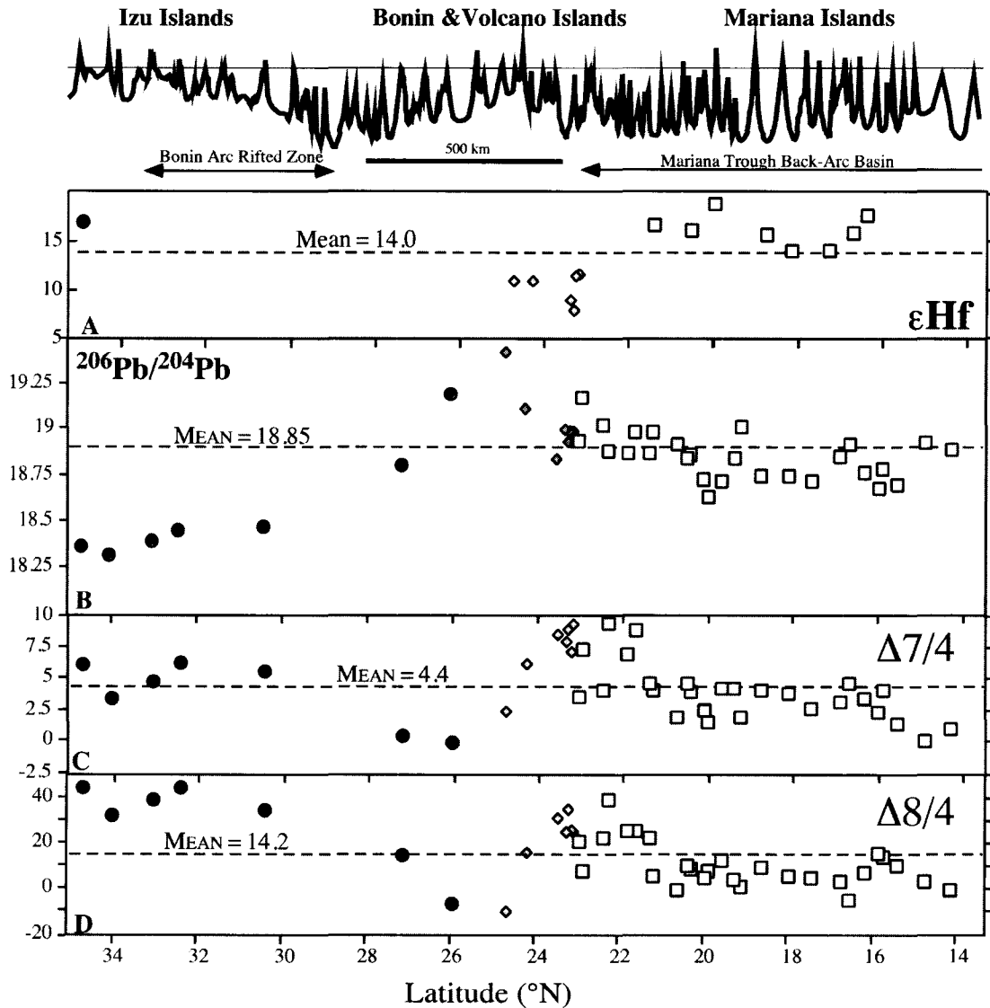
Figure 22. Isotopic variations along the magmatic front of the IBM arc. Symbols are the same as in Figure 17 (filled circles: Izu-Bonin; diamonds: Shoshonitic Province; open squares: Mariana). A) \epsilon_{\text{Hf}} ; B) ^{206}\text{Pb}/^{204}\text{Pb} isotopic variations; C) \Delta 7/4 ; and D) \Delta 8/4 . Hf isotopic data are from Pearce et al. [1999], White and Patchett [1984], Woodhead [1989], and Vervoort (personal communication, 2000). Delta notation for Pb follows Hart [1984]; Epsilon notation for Hf follows Pearce et al. [1999].
