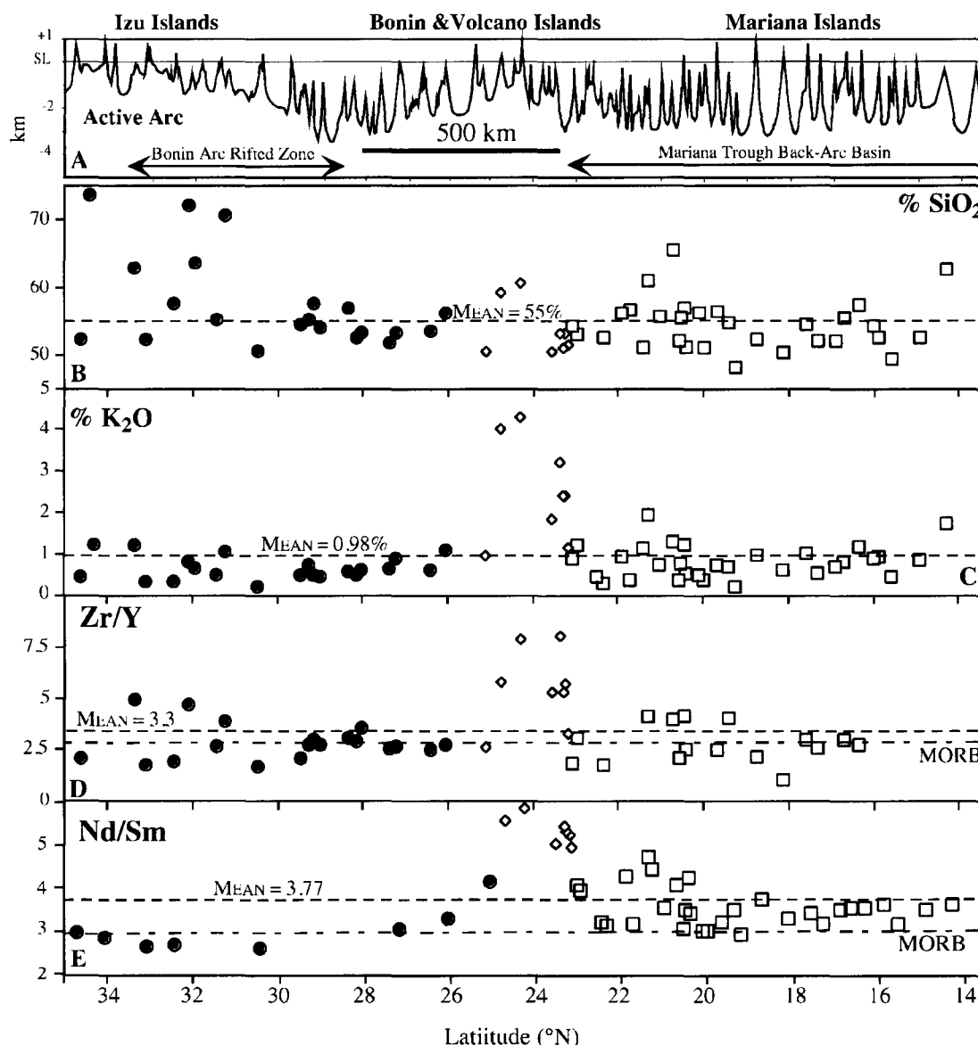
Figure 18. Profiles of mean silica and potash contents and Zr/Y and Nd/Sm for volcanoes along the magmatic front of the IBM arc. Data sources as described in text, same symbols as in Figure 17. A) Variations in bathymetry along the same profile, similar to Figure 2. Names of individual volcanoes can be found in Figure 2. Along-strike variations in silica B) and potash C) are shown, using symbols as in Figure 17. Mean silica and potash contents are shown for the IBM magmatic front as a dashed line. Along-strike variations in Zr/Y D) and Nd/Sm E) are shown, using symbols as in Figure 17. Mean values for Zr/Y and Nd/Sm are shown for the IBM magmatic front as a dashed line labeled Mean and also for typical MORB [Hofmann, 1988].
