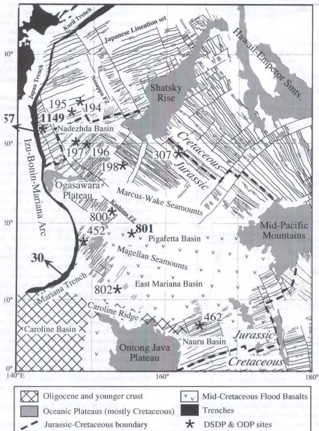
Figure 3. Simplified geologic and magnetic map of the western Pacific, modified after Nakanishi et al. [1992]. Relative motion of the Pacific Plate with respect to the Philippine Sea Plate is shown with arrows, numbers correspond to velocities (mm/year), after Seno et al. [1993].
