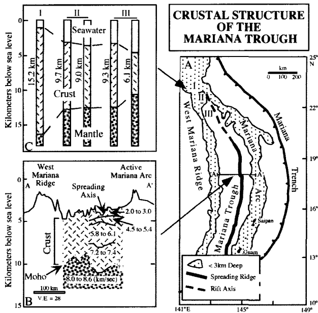
Figure 14. Crustal structure of the Mariana Trough. (A) Shows the location of B and C. (B) Crustal structure beneath the central Mariana Trough is combined from the seismic refraction results of Bibee et al. [1980] in the east, centered beneath the spreading ridge, and the results of LaTraille and Hussong [1980] in the west. Numbers correspond to P wave seismic velocities, in km/sec. The Moho is defined by velocities greater than 8 km/sec, although the 7.4 km/sec velocity in the east may be anomalously slow mantle, perhaps due to the presence of partial melt. (C) Crustal structure beneath the northern Mariana Trough is based on interpretation of gravity data [ Ishihara and Yamazaki , 1991]. Note the rapid thinning southward to crustal thicknesses corresponding to normal oceanic crust just south of 22°N.
