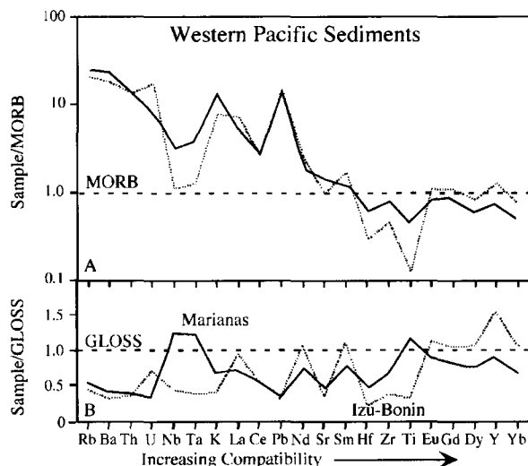
Figure 8. Chemical composition of sediments being fed into the IBM Subduction Factory. Composites for sediments outboard of Izu-Bonin (dotted line) and Mariana (solid line) are after Plank and Langmuir [1998], (A) normalized to abundances in MORB [Hofmann, 1988] and (B) normalized to Global Subducting Sediments (GLOSS; [Plank and Langmuir, 1998]).
