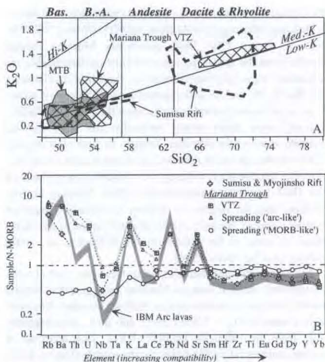
Figure 27. Chemical features of IBM rift-related lavas. A) Potash-silica diagram for IBM rift-related igneous rocks. Fields are shown for Sumisu and Myojinsho rifts (66 samples), Mariana Trough VTZ (41 samples), and Mariana Trough spreading segment (labeled MTB, 167 samples). Note the bimodal nature of lavas erupted in rifts and strictly mafic nature of lavas erupted in the region undergoing spreading. B) Incompatibility plot for extension-related IBM lavas. Sumisu rift data is mean from data set of Hochstaedter et al., 1990b; note that this pattern is incomplete. Mariana Trough data are for glasses analyzed by Pearce (unpublished ICP-MS data). VTZ sample is T7-54:1-1 (1.69% H 2 O). Two representative samples are given for the Mariana Trough spreading segment: 'arc-like' sample GTVA75:1-1 (2.21% H 2 O) and 'MORB-like' sample DS84:2-1 (0.21% H 2 O) [Gribble et al., 1996]. Composition of N-MORB and element order is after Hofmann [1988]. Grey field outlines the composition of Mariana and Izu segment lavas, from Figure 19.
