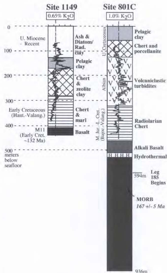
Figure 7. ODP sites 801C and 1149, locations shown on Figure 3. 801C is thought to be representative of sediments being subducted beneath the Marianas and 1149 of those going down beneath Izu-Bonin. Superimposed on simplified lithological columns are K contents determined using the natural gamma down hole logging tool. Note that enrichments in K and other incompatible elements in sediments being subducted beneath the Mariana arc is largely due to the thick sequence of Albian (Cretaceous) volcanoclastics http://www-odp.tamu.edu/publications/185_IR/VOLUME/CHAPTERS/IR185_04.PDF
