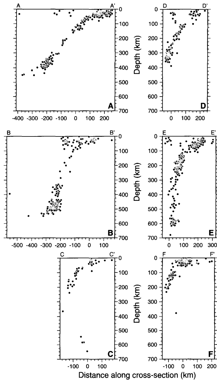
Figure 11. Cross-sectional views of the IBM system using the earthquake catalog of Engdahl et al. [1998]. Black circles represent hypocentral locations in volume \sim 60 km to each side of the lines shown in Figure 10. Large variations in slab dip and maximum depth of seismicity are apparent. Distance along each section is measured from the magmatic arc. A) Northern Izu-Bonin region. Slab dip is \sim 45^\circ ; seismicity tapers off from \sim 175 km to \sim 300 km but increases around 400 km, and terminates at \sim 475 km. B) Central Izu-Bonin region. Slab dip is nearly vertical; seismicity tapers off from \sim 100 km to \sim 325 km but increases in rate and extends horizontally around 500 km, and terminates at \sim 550 km. C) Southern Izu-Bonin region. Slab dip is \sim 50^\circ ; seismicity is continuous to \sim 200 km, but a very few anomalous events are evident down to \sim 600 km. D) Northern Mariana region. Slab dip is \sim 60^\circ ; seismicity is continuous to \sim 375 km and terminates at \sim 400 km, but a very few anomalous events are evident down to \sim 600 km. E) Central Mariana region. Slab dip is vertical; seismicity tapers off slightly between \sim 275 km and \sim 575 km, but is essentially continuous. A pocket of deep events around 600 km exists, as well as 1 deep event at 680 km. F) Southern Mariana region. Slab dip is \sim 55^\circ ; seismicity is continuous to \sim 225 km, with an anomalous event at 375 km.
