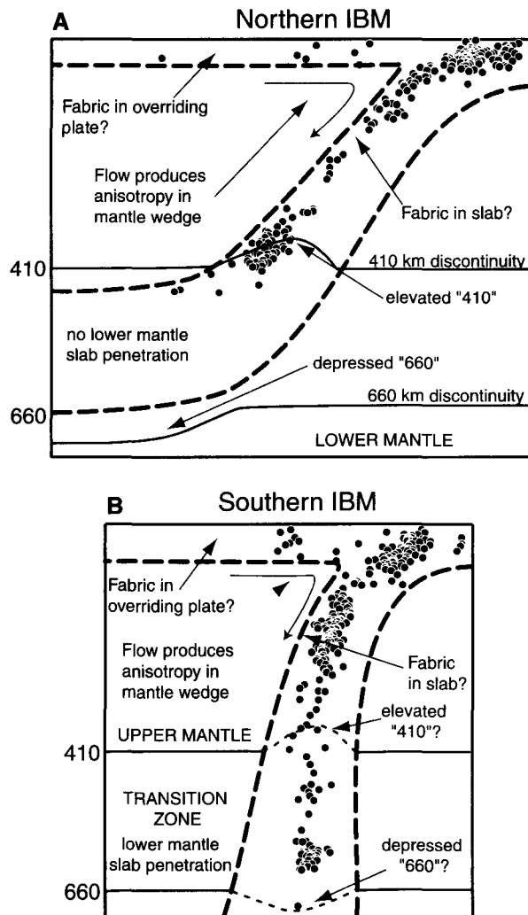
Figure 12. Cartoon representation of seismic observations in the IBM system. Black circles show representative seismicity for each region. Thick dashed lines show rough interpretation of tomographic images for each area. A) Northern IBM (near section A in Figure 11). Slab dip is variable, but averages around 50°. Tomographic images suggest that the slab does not penetrate the lower mantle, but extends horizontally to the west. The 410 km seismic discontinuity (thin line at 410) appears to be locally elevated; the 660 km seismic discontinuity (thin line at 660) appears to be depressed for an extended distance to the west. Seismic anisotropy indicates the presence of fabric in the mantle wedge, as well as possibly in the overriding plate and subducting slab. B) Southern IBM (near section E in Figure 11). Slab dip is slightly variable, but generally becomes vertical. Tomographic images suggest that the slab penetrates the lower mantle. Regional variations of upper mantle discontinuities have not yet been documented, but a locally elevated “410” and a locally depressed “660” (thin dashed lines) might be expected. Seismic anisotropy indicates the presence of fabric in the mantle wedge and subducting slab, as well as possibly in the overriding plate.
