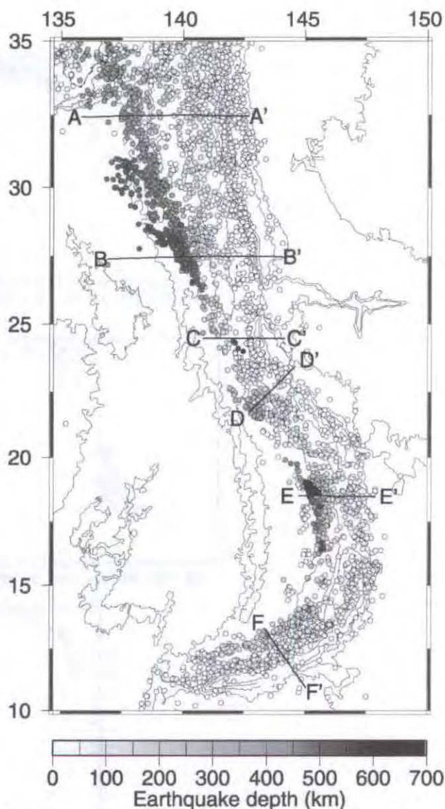
Figure 10. Map view of bathymetry and seismicity in the Izu-Bonin-Mariana Subduction Factory using the earthquake catalog of Engdahl et al. [1998]. Circles denote epicentral locations; lighter circles represent shallower events, darker circles represent deeper events. Black lines denote cross-sectional areas depicted in Figure 11. Large variations in the seismic structure of the region are evident.
