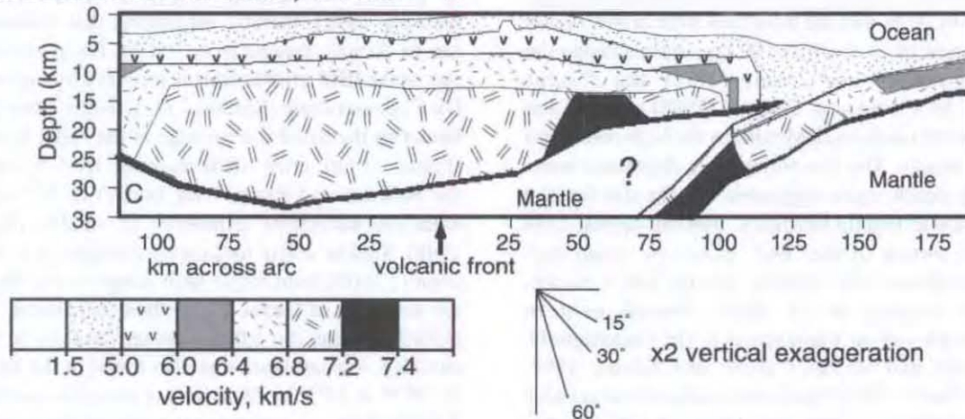
Figure 13. Arc-perpendicular cross-sections aligned along the volcanic front, redrawn to a uniform vertical exaggeration (x2) and scale, and with uniform velocity shading. "6.2" and "7.3" identify the 6.2 \pm 0.2 km/s middle crustal layer and 7.3 \pm 0.1 km/s deepest crustal layer of the IBM arc. Neither layer is prominent in the other two models. Redrawn after A: [Suyehiro et al., 1996]; B: [Lange, 1992]; C: [Holbrook et al., 1999].
