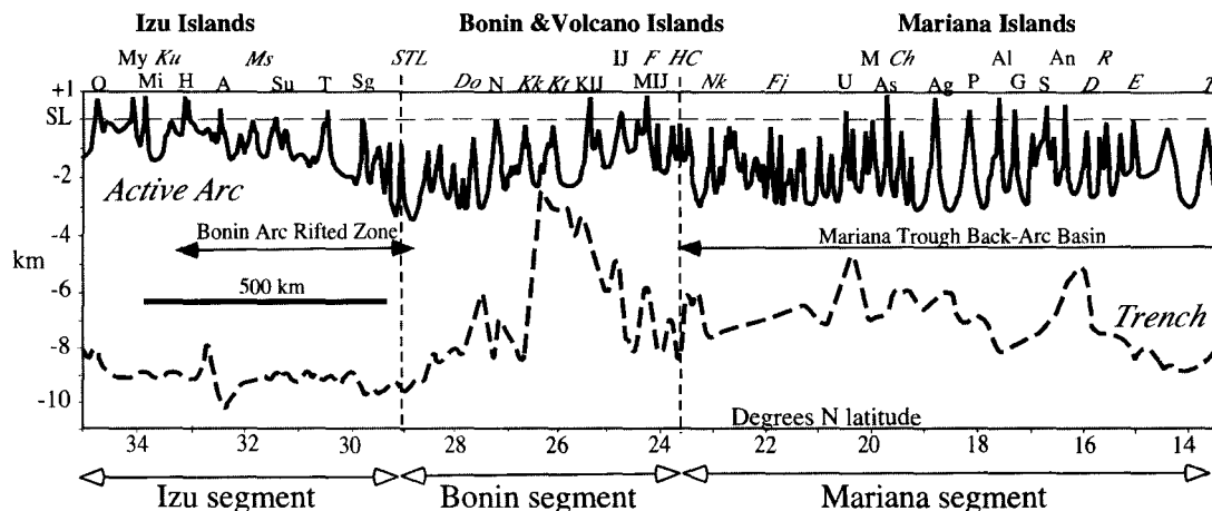
Figure 2. Along-strike profiles of the IBM Arc System, from Japan (left) to Guam (right). The thick solid line shows the bathymetry and topography along the volcanic axis of the active arc, with the thin dashed horizontal line marking sealevel. The approximate locations of the principal island groups (Izu, Bonin-Volcano, and Mariana) are shown. Submarine volcanoes (and the Sofugan Tectonic Line, STL) are given as italicized abbreviations: Ku, Kurose; Ms, Myojin-sho; Do, Doyo; Kk, Kaikata; Kt, Kaitoku; F, Fukutoku-oka-no-ba; HC, Hiyoshi Volcanic Complex; Nk, Nikko; Fj, Fukujin; Ch, Chamorro; D, Diamante; R, Ruby; E, Esmeralda; T, Tracy. Subaerial volcanoes are given as normal abbreviations: O, Oshima; My, Miyakejima; Mi, Mikurajima; H, Hachijojima; A, Aogashima; Su, Sumisujima; T, Torishima; Sg, Sofugan; N, Nishinoshima; KIJ, Kita Iwo Jima; IJ, Iwo Jima; MIJ, Minami Iwo Jima; U, Uracas; M, Maug; As, Asuncion; Ag, Agrigan; P, Pagan; Al, Alamagan; G, Guguan; S, Sarigan; An, Anatahan. Locations of important zones of intraarc and back-arc extension in the north (Bonin Arc Rifted Zone) and south (Mariana Trough Back-Arc Basin) are marked. The thick dashed line shows the maximum depth in the trench along its strike. Frontal arc elements are not shown, but consist of the Bonin or Ogasawara Islands between 26° and 28°N and the Mariana frontal arc islands between 13° and 16°N.
