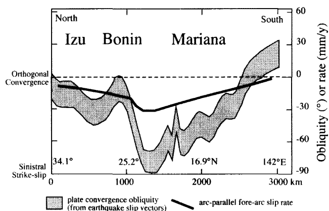
Figure 6. Convergence obliquity and fore-arc extension along the IBM arc, modified after McCaffrey [1996]. Arc segments Izu, Bonin, and Mariana are shown. Note that the northernmost Mariana arc is characterized by nearly strike-slip motion, whereas much of the Izu-Bonin and southern Mariana Arc is characterized by plate convergence that is almost orthogonal.
