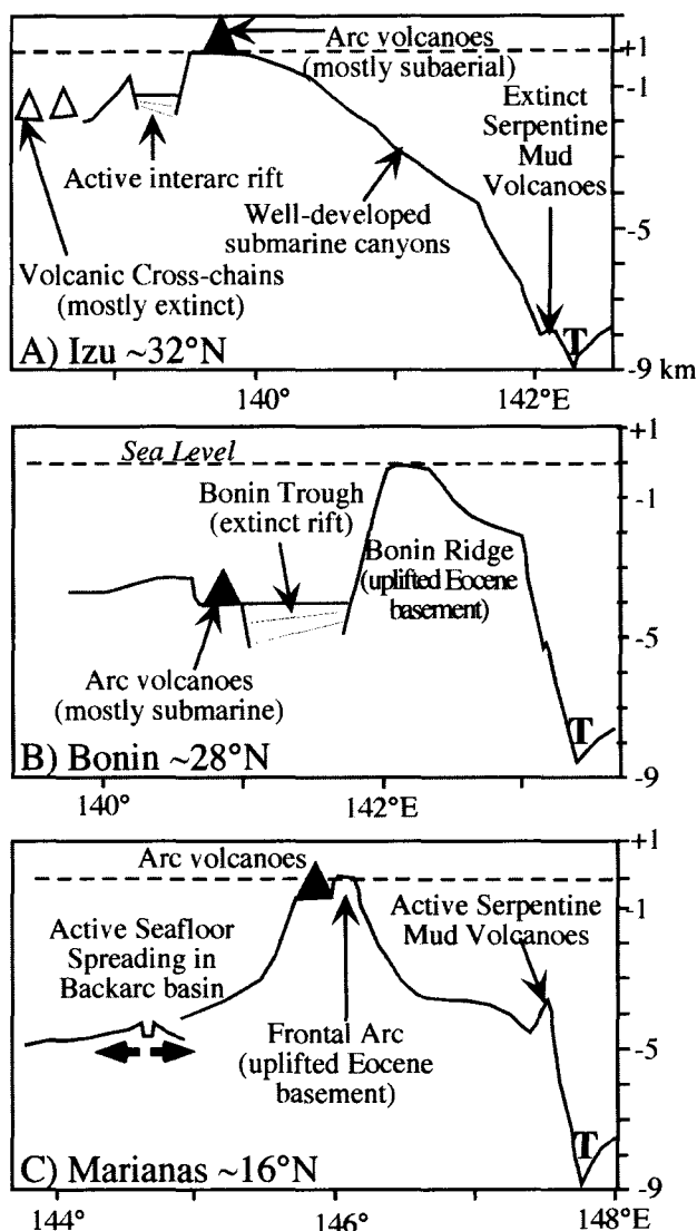
Figure 4. Greatly simplified cross sections along the IBM arc system, showing variations in morphology and tectonic style from north (Izu) through central (Bonin) and southern (Mariana) segments. Locations are shown in Figure 1. Sections taken from various reports, especially Honza and Tamaki [1985], Hussong and Uyeda [1982], Karig [1971b], and Taylor [1992]. T = trench, solid triangle = magmatic arc. Vertical exaggeration ~ 25x.
