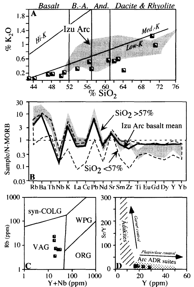
Figure 29. Geochemical characteristics of Tanzawa plutonic complex, all data from Kawate and Arima [1998]. A) K-Si diagram. Field occupied by volcano means from the Izu Arc (Figure 17) is shown in gray. Italicized volcanic rock names across the top (B.A. = basaltic andesite; And. = andesite) are intended as compositional guide. B) Incompatibility plot, composition of N-MORB and element order is after Hofmann [1988]. Field defined by mafic rocks (<57% SiO 2 ) is outlined with dashed line and that for felsic rocks (>57% SiO 2 ) is shaded. Izu Arc Basalt Mean is from Figure 19, note absence of data for U, Ta, and Hf. C) Tectonic discriminant diagram after Pearce et al. [1984]. Syn-COLG = syn-collisional granitoid; WPG = within-plate granitoid; ORG = ocean-ridge granitoid; VAG = volcanic arc granitoid. D) Petrogenetic diagram for adakites vs. arc andesite-dacite-rhyolite (ADR) suites, showing the composition of felsic rocks generated in equilibrium with garnet vs. those generated in equilibrium with plagioclase. Figure modified after Drummond and Defant [1990].
