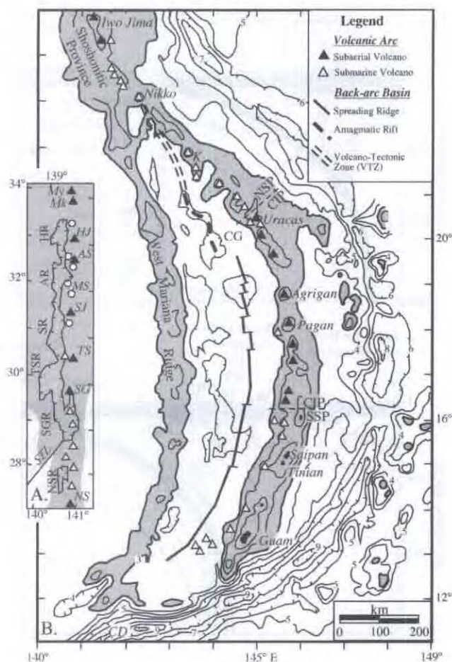
Figure 26. Actively extending systems of the IBM arc. A) Tectonic sketch map of Izu rifts, modified after Taylor [1992]; shaded where shallower than 3 km. Note this is rotated clockwise about 10° from true north. Calderas shown with open circles. Abbreviations for frontal arc volcanoes (from the north): My, Miyake Jima; Mk, Mikura Jima; HJ, Hachijo Jima; AS, Aoga Shima; MS, Myojin Sho; TS, Tori Shima; SJ, Sofu Gan; NS, Nishino Shima. STL = Sofugan Tectonic Line. Abbreviations for rifts (from the north): HR, Hachijo Rift; AR, Aogashima Rift; SR, Sumisu Rift; TSR, Torishima Rift; SGR, Sofugan Rift; NSR, Nishinoshima Rift. B) Tectonic sketch map of the Mariana Arc and back-arc basin. Bathymetric contours are in km, region shallower than 3 km is shaded. CD= Challenger Deep, SSP = Southern Seamount Province, CIP=Central Island Province, NSP=Northern Seamount Province, K=location of Kasuga cross-chain, CG=Central Graben. Note that seafloor spreading characterizes the Mariana Trough south of 19°45'N and rifting is characteristic from this latitude north to Nikko, where the extension axis intersects the arc.
