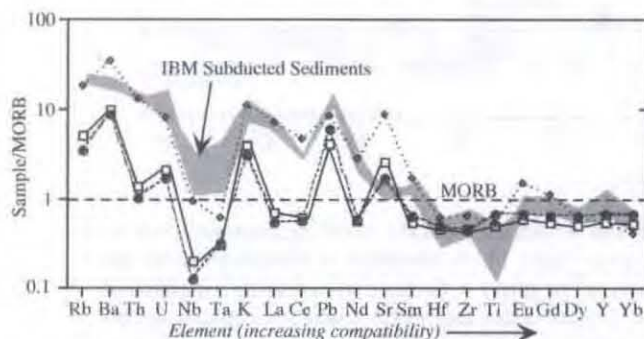
Figure 19. Incompatibility plot for lavas from along the front of the IBM arc. Typical compositions for the Mariana arc (GUG-9 of Elliott et al. [1997]; 51% \text{SiO}_2 ) and Shoshonitic province (54H of Peate and Pearce [1998]; 47.8% \text{SiO}_2 ) are plotted, along with a mean calculated for Izu arc mafic lavas (51.6% \text{SiO}_2 [Taylor and Neshitt, 1998]). Symbols are the same as in Figure 17 (filled circles: Izu-Bonin; diamonds: Shoshonitic Province; open squares: Mariana). Composition of MORB and element order is after N-MORB of Hofmann [1988]. Grey field outlines the composition of IBM subducted sediment, from Figure 8.
