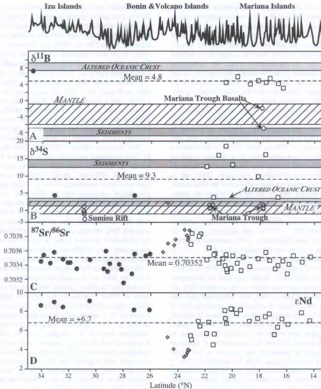
Figure 20. Isotopic variations along the IBM arc. Symbols are the same as in Figure 17 (filled circles: Izu-Bonin; diamonds: Shoshonitic Province; open squares: Mariana). (A) B isotopic variations; data for IBM arc after Ishikawa and Nakamura [1994] and Ishikawa and Tera [1999]; data for Mariana Trough basalts after Chaussidon and Jambon [1994]. Isotopic composition of altered oceanic crust, sediment, and mantle are from Ishikawa and Tera [1999]. (B) S isotopic composition of IBM arc lavas, Mariana Trough, and Sumisu rift lavas. Data for IBM arc lavas from Alt et al. [1993], Ueda and Sakai [1984], and Woodhead et al. [1987]; Data for ten Mariana Trough basalts are from Alt et al. [1993]; for 7 Sumisu Rift lavas from Hochstaedter et al. [1990a]. Fields for sediments, altered oceanic crust, and mantle are from Alt et al. [1993]. (C) Sr isotopic data for IBM arc lavas, normalized to E&A \text{SrCO}_3 ; data sources described in text. (D) Nd isotopic data for IBM arc lavas, adjusted to a common value for the La Jolla Nd standard; data sources described in text.
