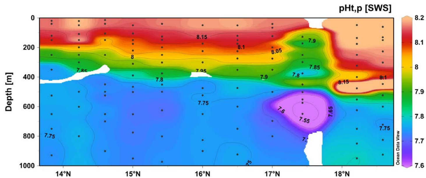
Figure 4 tm : pH along the N-S transect. Black points indicate samples
