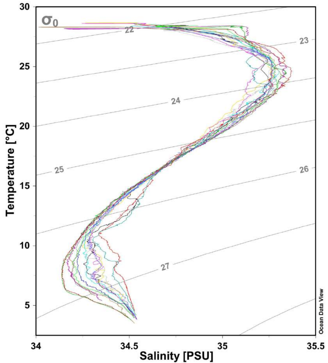
Figure 12 um : Temperature-Salinity diagram for all stations sampled. The color of the station corresponds to the color of the T-S line, and the grey contours represent potential density ( \sigma_0 ).
