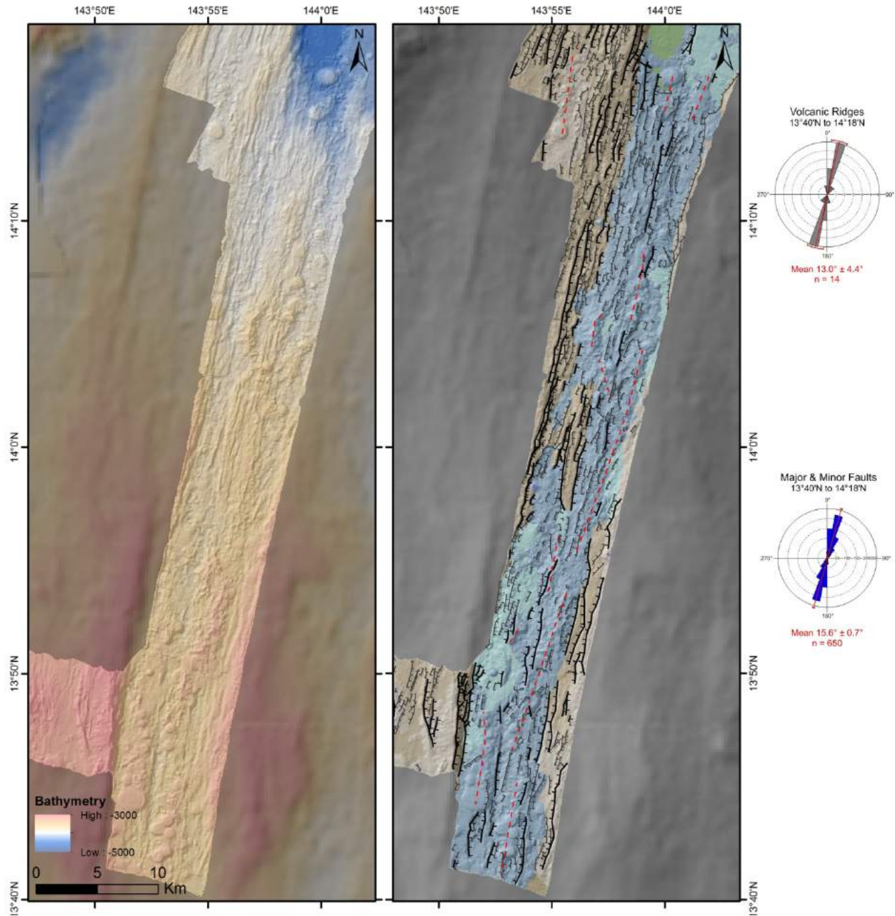
Figure 4 ge02 – Bathymetry (left) and predicted geological map (right) of the segment centered at 13.9°N (Segment 3), with rose diagrams of the volcanic ridge axes and major and minor faults of the entire segment, from 13°40'N to 14°18'N.
