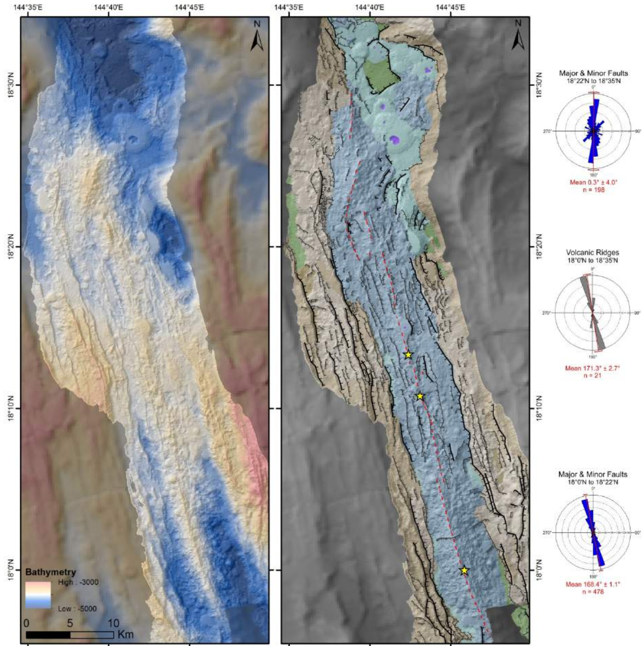
Figure 11 ge02 – Bathymetry (left) and predicted geological map (right) of the segment centered at 18.2°N (Segment 10), with rose diagrams of the volcanic ridge axes and major and minor faults of the entire segment, from 18°0'N to 18°35'N. Approximate locations of hydrothermal venting indicated by yellow stars.
