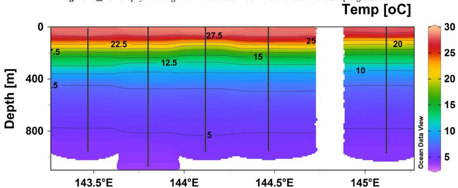
Figure 11 tm : Temperature along the E-W transect. Black lines indicate where sampling occurred.
