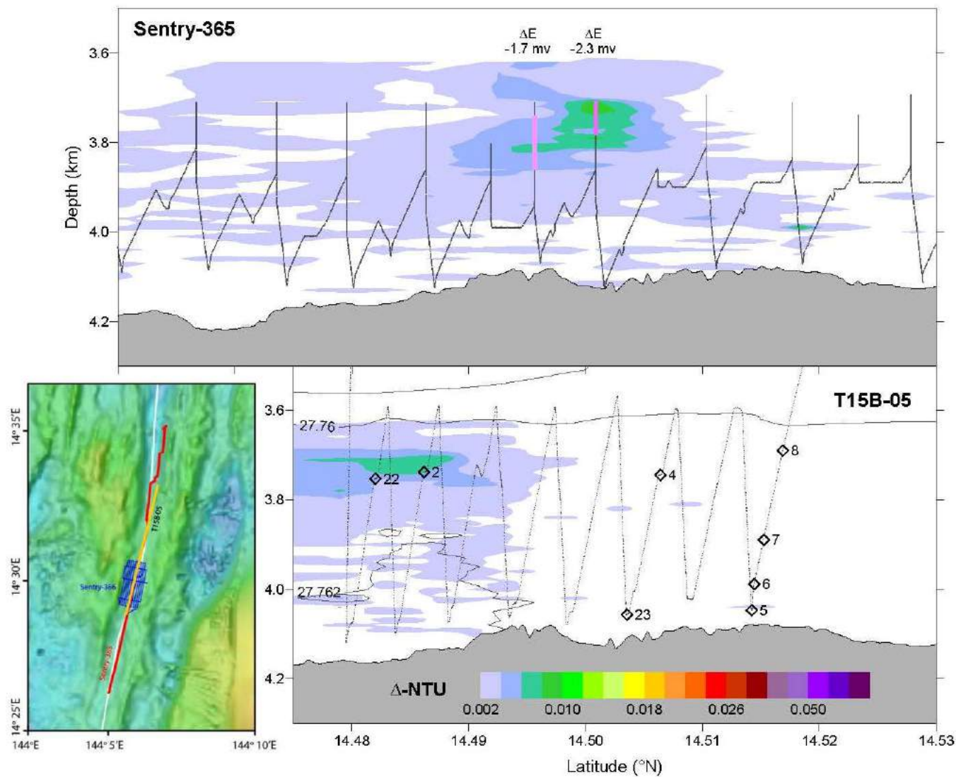
Figure 2 CTD : Color contours map the particle plume ( \Delta NTU) distribution above the Mariana back-arc segment centered at 14.5 ^{\circ} N (Map 4): AUV dive Sentry-365 (top panel) and CTD tow T15B-05 (bottom panel). Black dots show tow tracklines; open diamonds are bottle sample locations with labels indicating Niskin bottle number. Pink dots along Sentry-365 trackline indicate duration and magnitude of ORP anomalies ( dE/dt < 0 ; color indicates \Delta E for each signal and is labeled above each anomaly). No ORP data are shown for T15B-05 because no anomalies were detected during the tow. Inset: map of tracklines for Sentry-365 (red), T15B-05 (yellow), and the Sentry mapping mission ( Sentry-366 ; blue).
