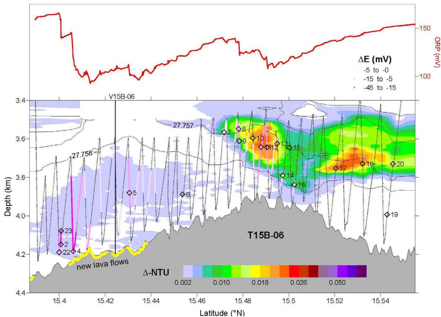
Figure 3 CTD : Color contours map the particle plume ( \Delta NTU ) distribution above the Mariana back-arc segment centered at 15.5°N (Map 5): CTD tow T15B-06. Black dots show tow trackline; open diamonds are bottle sample locations with labels indicating Niskin bottle number. Red line above color contours is ORP voltage; pink dots along trackline indicate duration and magnitude of ORP anomalies ( dE/dt < 0 ; color indicates \Delta E for each signal). Yellow line along bathymetry shows extent of new lava flow along the tow trackline. Location of vertical cast V15B-06 is shown with a black line.
