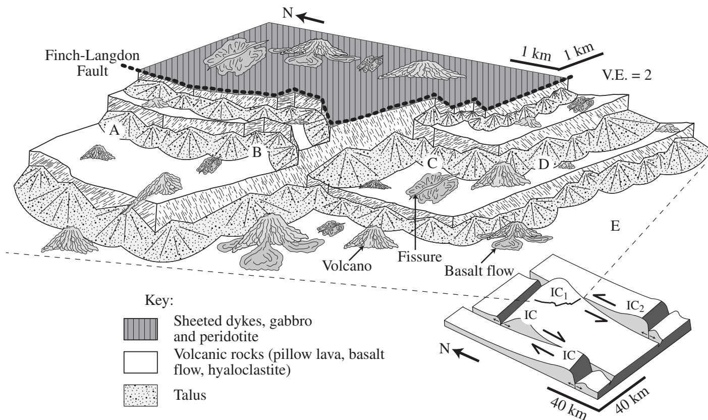
Figure 8. Model (ca. 10 Ma, V.E. = 2) of the Finch-Langdon fault (dashed line) and surrounding crust interpreted as an inside corner (IC) structure (inset after Tucholke and Lin, 1994). Shaded crust NE of the fault comprises sheeted dikes, gabbro, and peridotite. White benches, of lower relief, comprise volcanic rocks (pillow lava, basalt flow, hyaloclastite). Fault scarps show striated surfaces. Sediment wedges comprise sediment produced by the physical disintegration and tectonic abrasion of oceanic crust in submarine fault zones. Younger volcanic edifices and basalt flows that cap some sedimentary rocks are represented by volcanoes, associated flows, and massive basalt flows erupted from fissures. Volcanic activity interpreted to be related to a spreading-center located a few kilometers to the north (see inset, location IC 1 ) or to the south (see inset, location IC 2 ). Location “A” represents our interpretation of the setting of deposition of samples taken from Unity Point; “B” represents Douglas Point; “C” represents Bauer Bay; and “D” represents Mawson Point and Cormorant Point; “E” represents the small pockets of limestone or chert isolated from tectonic sedimentation (see Fig. 2 for location, and Figs. 3, 4, 5, and 6 for lithologic and stratigraphic descriptions).
